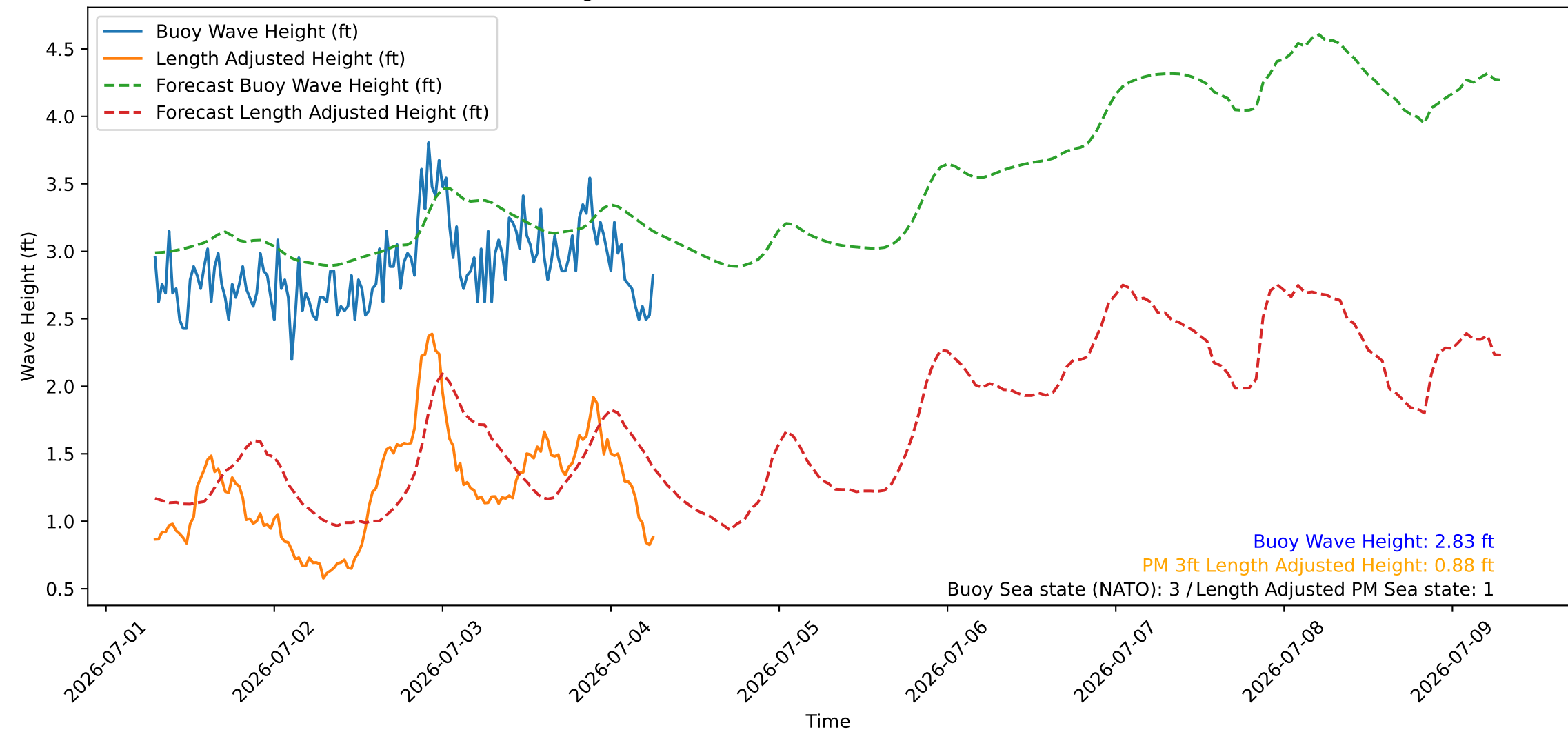
Wave Heights over Time for Red Beach at 2026-07-04 06:50:48
