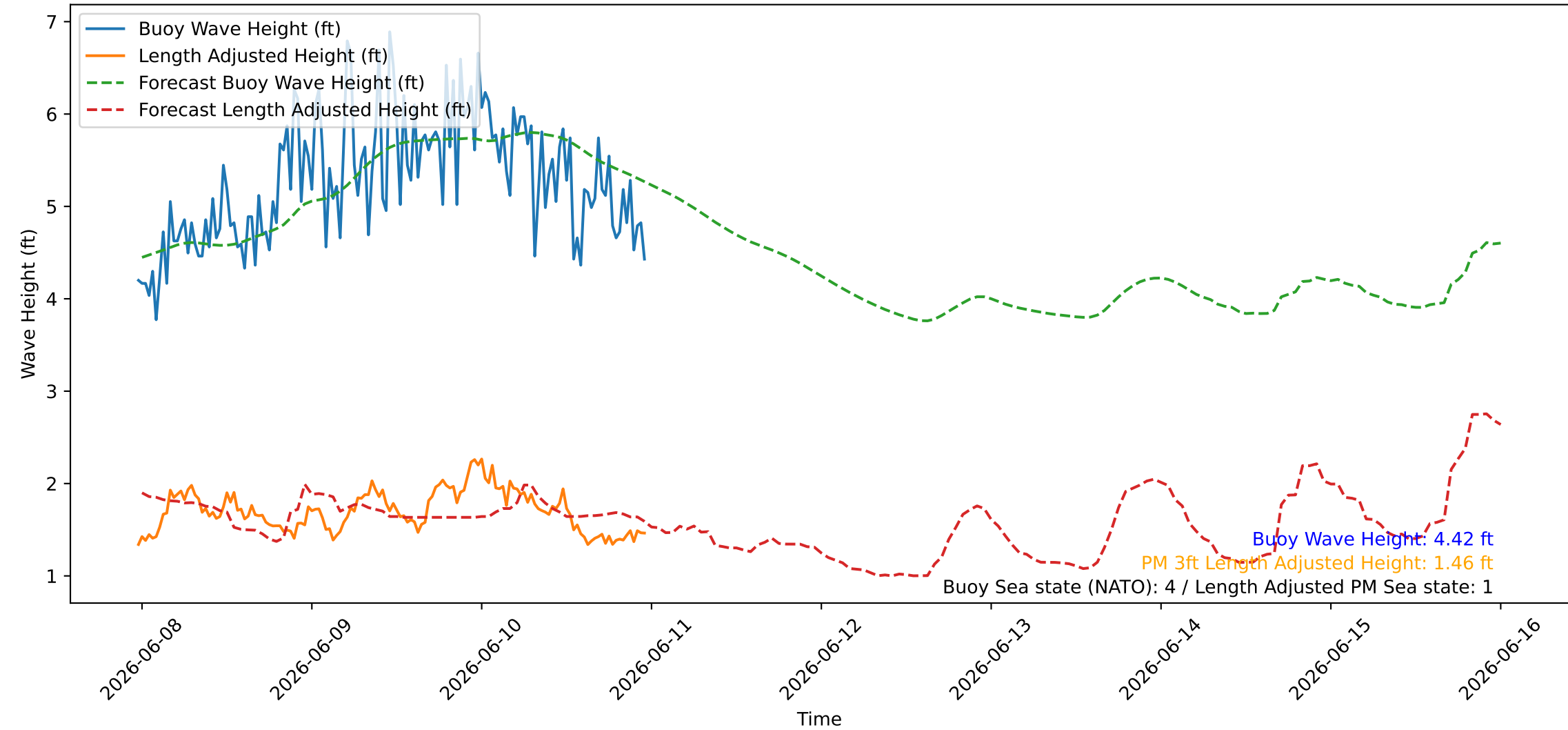
Wave Heights over Time for Green Beach at 2026-06-10 23:41:10
