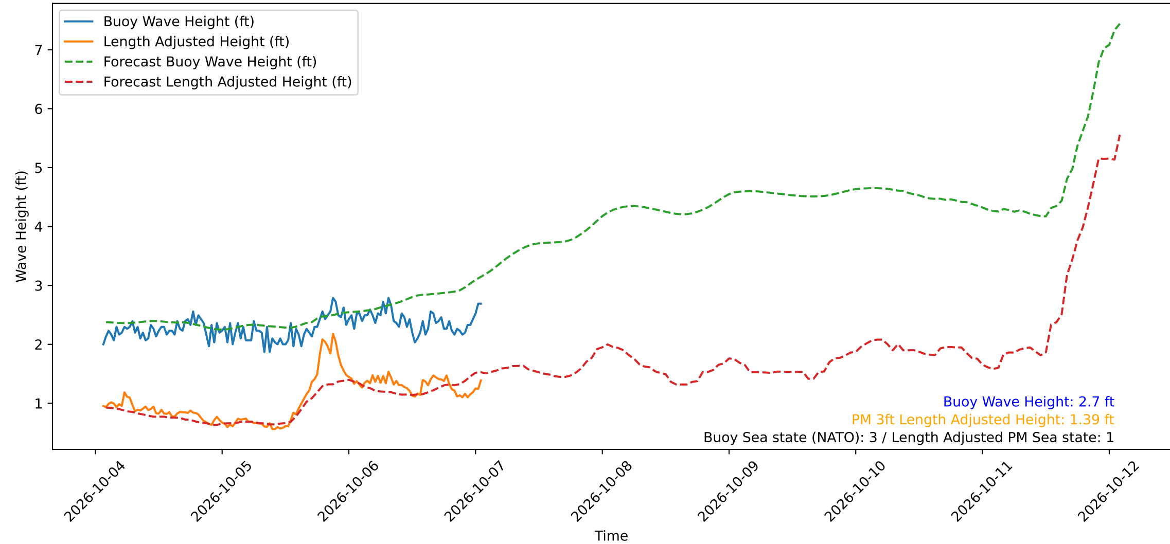
Wave Heights over Time for Oceanside Harbor at 2026-10-07 01:40:29
