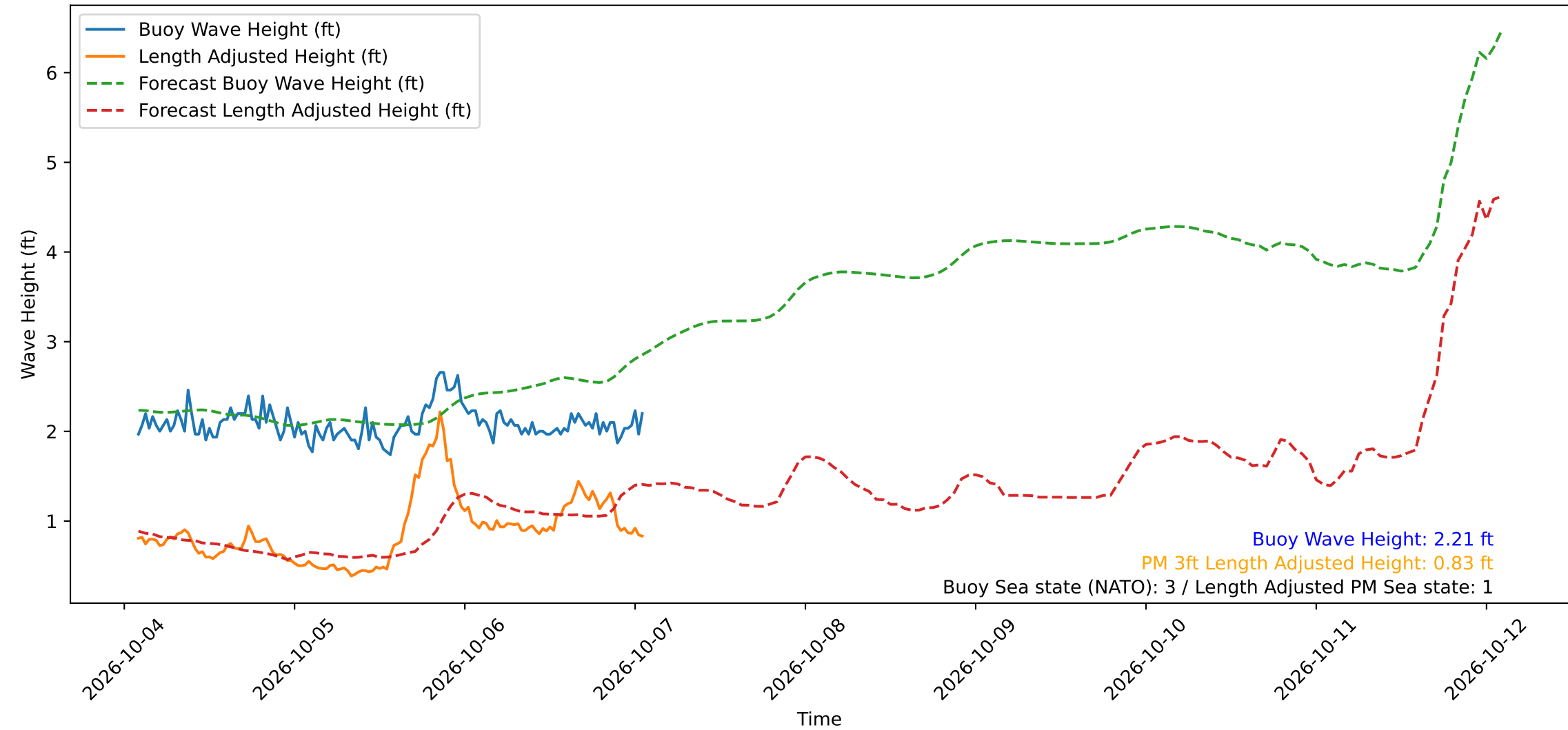
Wave Heights over Time for Red Beach at 2026-10-07 01:40:49
