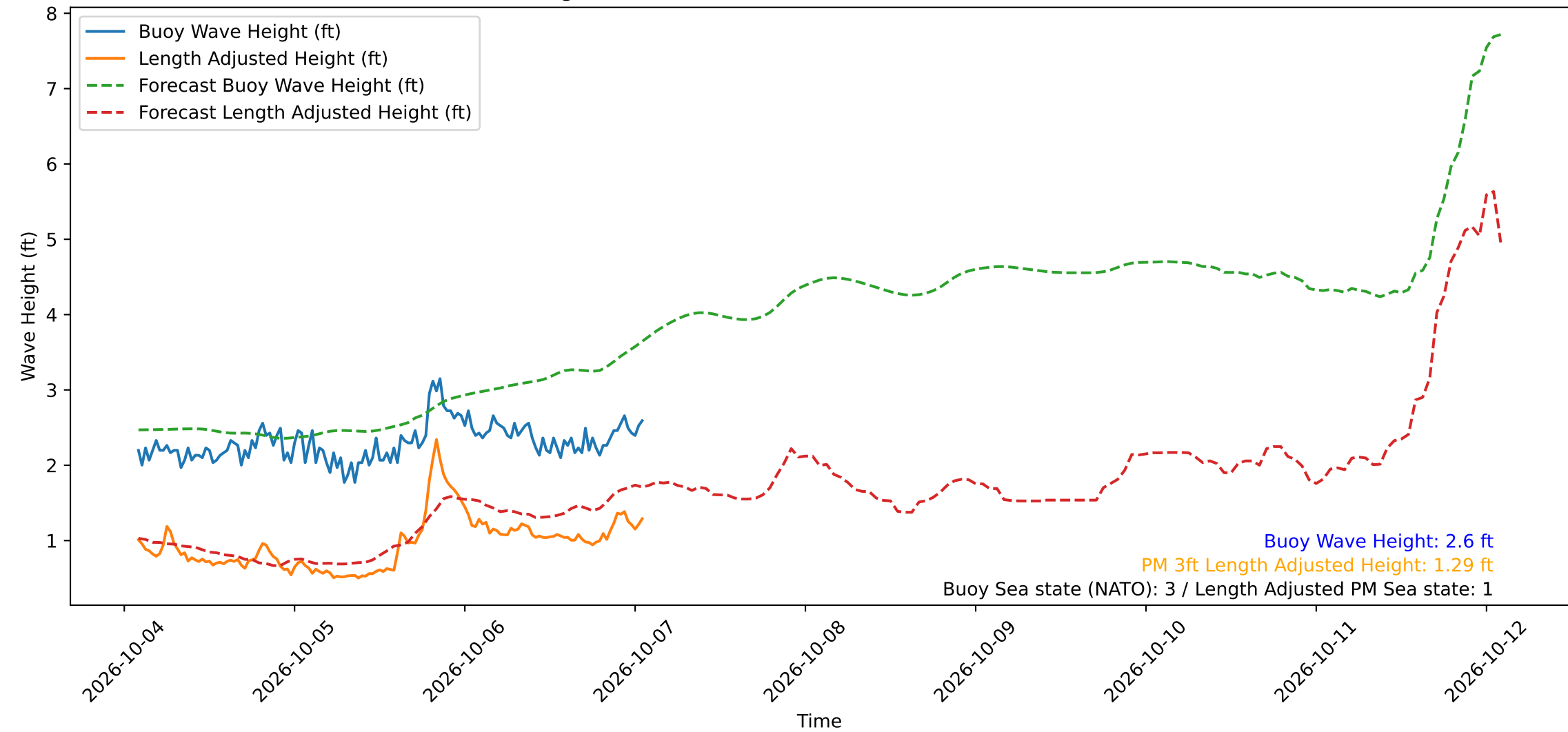
Wave Heights over Time for Green Beach at 2026-10-07 01:41:12
