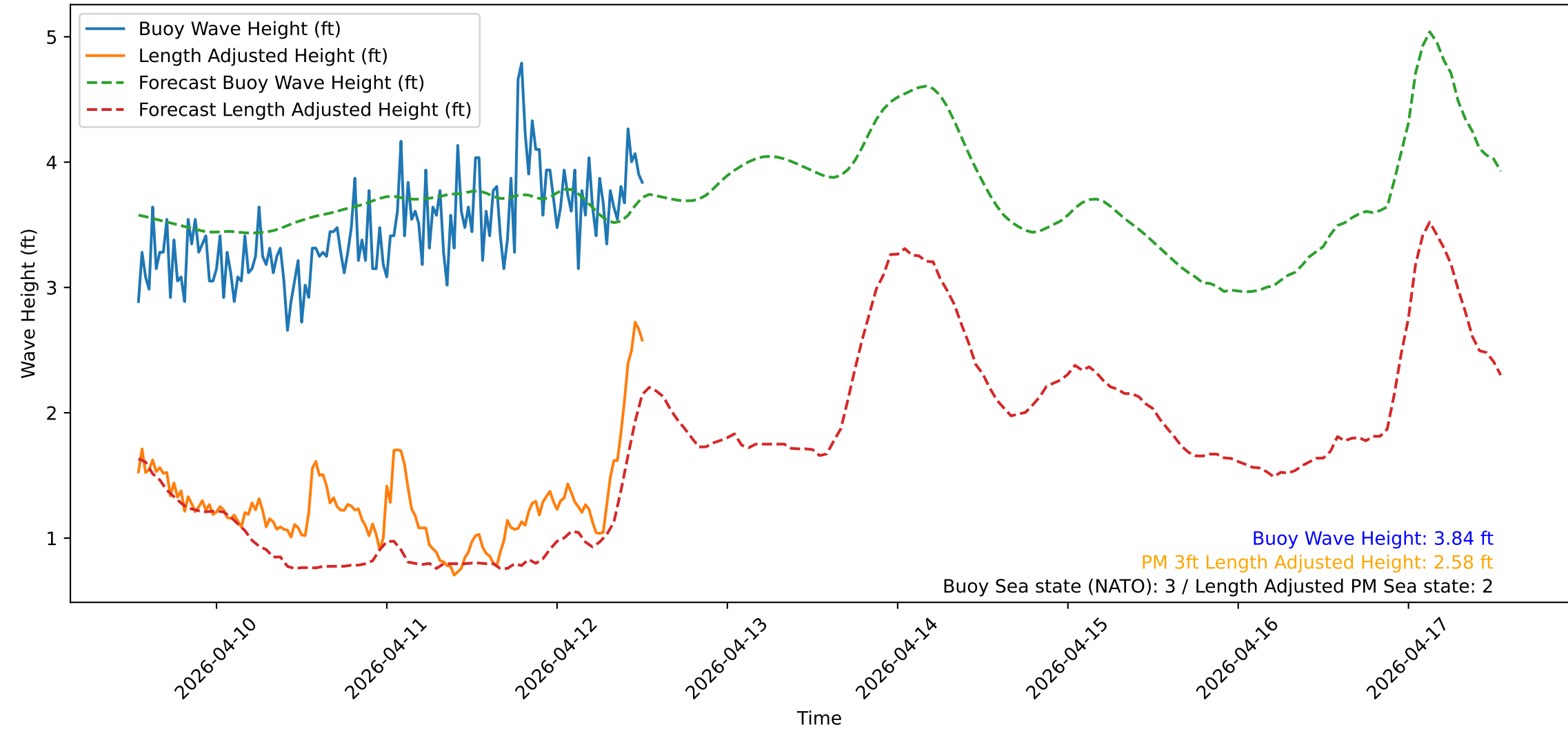
Wave Heights over Time for Oceanside Harbor at 2026-04-12 12:50:31
