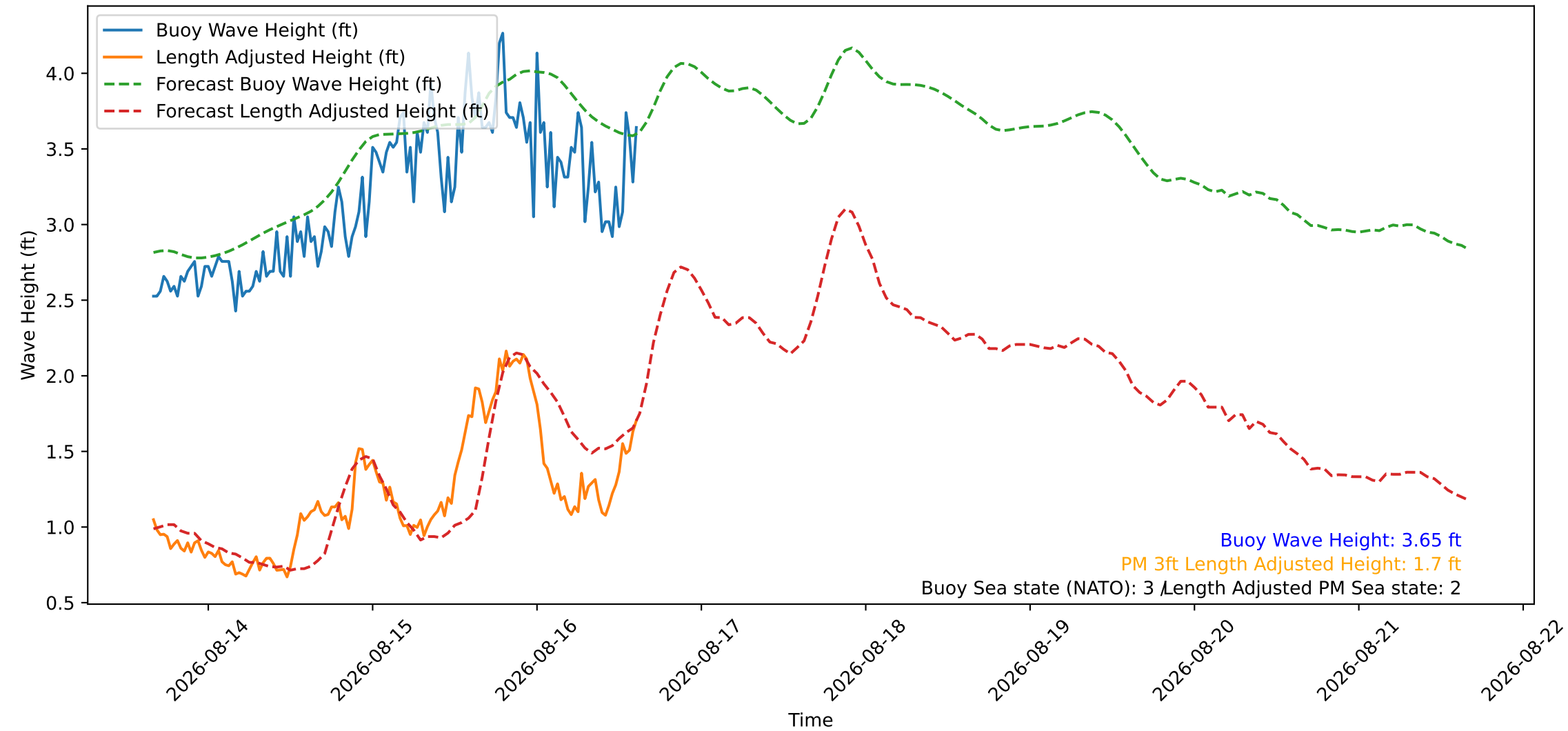
Wave Heights over Time for Green Beach at 2026-08-16 15:31:09
