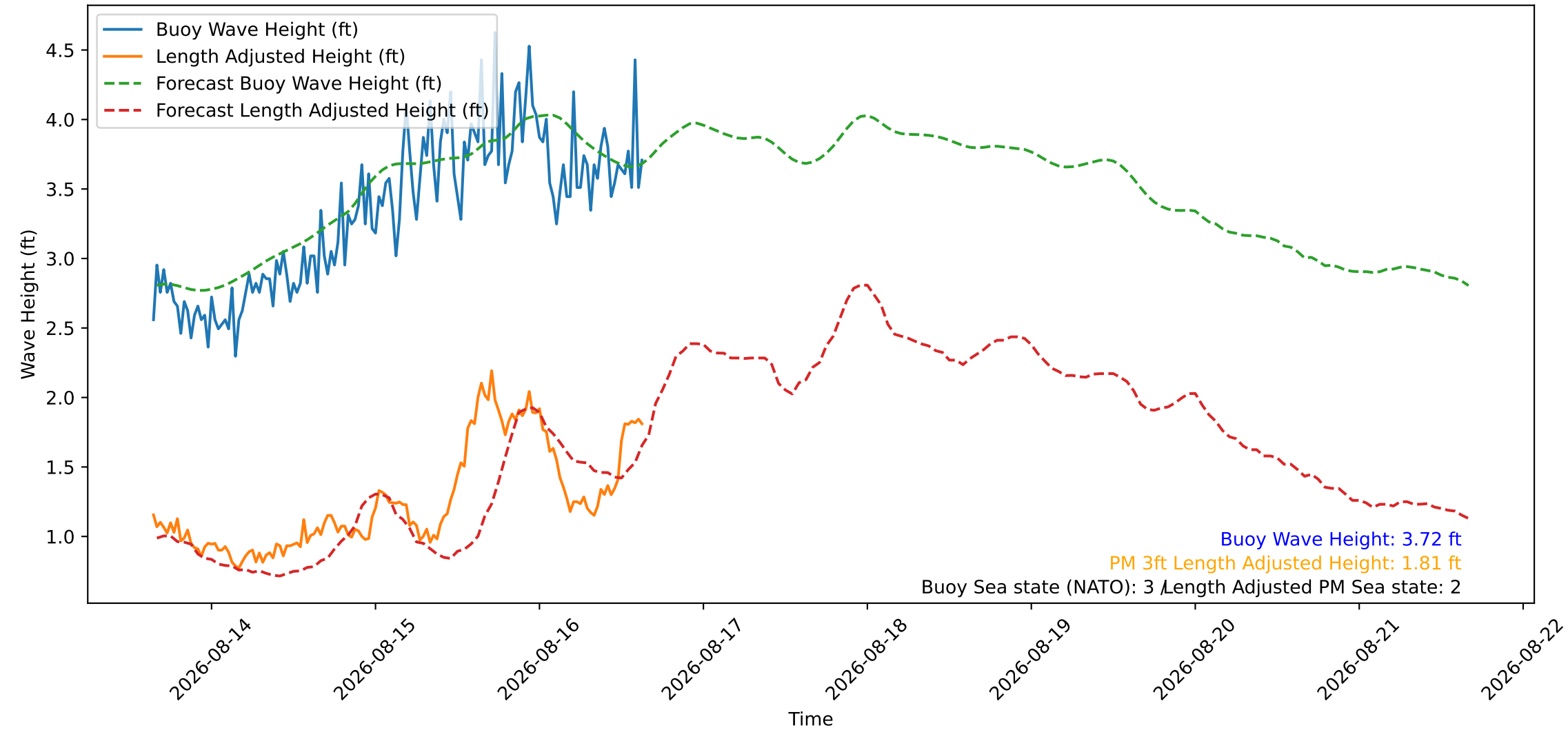
Wave Heights over Time for Oceanside Harbor at 2026-08-16 15:30:27
