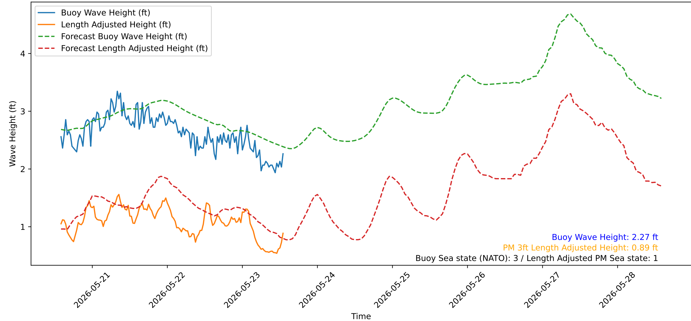
Wave Heights over Time for Red Beach at 2026-05-23 13:50:53
