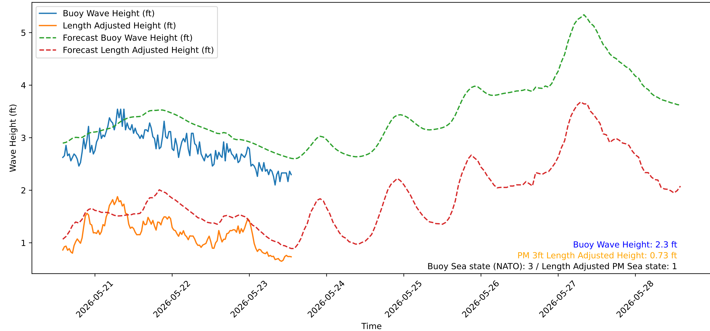
Wave Heights over Time for Green Beach at 2026-05-23 13:51:15
