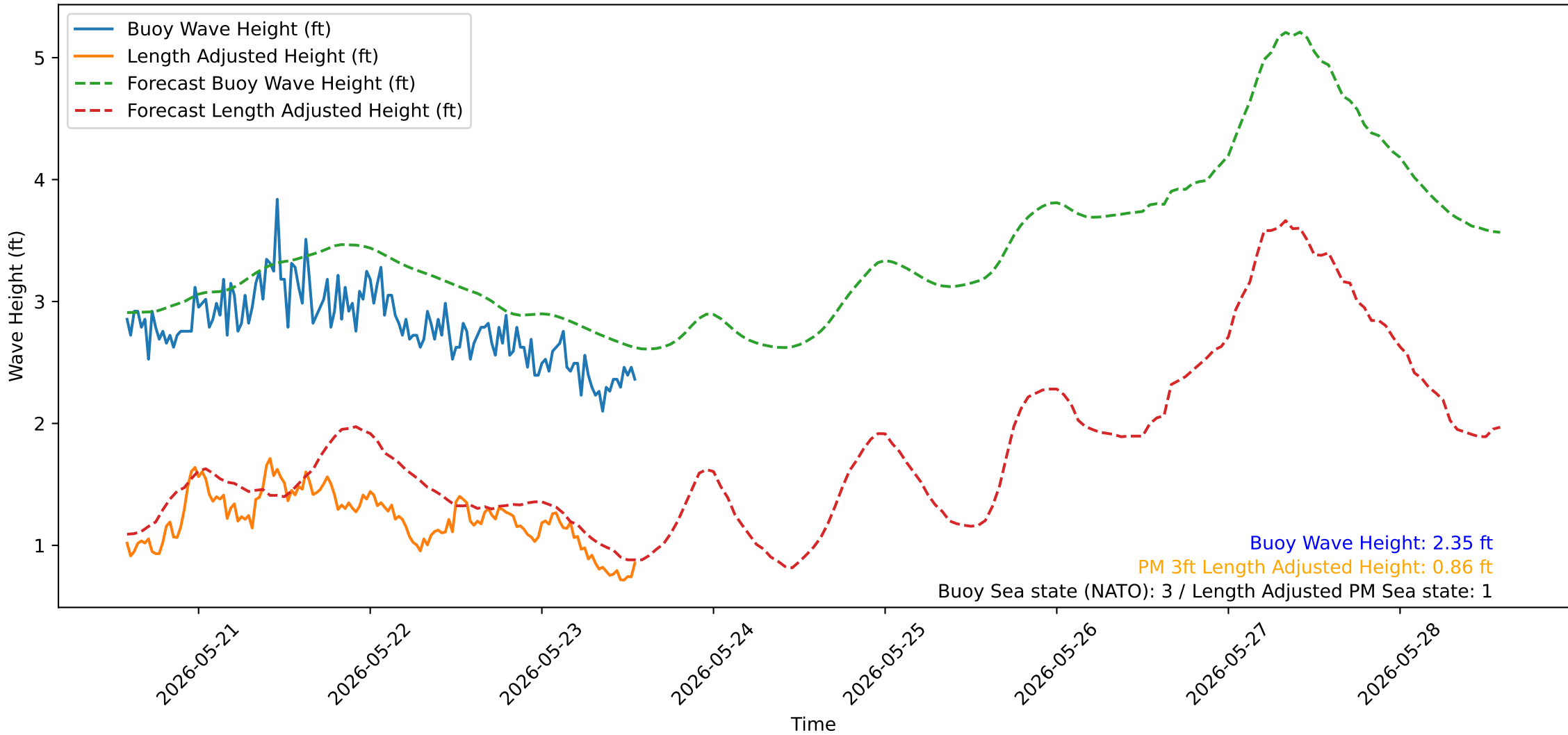
Wave Heights over Time for Oceanside Harbor at 2026-05-23 13:50:32
