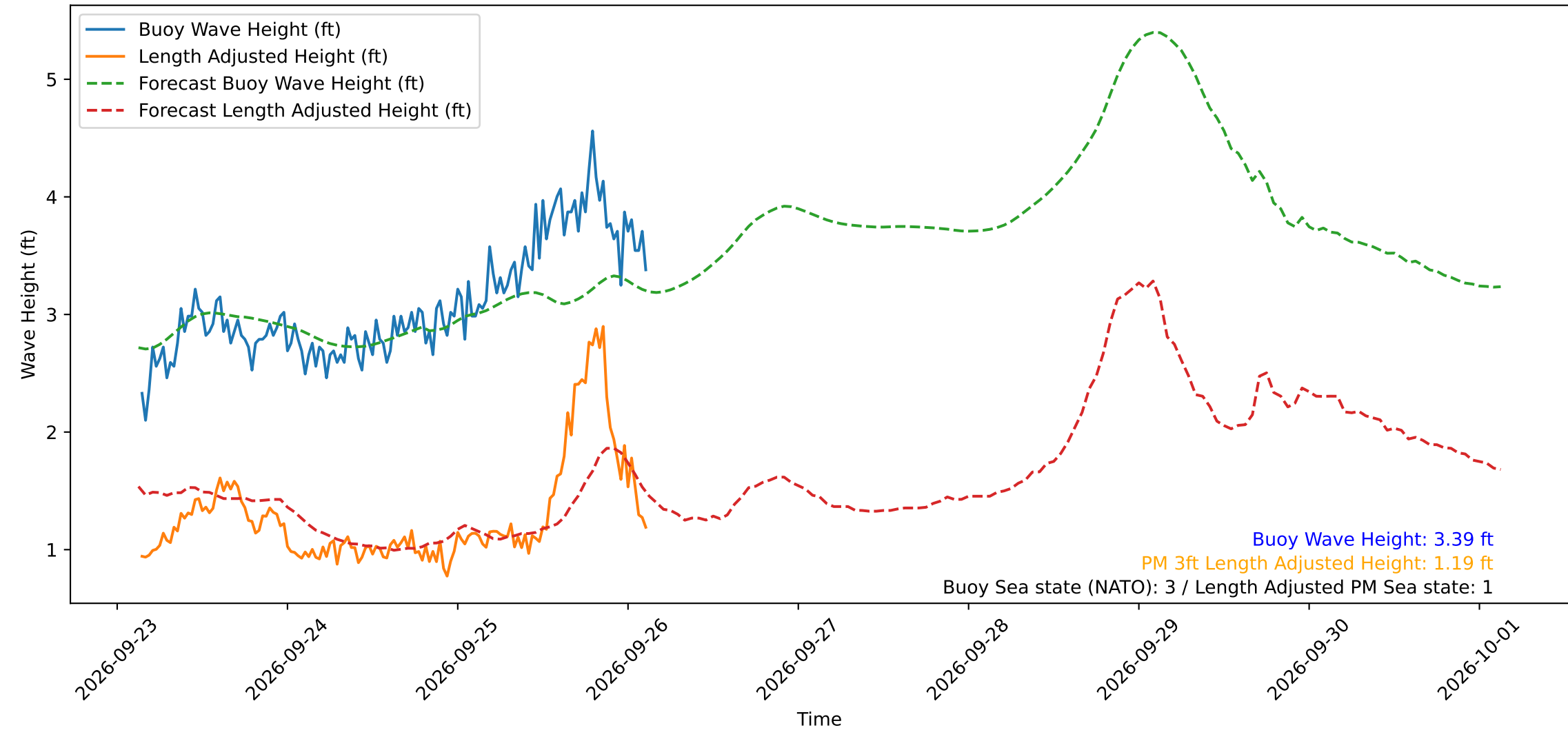
Wave Heights over Time for Green Beach at 2026-09-26 03:21:15
