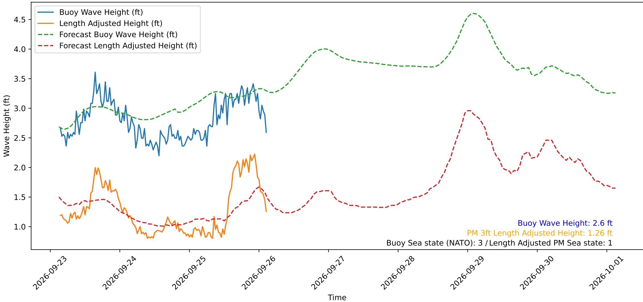
Wave Heights over Time for Oceanside Harbor at 2026-09-26 03:20:30
