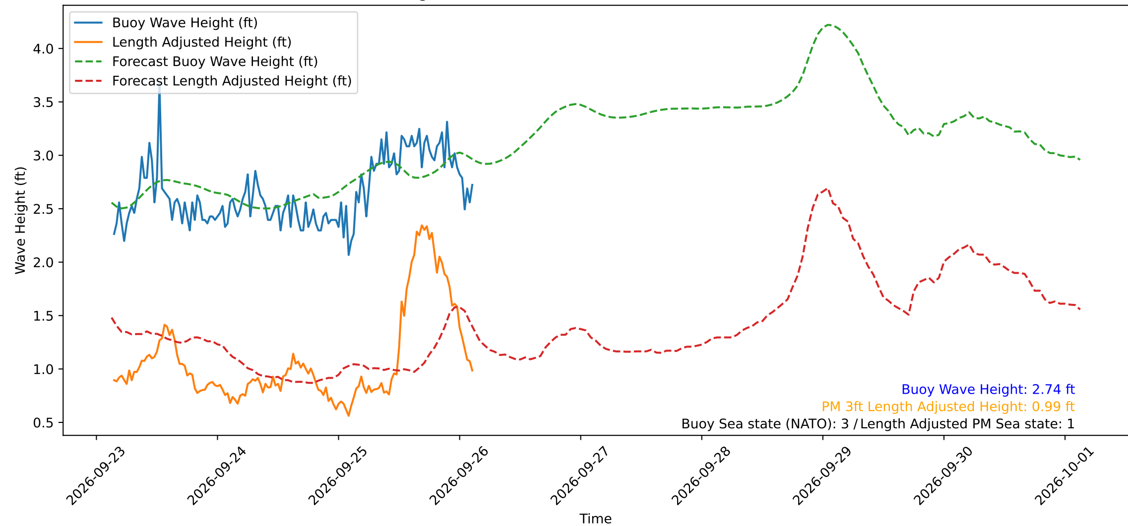
Wave Heights over Time for Red Beach at 2026-09-26 03:20:51
