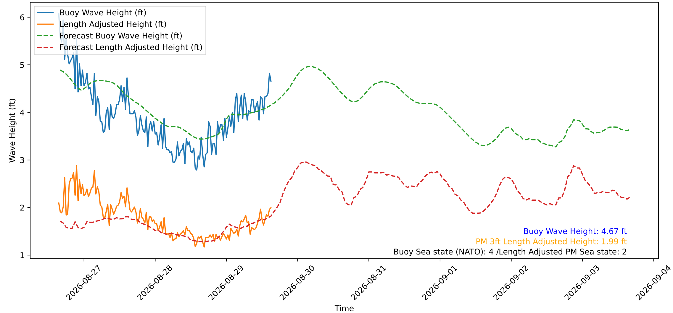
Wave Heights over Time for Oceanside Harbor at 2026-08-29 15:40:30
