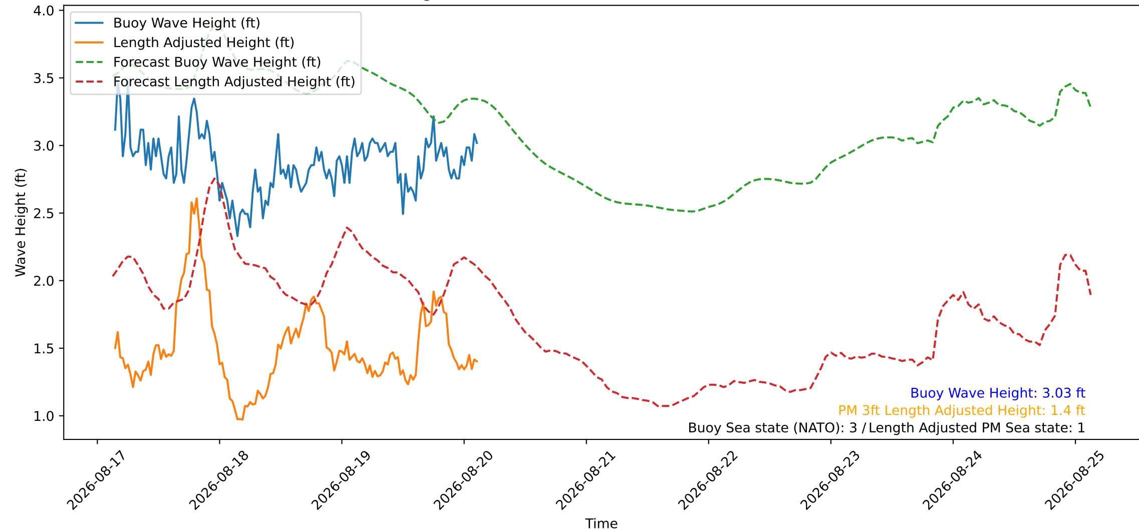
Wave Heights over Time for Red Beach at 2026-08-20 03:10:46
