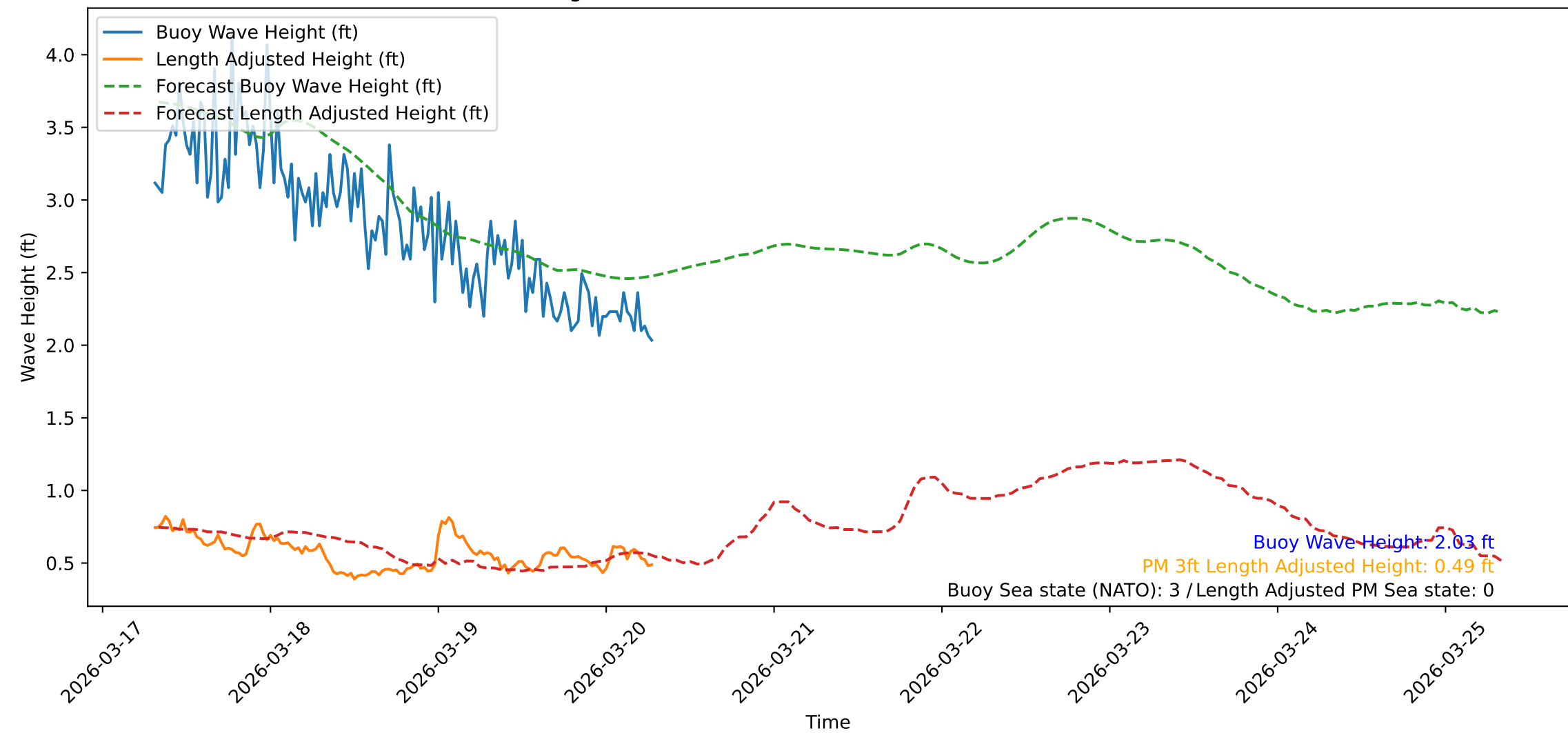
Wave Heights over Time for Green Beach at 2026-03-20 07:31:10
