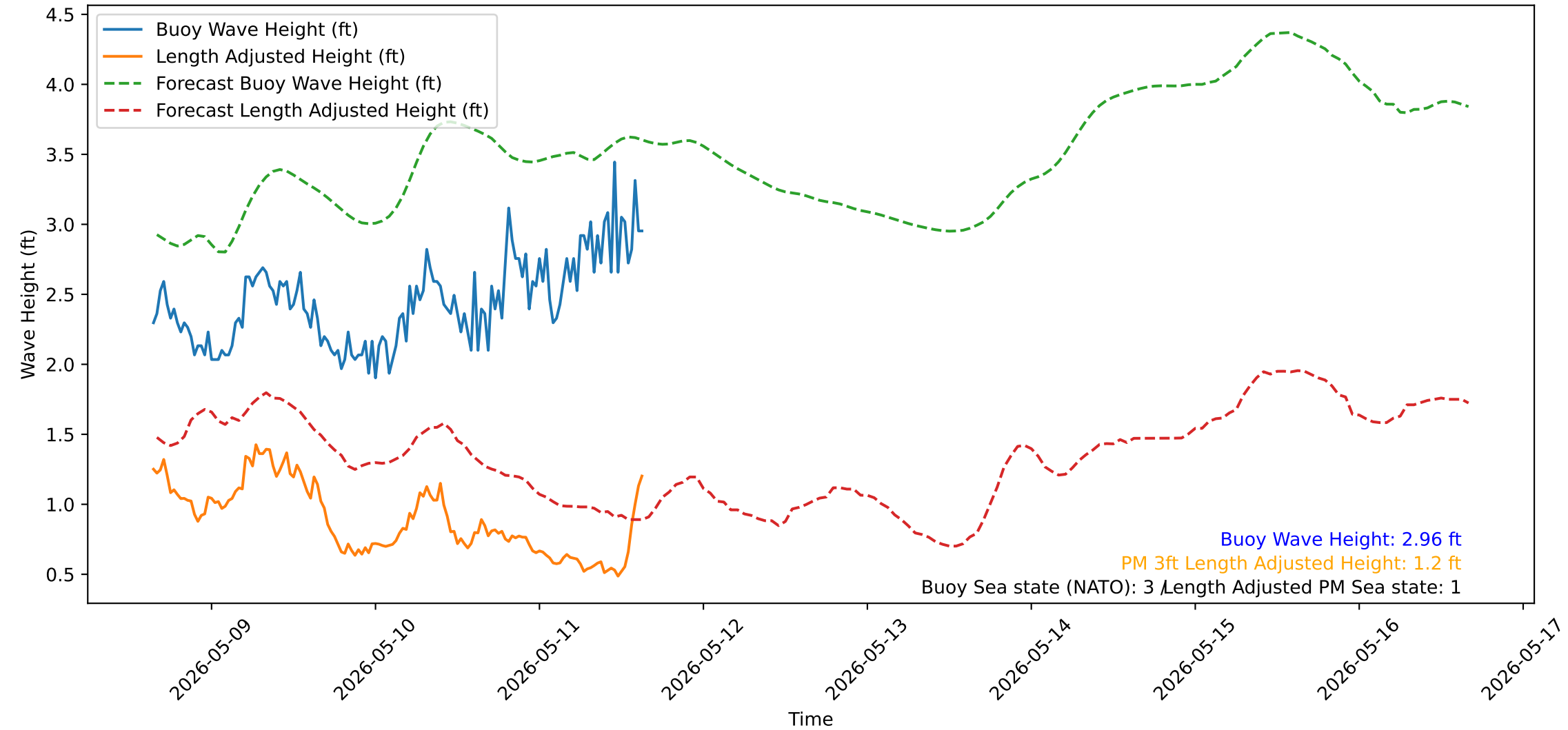
Wave Heights over Time for Green Beach at 2026-05-11 15:41:13
