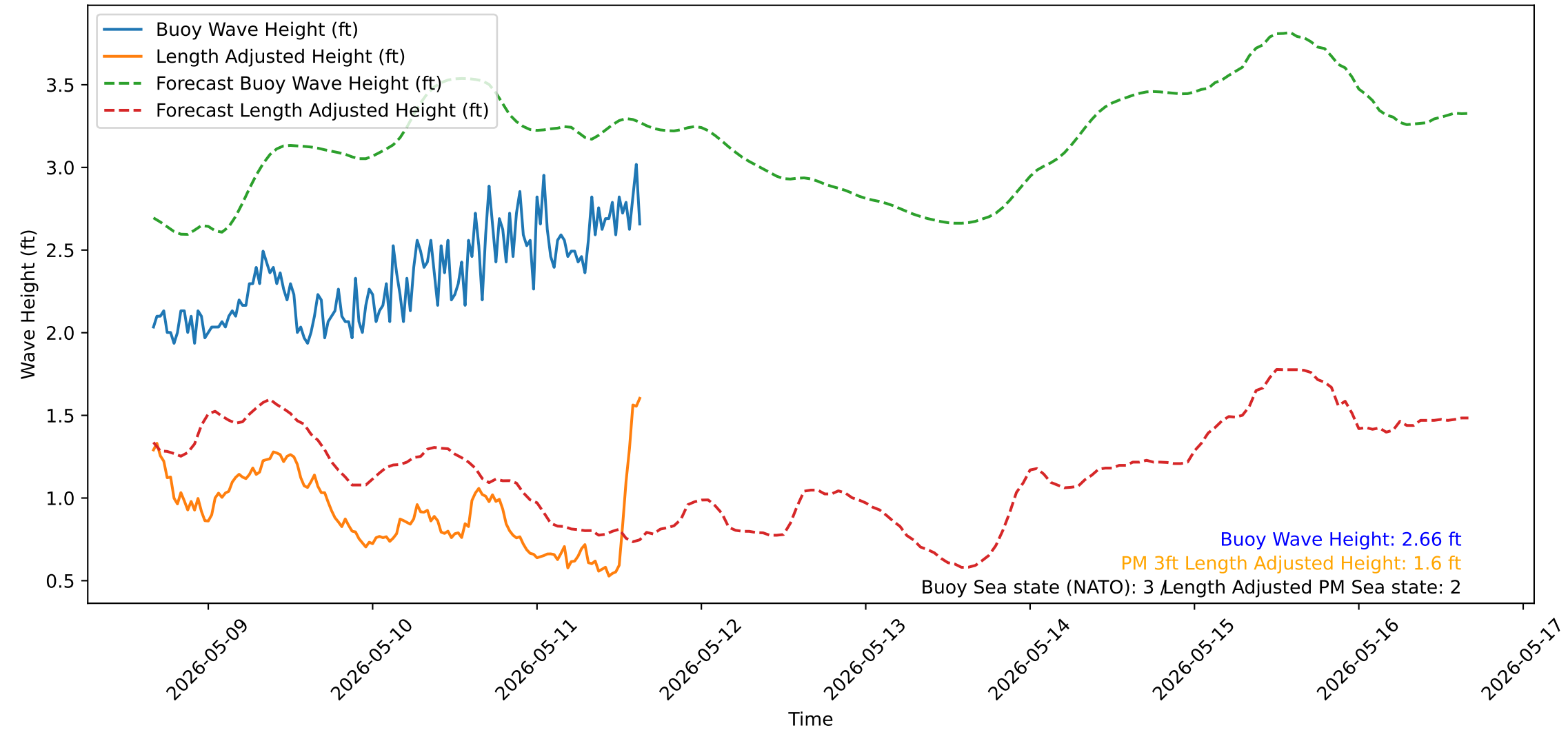
Wave Heights over Time for Red Beach at 2026-05-11 15:40:51
