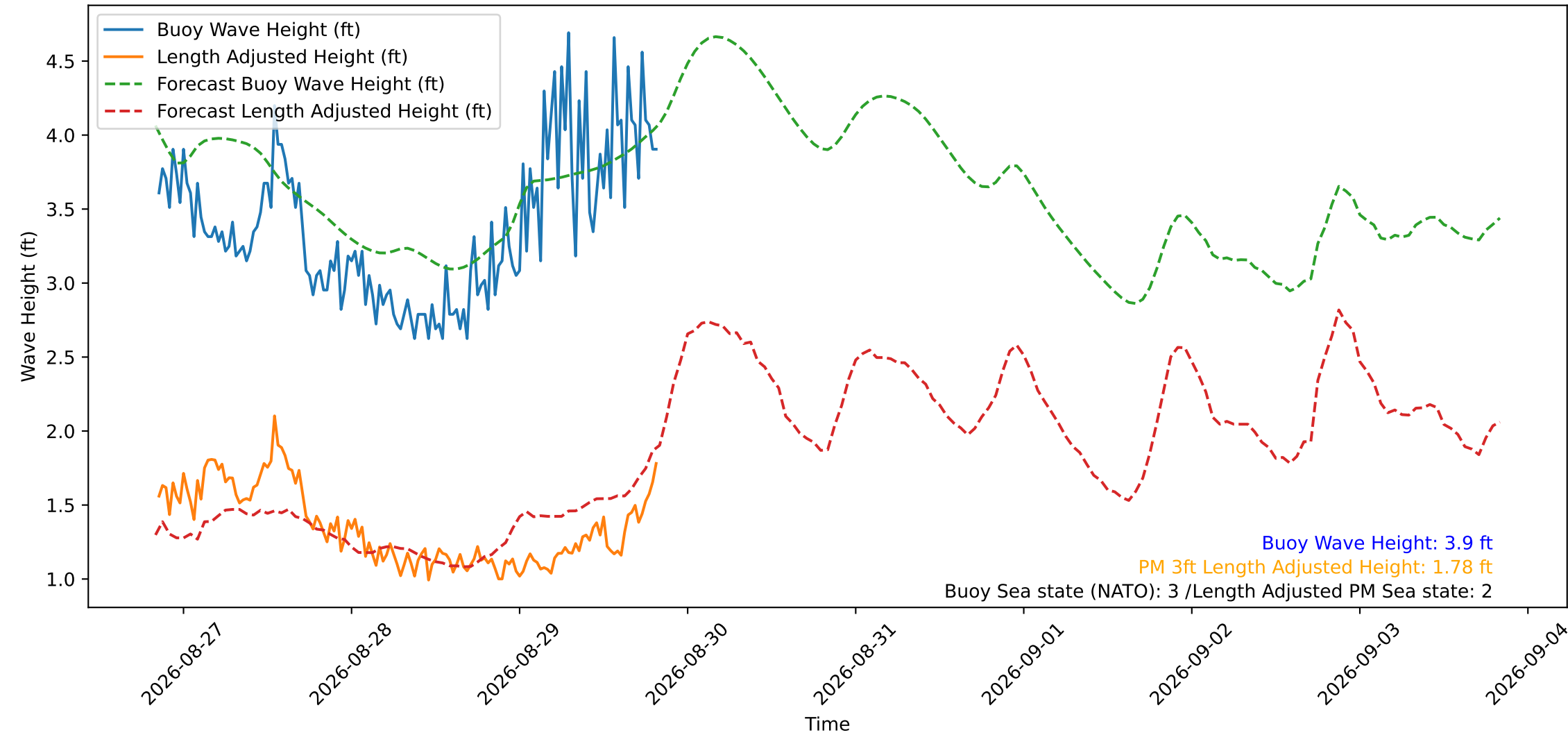
Wave Heights over Time for Red Beach at 2026-08-29 20:20:54
