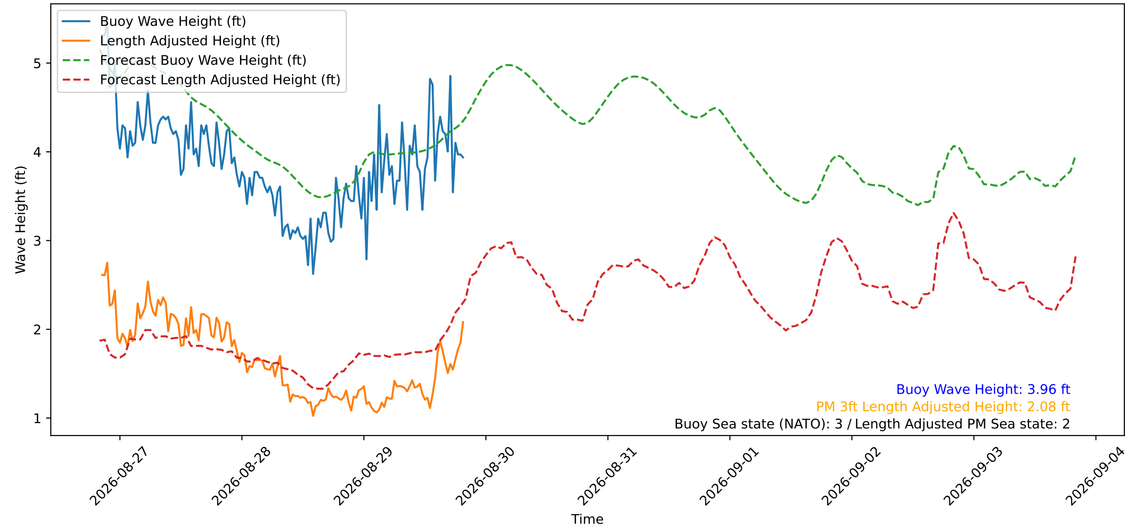
Wave Heights over Time for Green Beach at 2026-08-29 20:21:18
