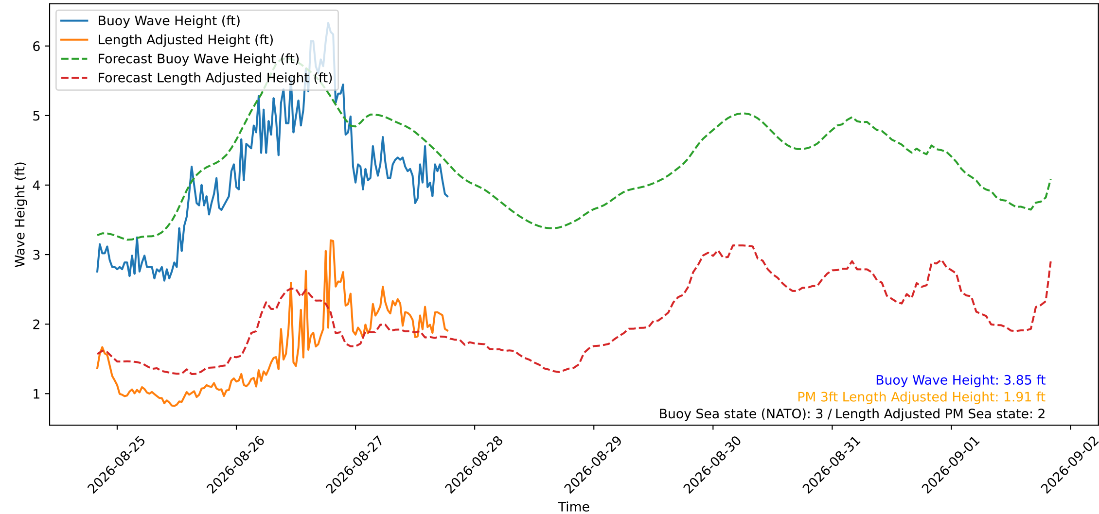
Wave Heights over Time for Green Beach at 2026-08-27 19:31:12
