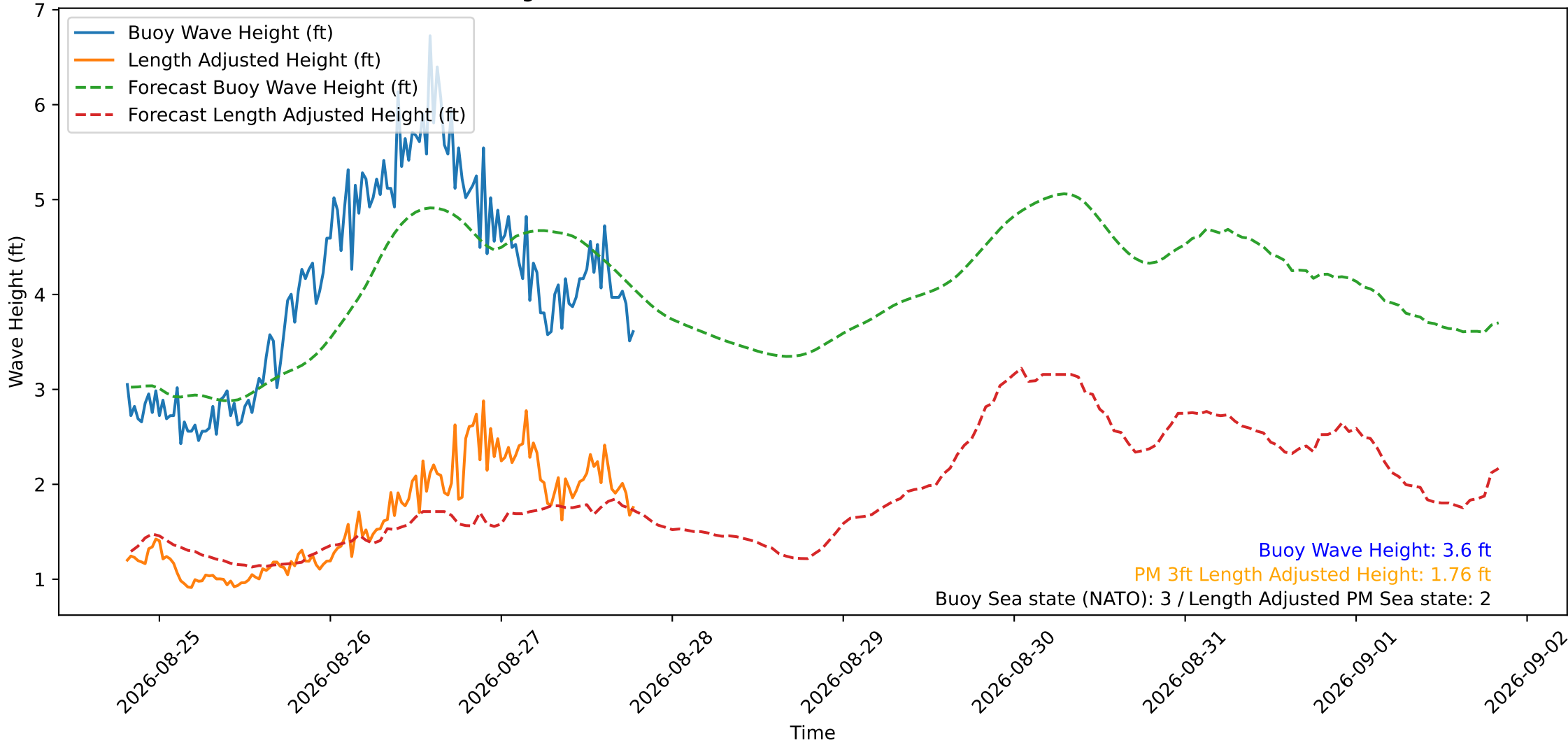
Wave Heights over Time for Oceanside Harbor at 2026-08-27 19:30:30
