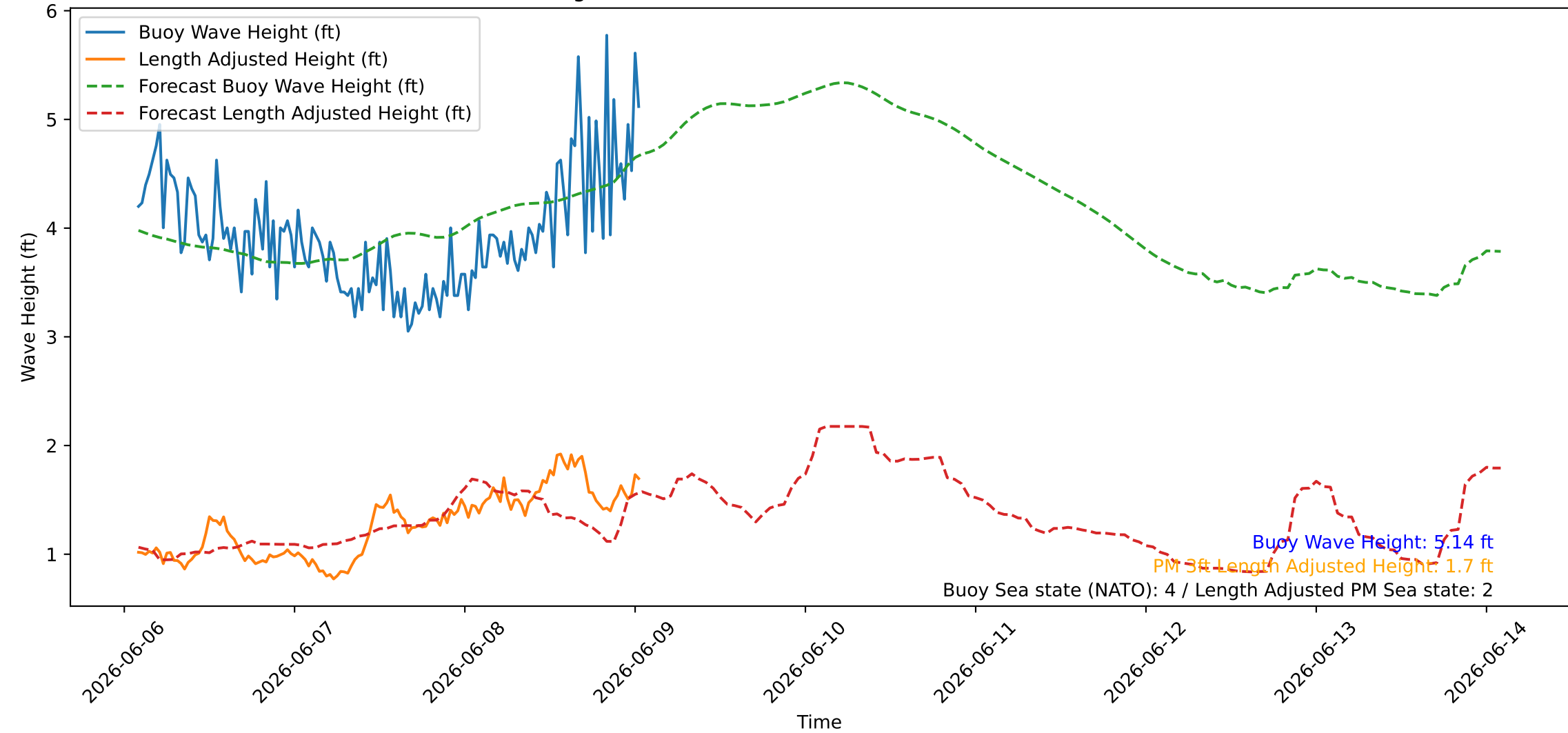
Wave Heights over Time for Red Beach at 2026-06-09 01:30:45
