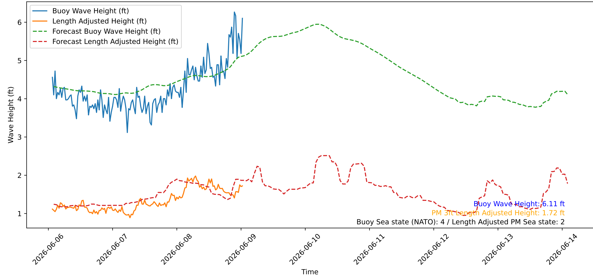
Wave Heights over Time for Green Beach at 2026-06-09 01:31:08
