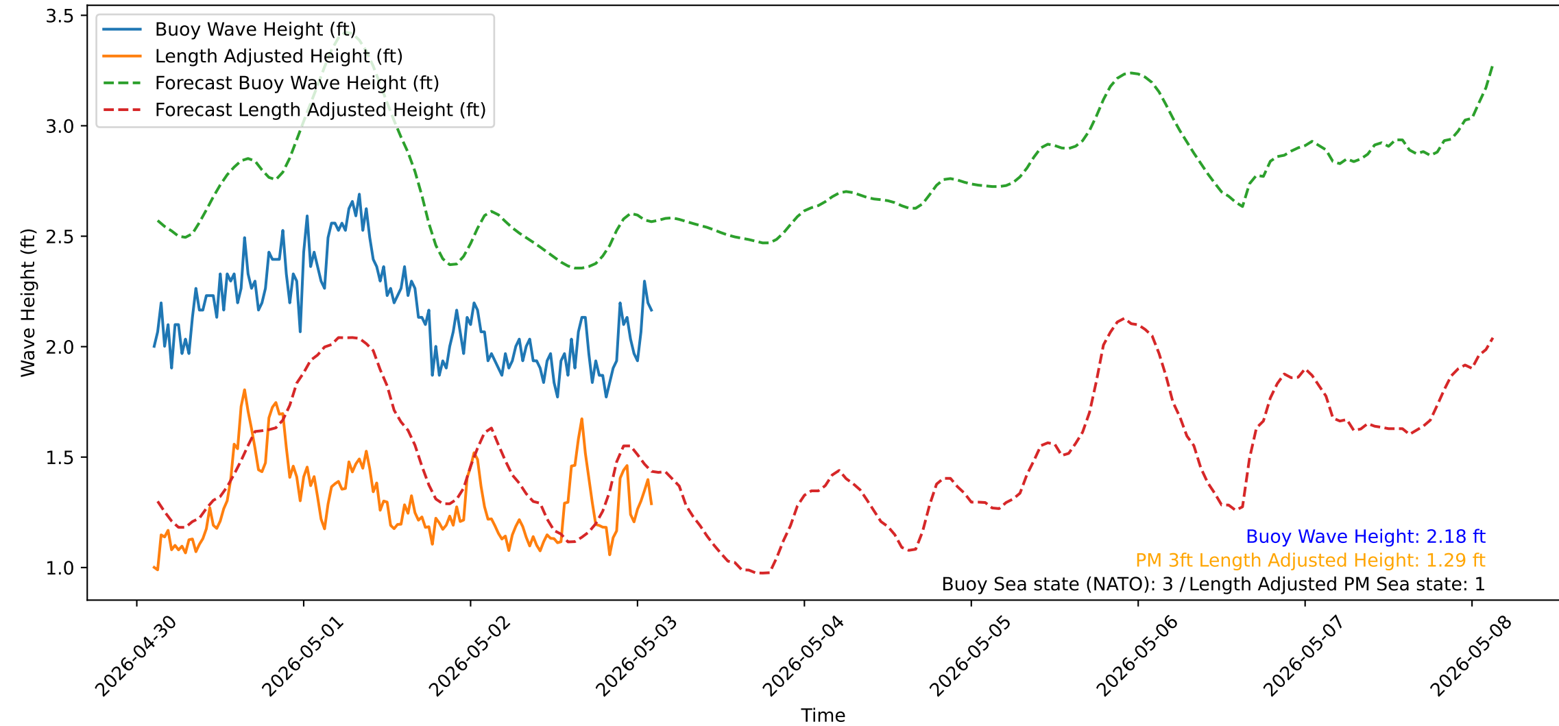
Wave Heights over Time for Oceanside Harbor at 2026-05-03 02:30:31
