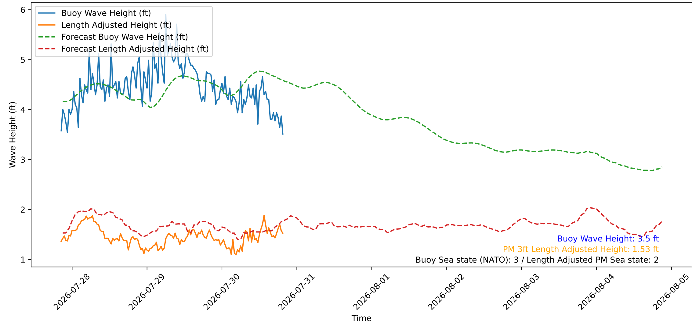
Wave Heights over Time for Oceanside Harbor at 2026-07-30 20:40:26
