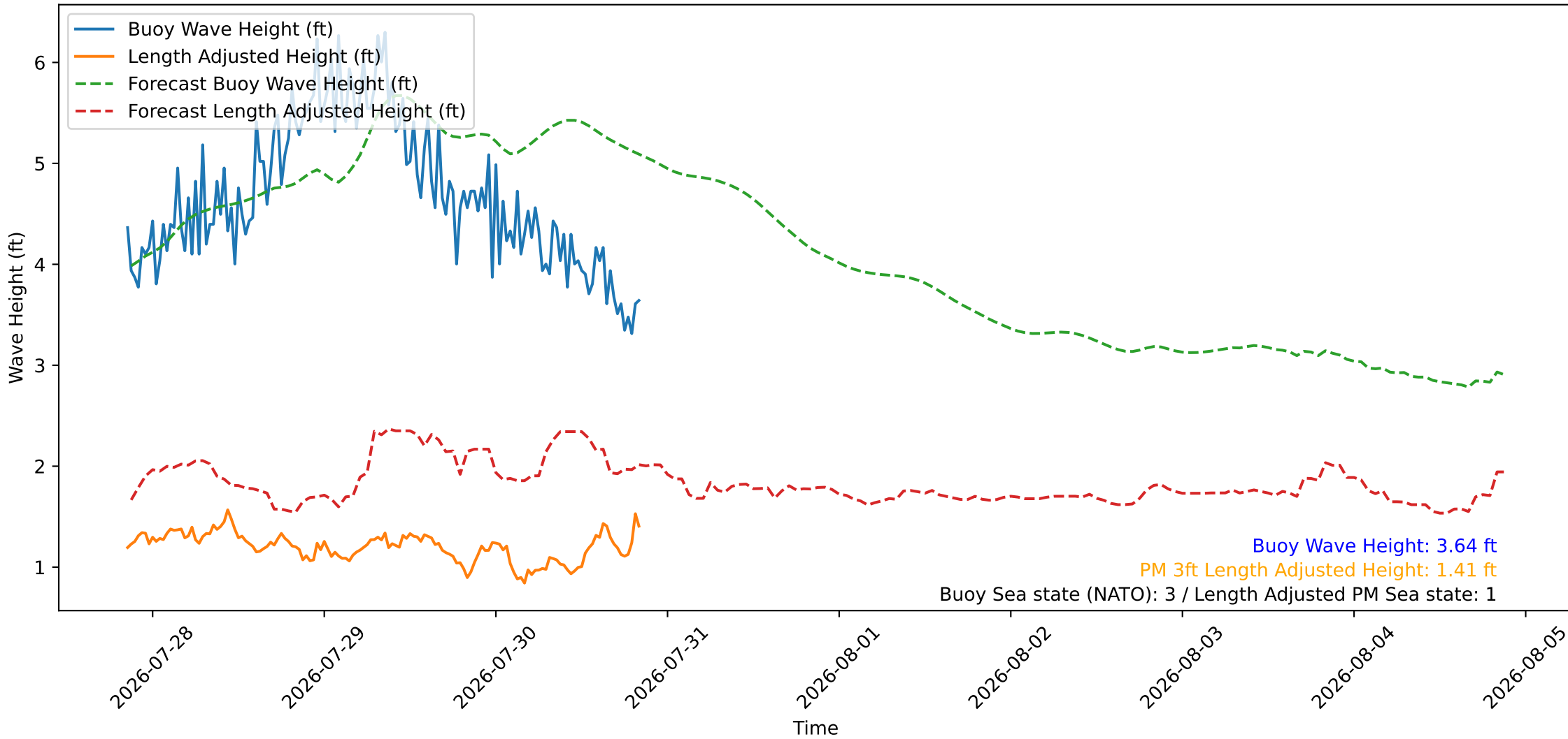
Wave Heights over Time for Green Beach at 2026-07-30 20:41:08
