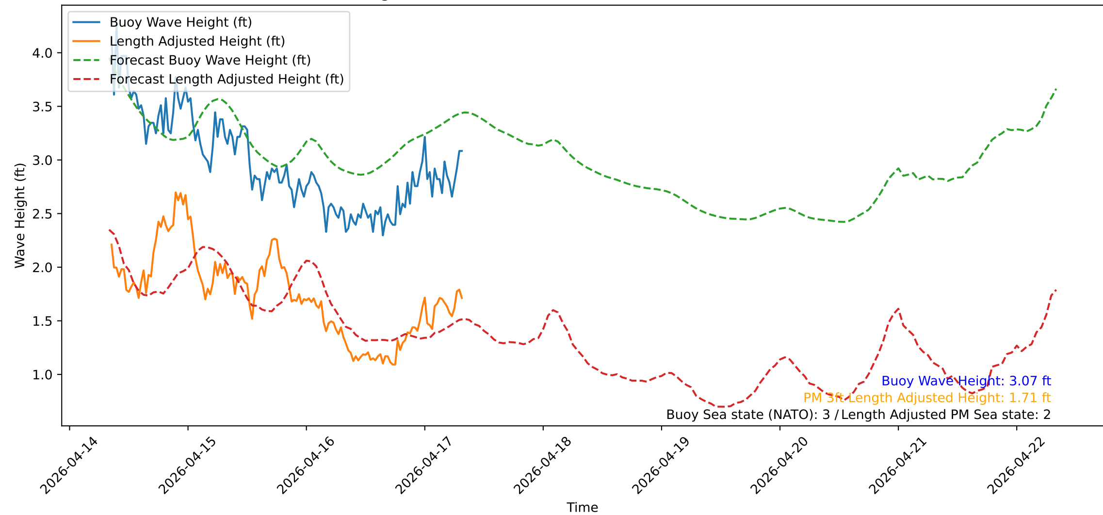
Wave Heights over Time for Oceanside Harbor at 2026-04-17 08:20:31
