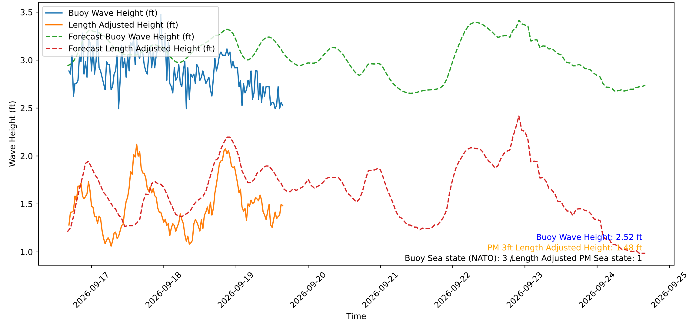
Wave Heights over Time for Green Beach at 2026-09-19 16:11:10
