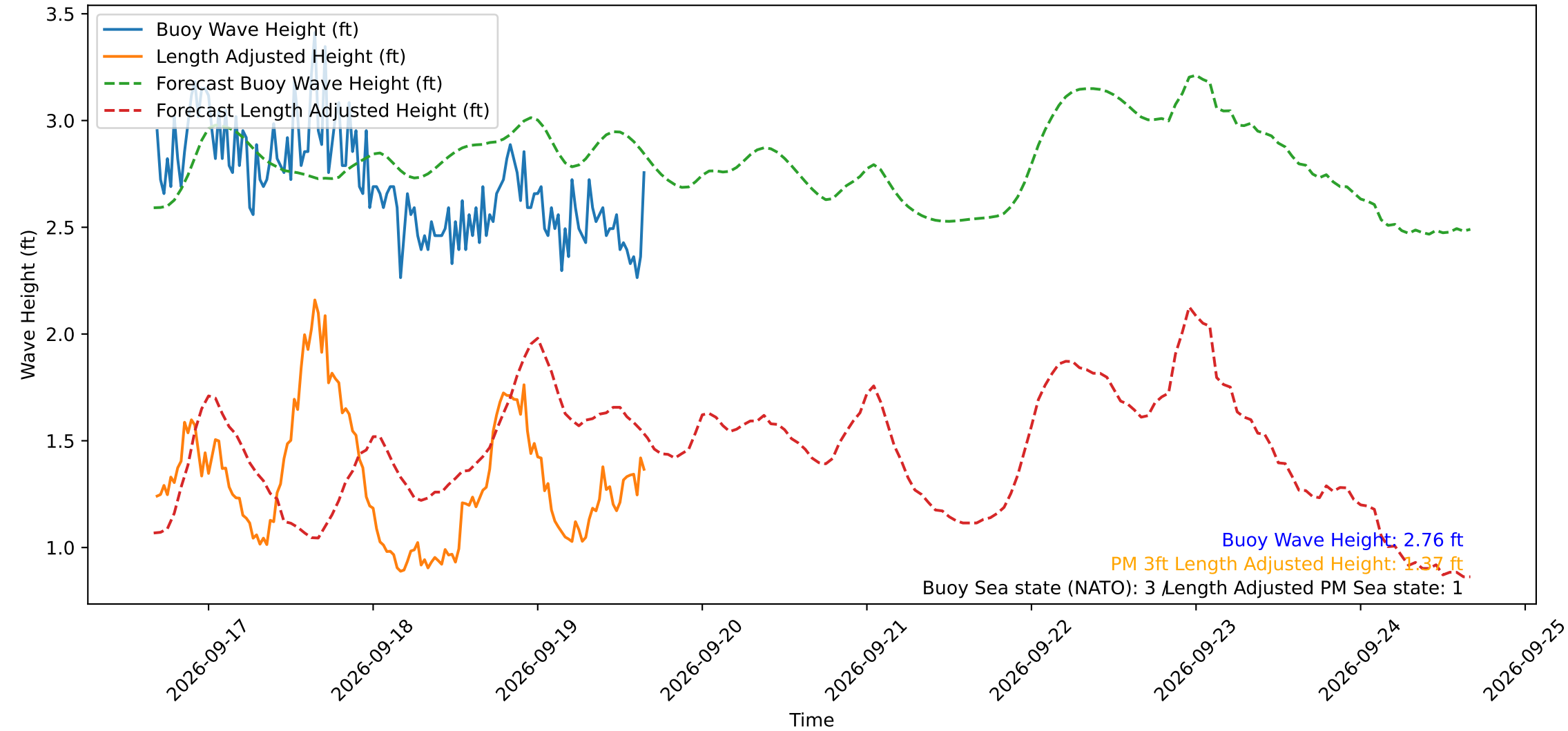
Wave Heights over Time for Red Beach at 2026-09-19 16:10:48
