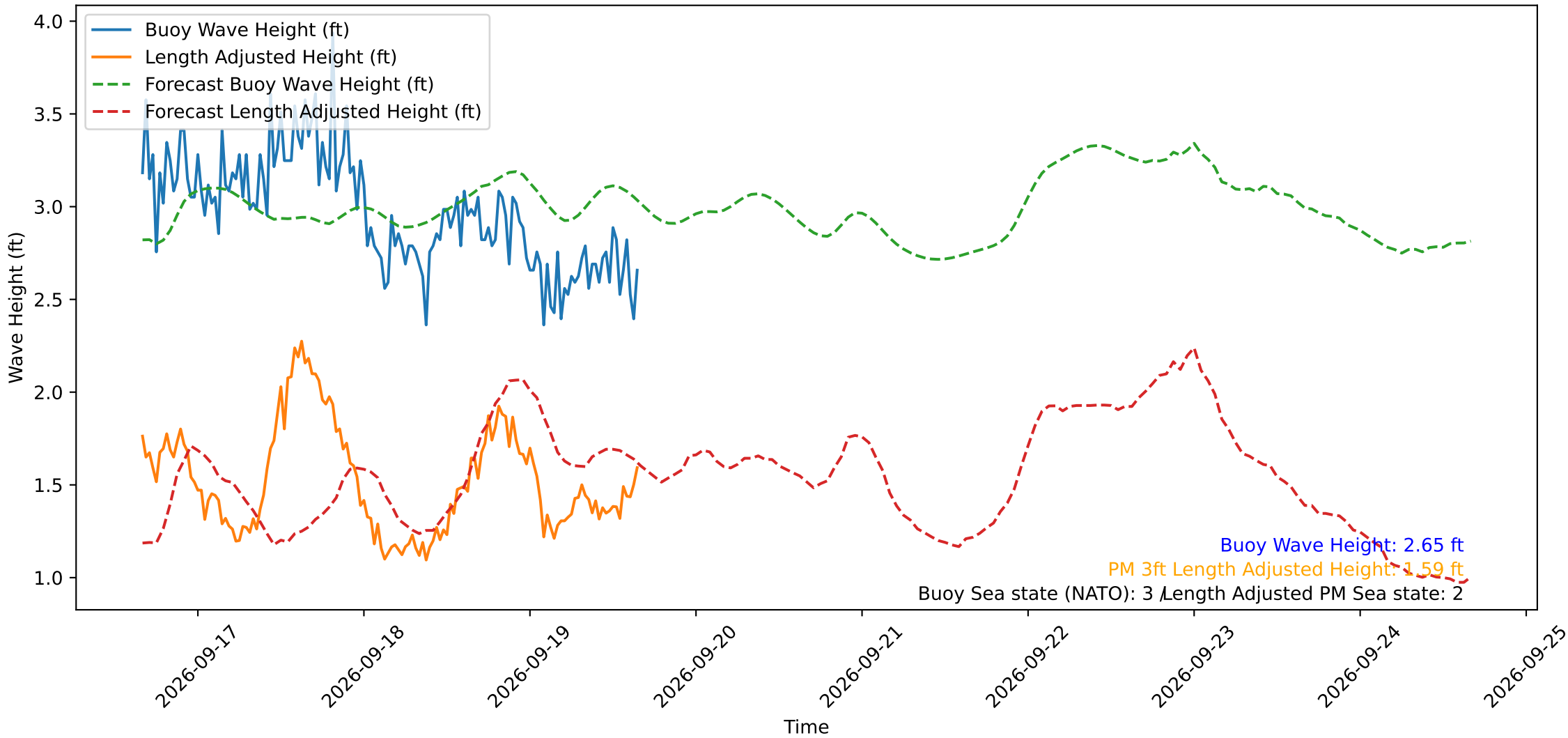
Wave Heights over Time for Oceanside Harbor at 2026-09-19 16:10:29
