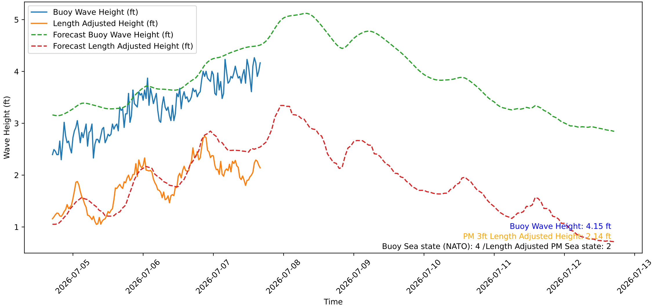
Wave Heights over Time for Oceanside Harbor at 2026-07-07 16:50:26
