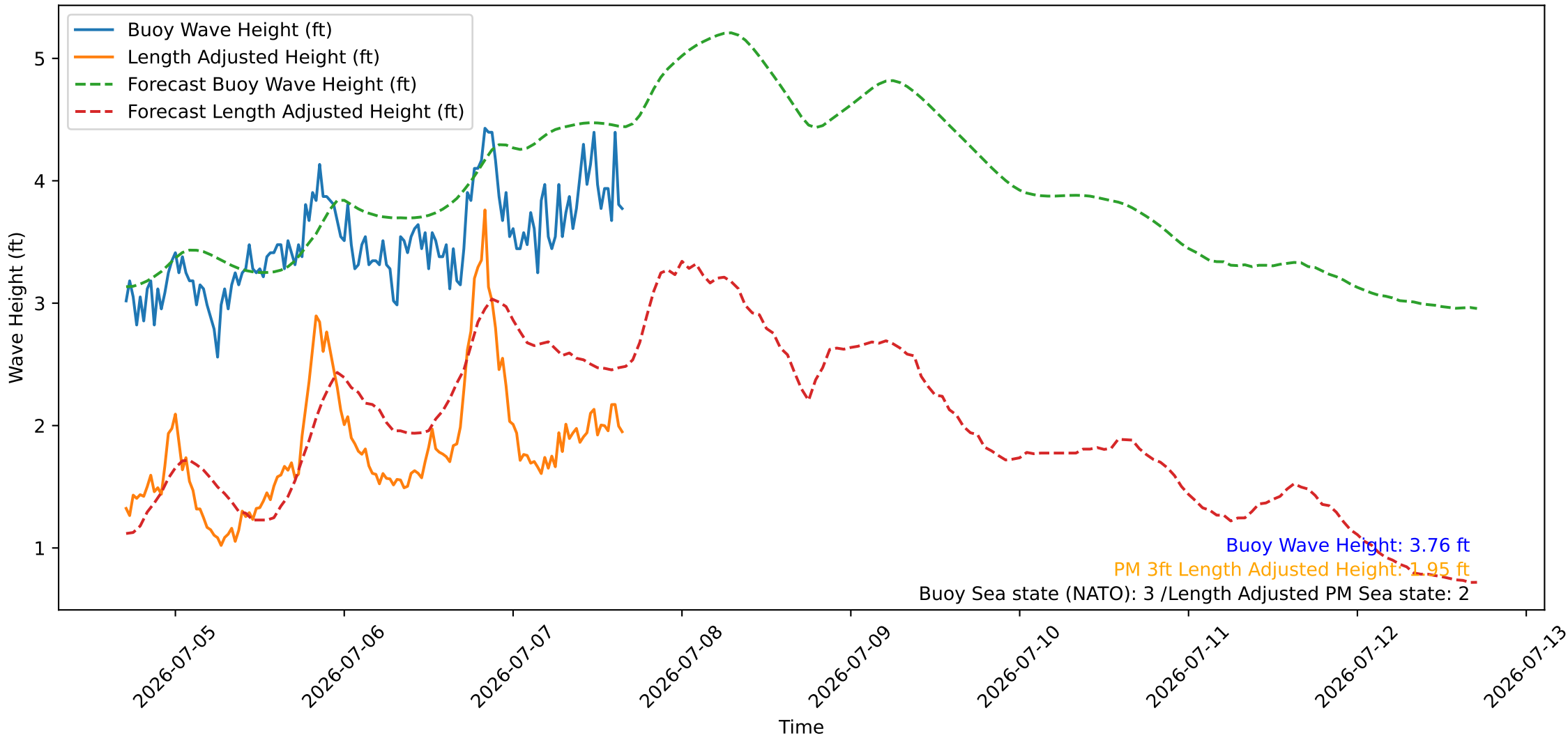
Wave Heights over Time for Green Beach at 2026-07-07 16:51:09
