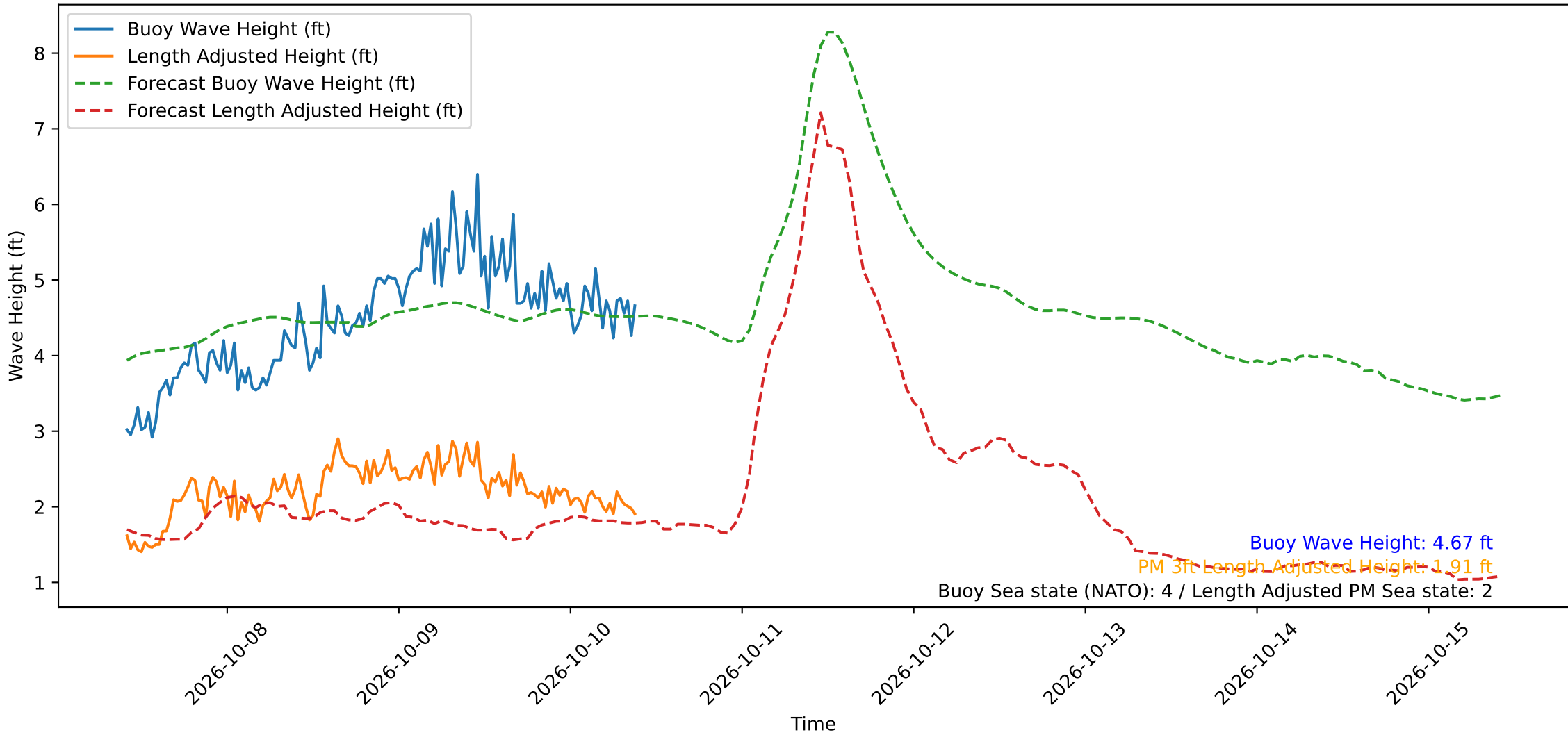
Wave Heights over Time for Oceanside Harbor at 2026-10-10 09:50:30
