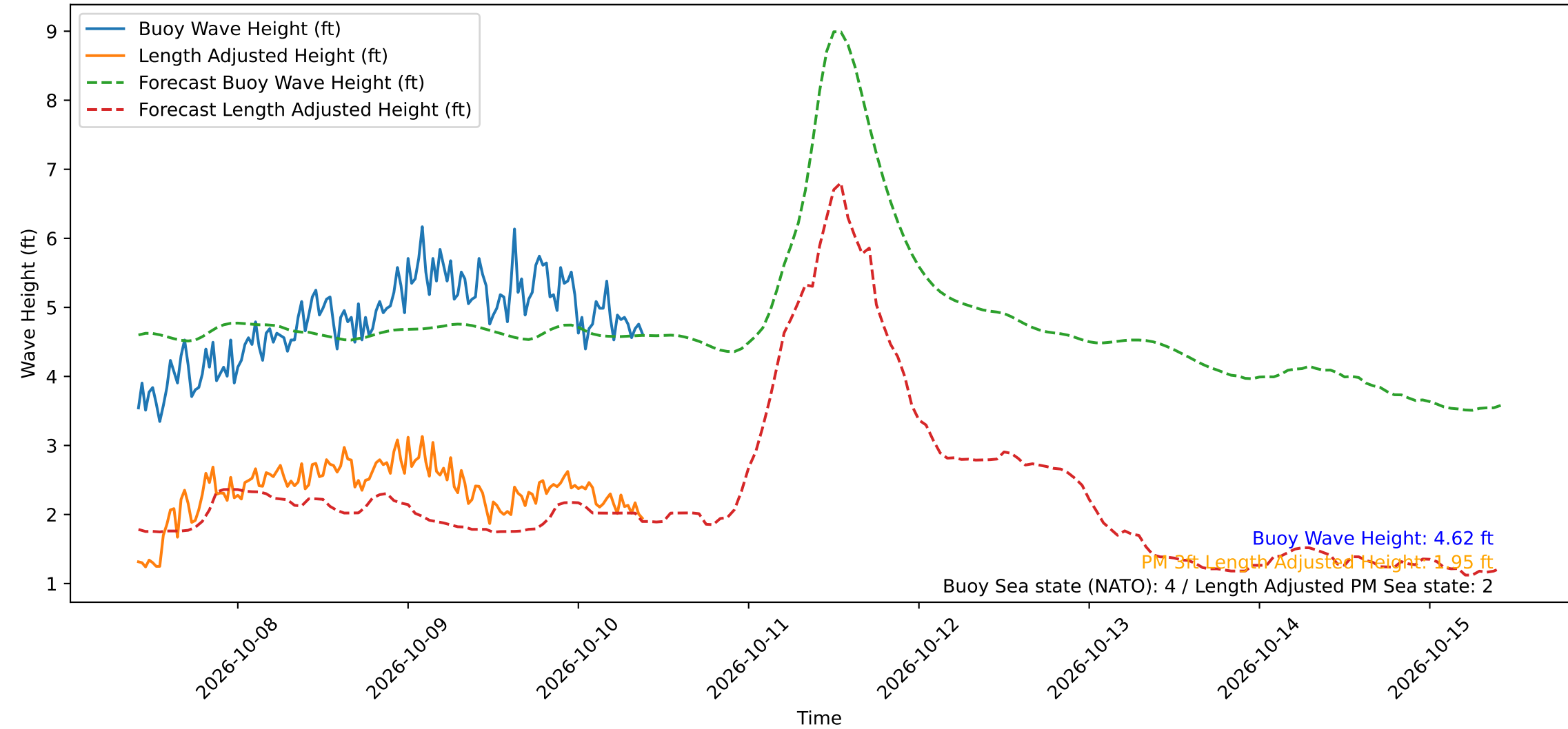
Wave Heights over Time for Green Beach at 2026-10-10 09:51:14
