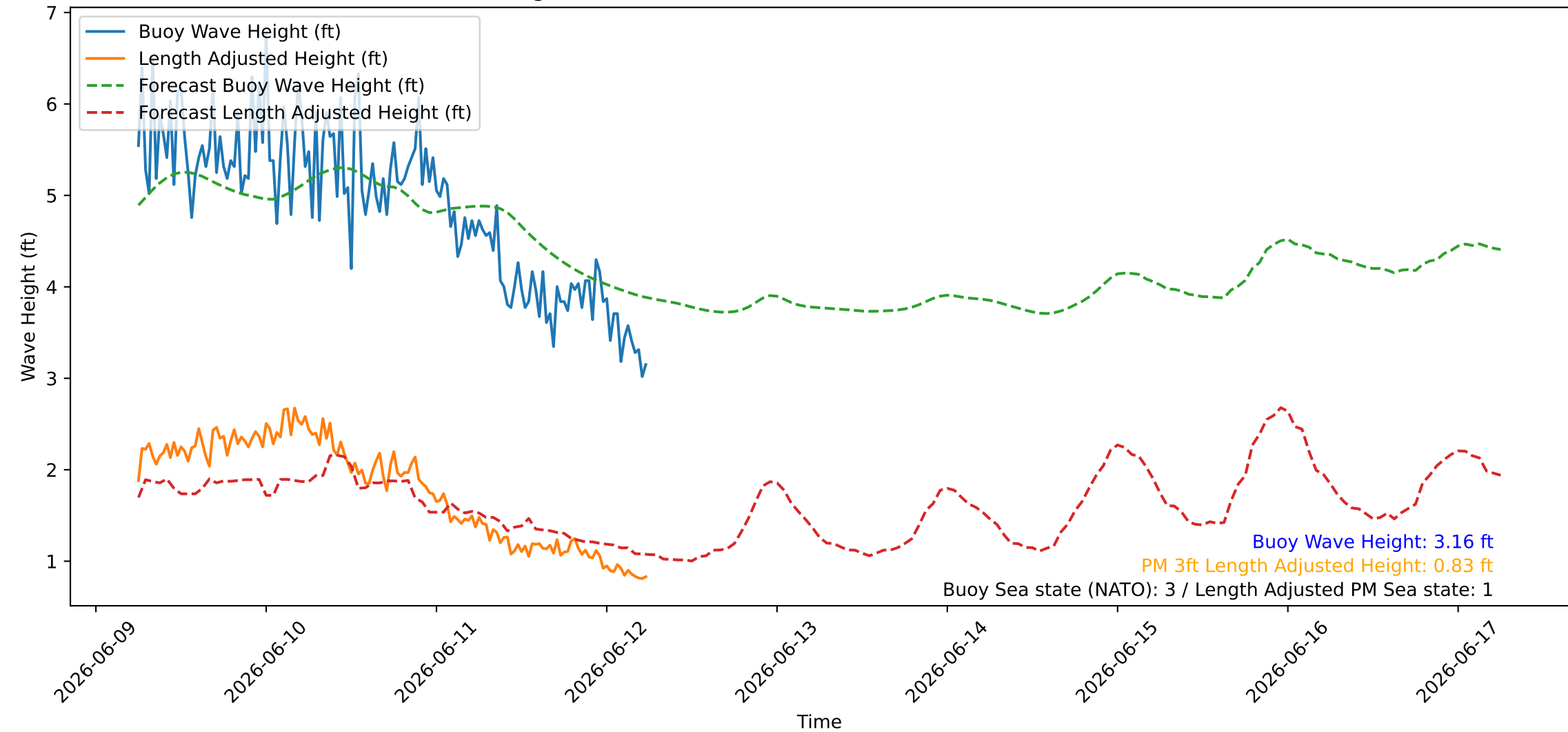
Wave Heights over Time for Oceanside Harbor at 2026-06-12 06:00:27
