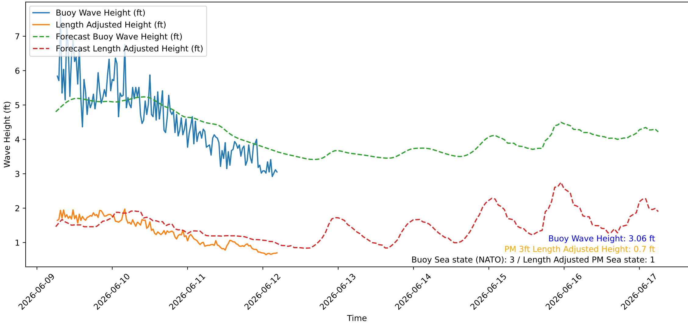
Wave Heights over Time for Red Beach at 2026-06-12 06:00:46
