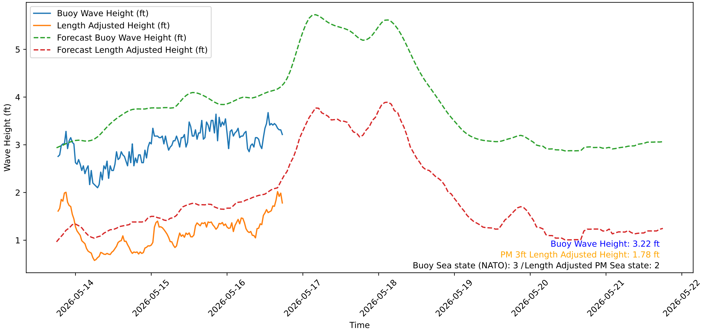
Wave Heights over Time for Green Beach at 2026-05-16 18:21:15
