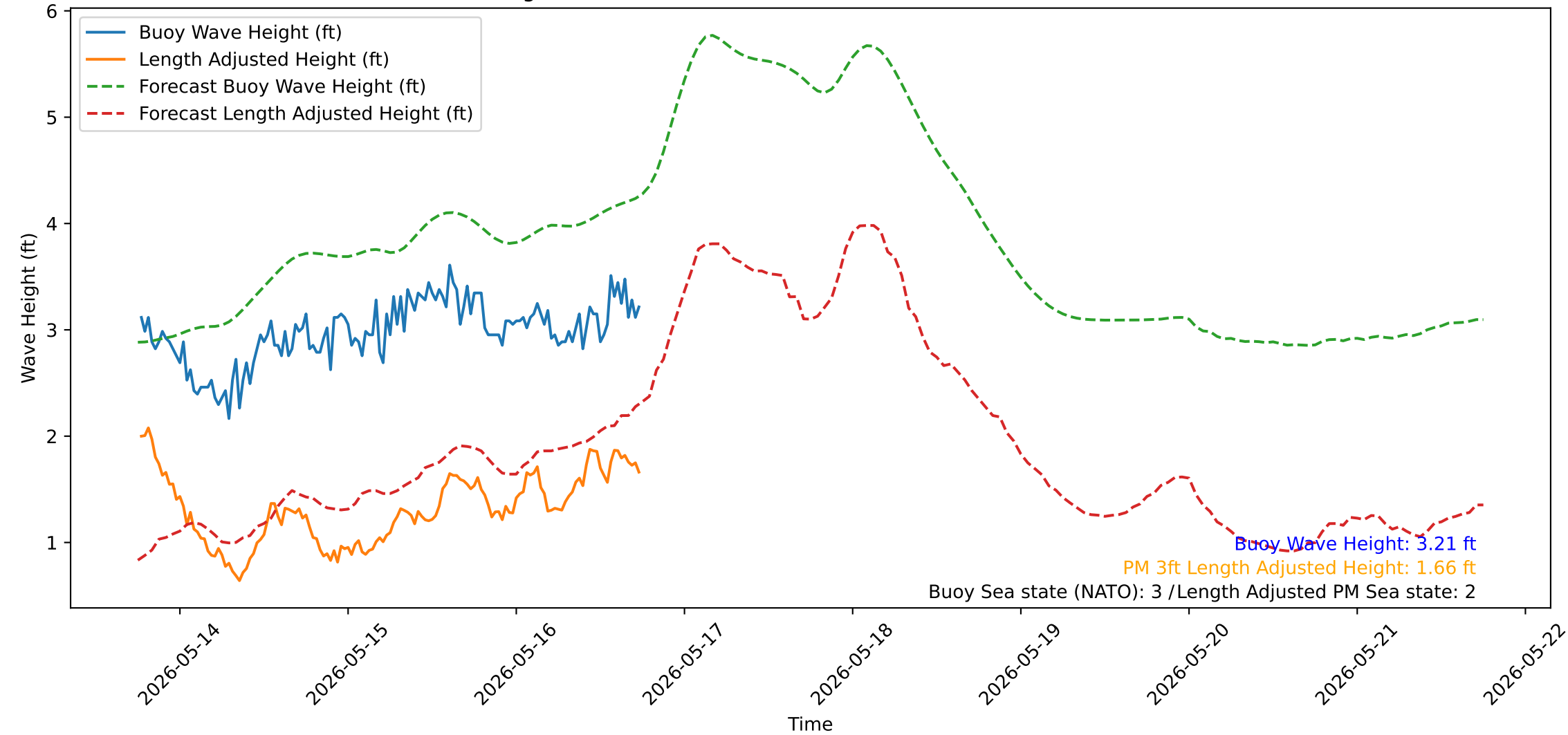
Wave Heights over Time for Oceanside Harbor at 2026-05-16 18:20:32
