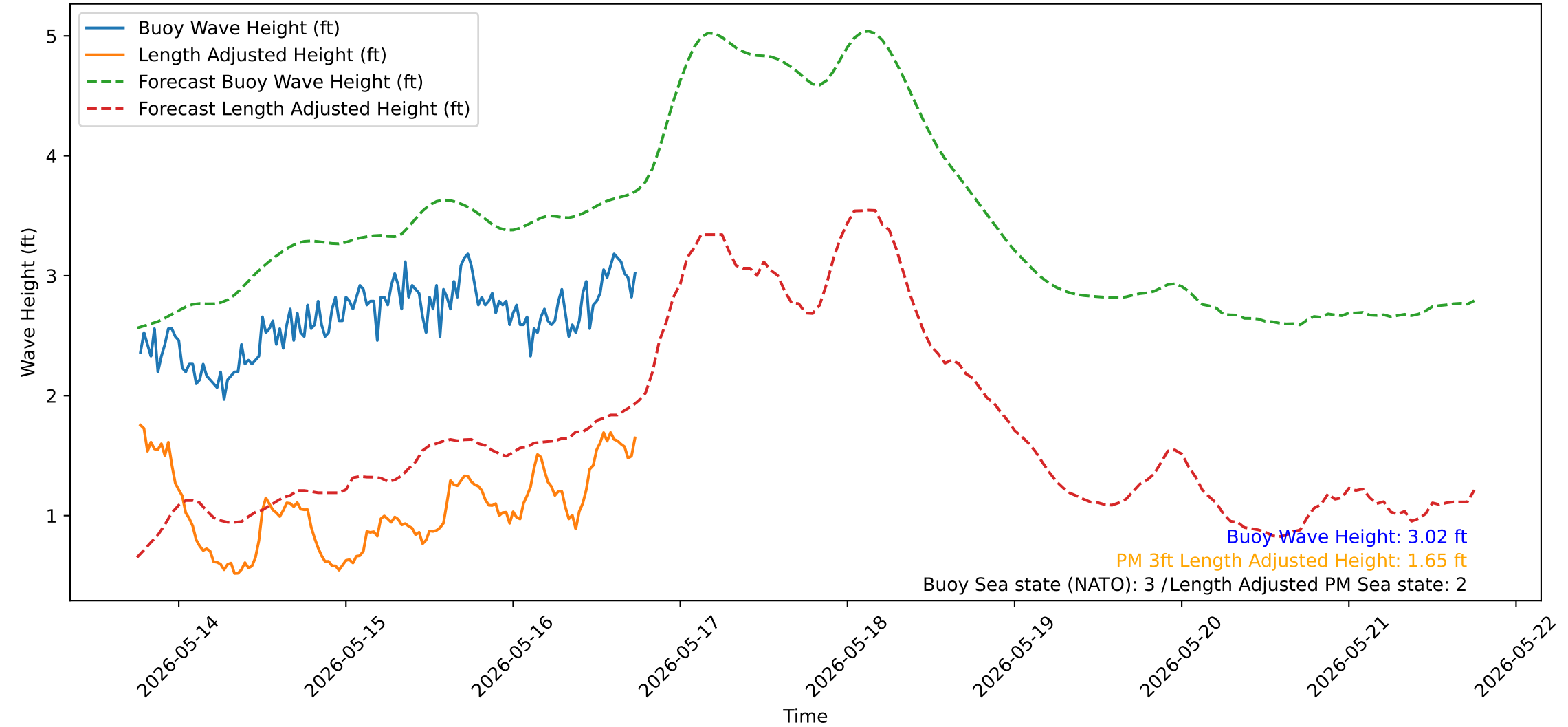
Wave Heights over Time for Red Beach at 2026-05-16 18:20:52
