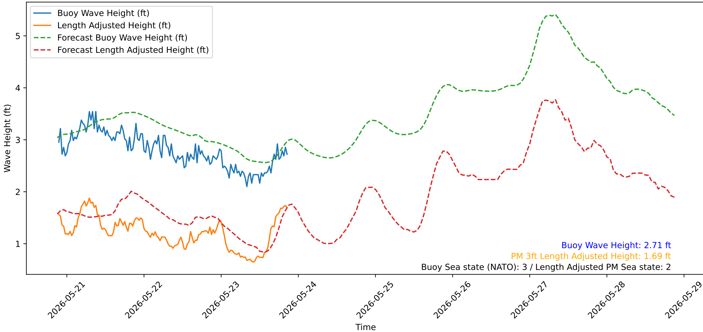
Wave Heights over Time for Green Beach at 2026-05-23 21:21:15
