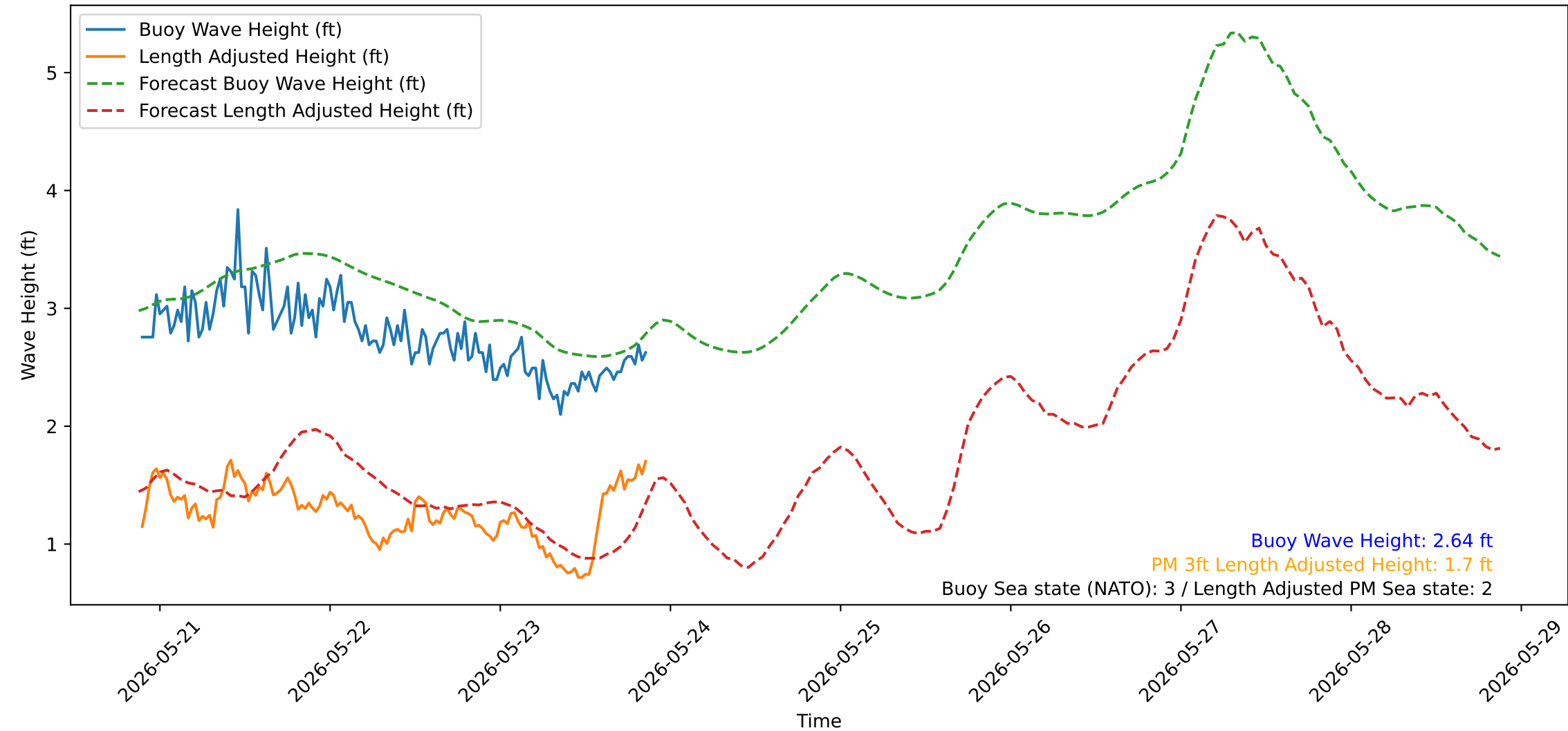
Wave Heights over Time for Oceanside Harbor at 2026-05-23 21:20:32
