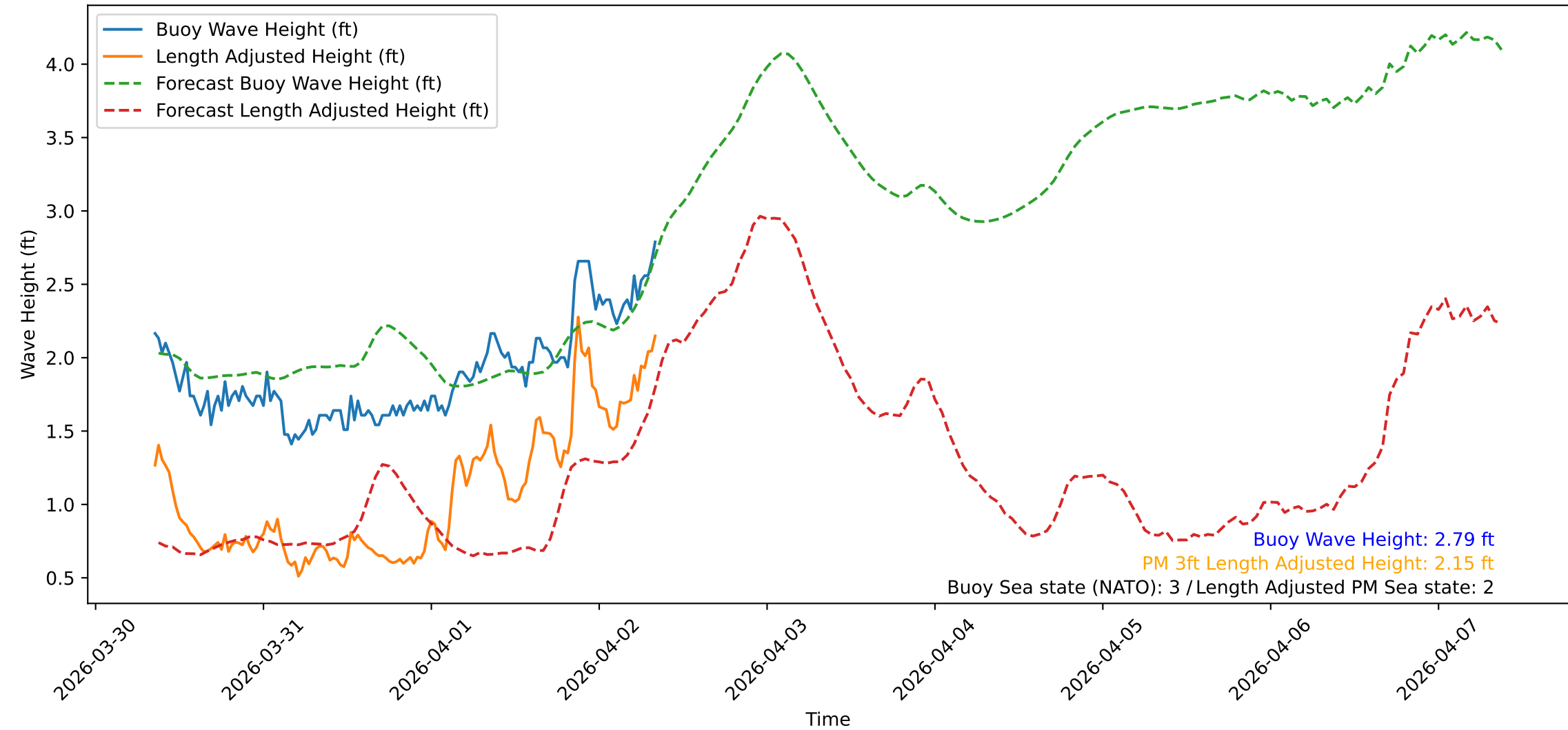
Wave Heights over Time for Green Beach at 2026-04-02 08:41:11
