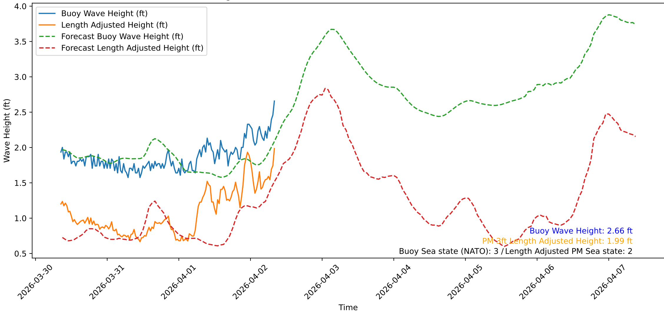
Wave Heights over Time for Oceanside Harbor at 2026-04-02 08:40:32
