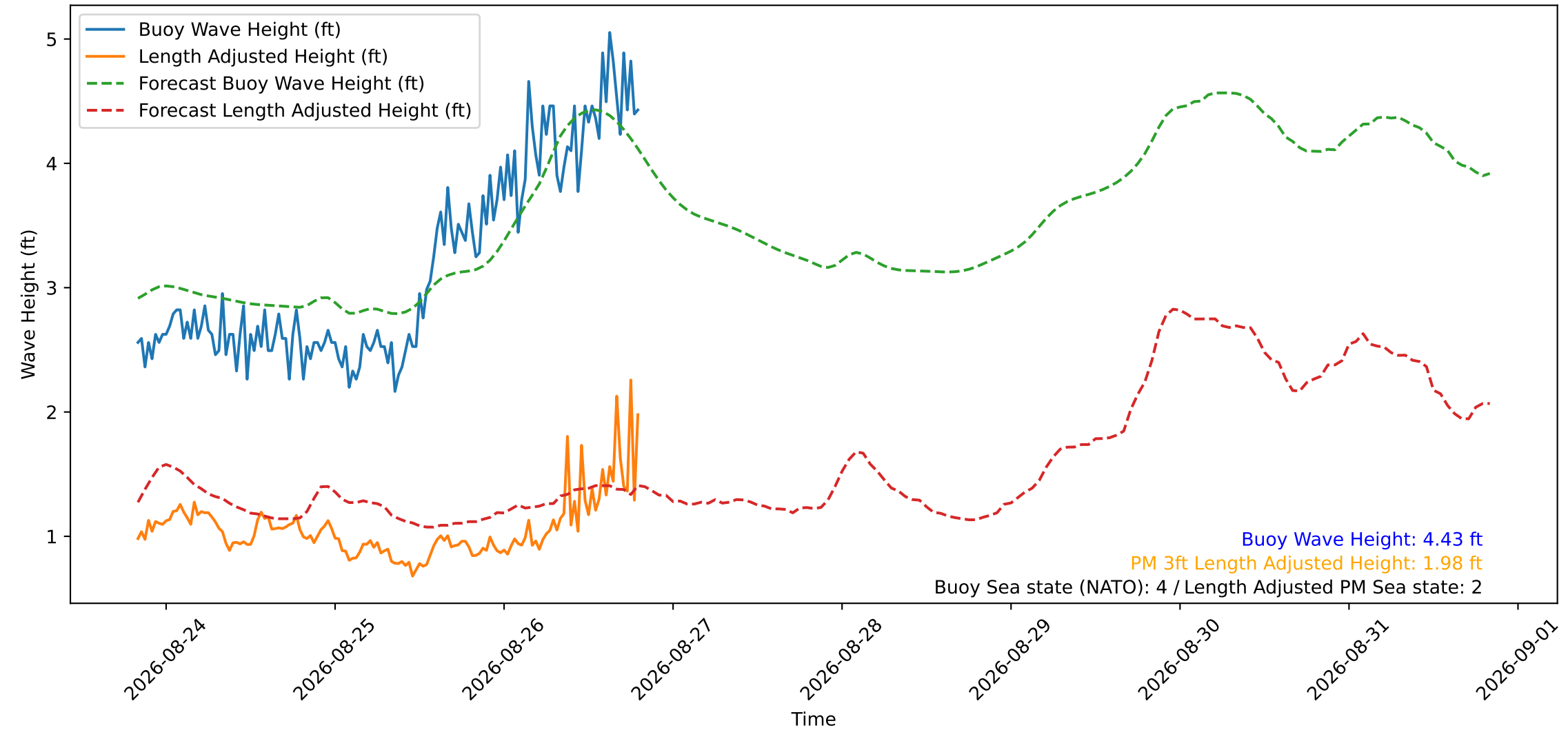
Wave Heights over Time for Red Beach at 2026-08-26 19:50:51
