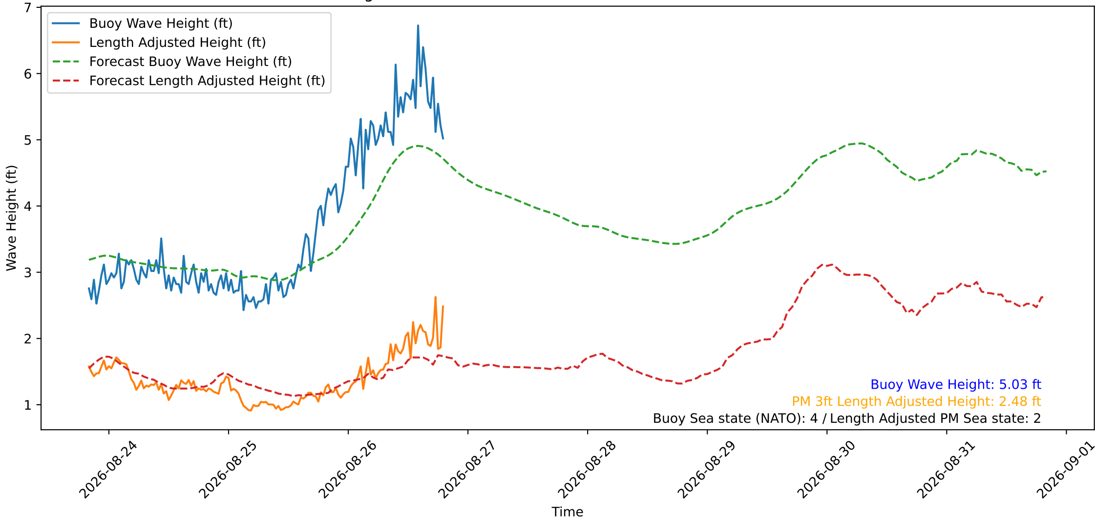
Wave Heights over Time for Oceanside Harbor at 2026-08-26 19:50:30
