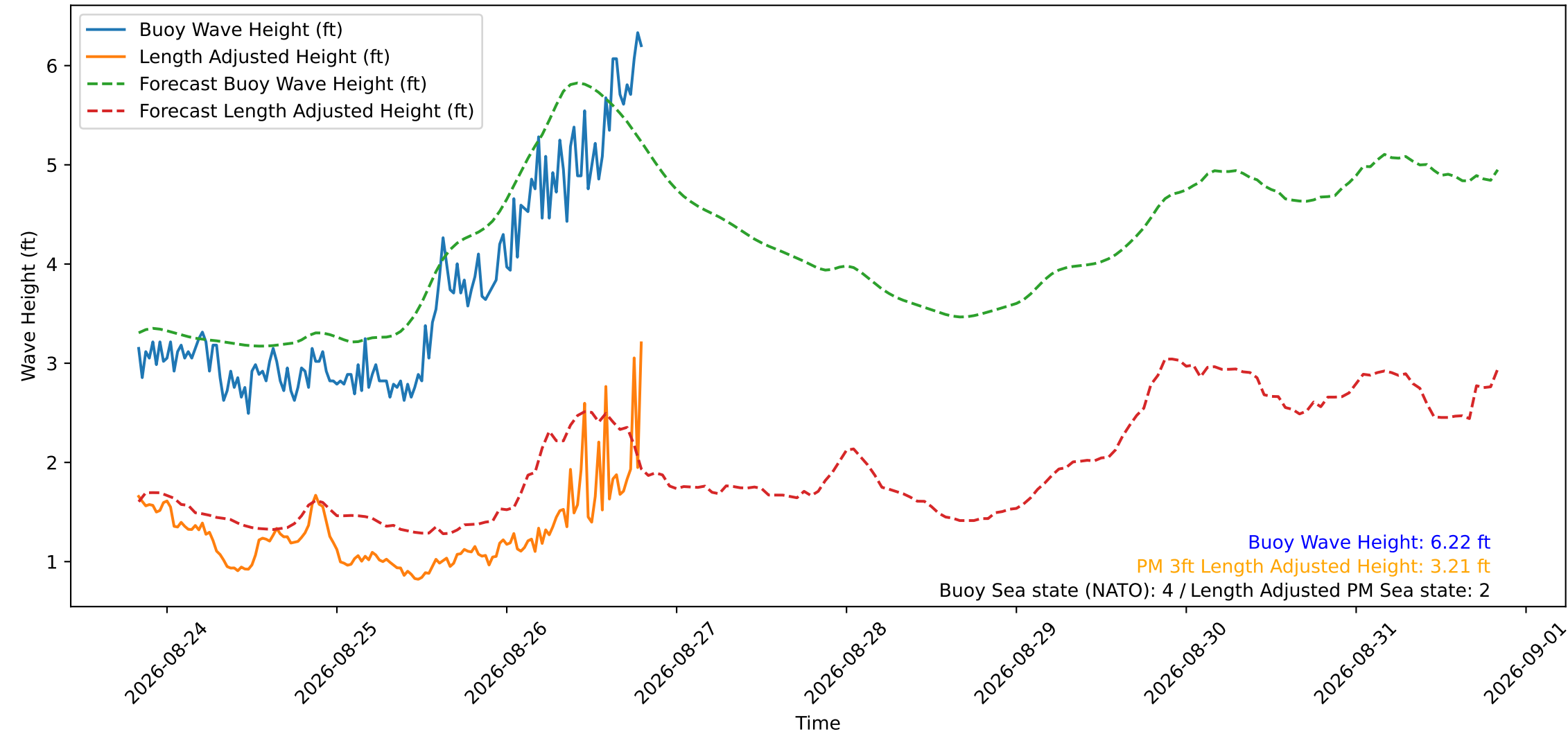
Wave Heights over Time for Green Beach at 2026-08-26 19:51:17
