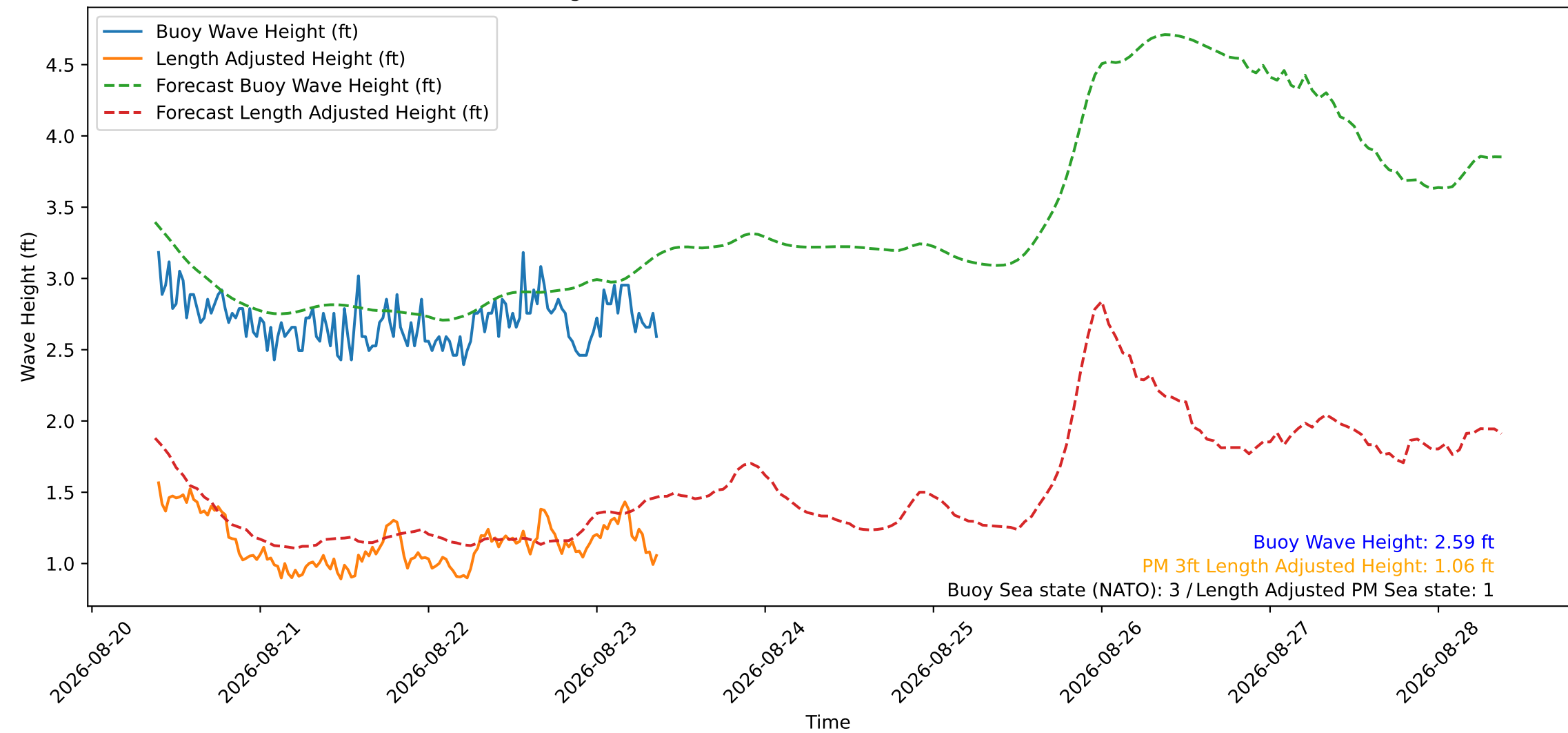
Wave Heights over Time for Green Beach at 2026-08-23 09:11:12
