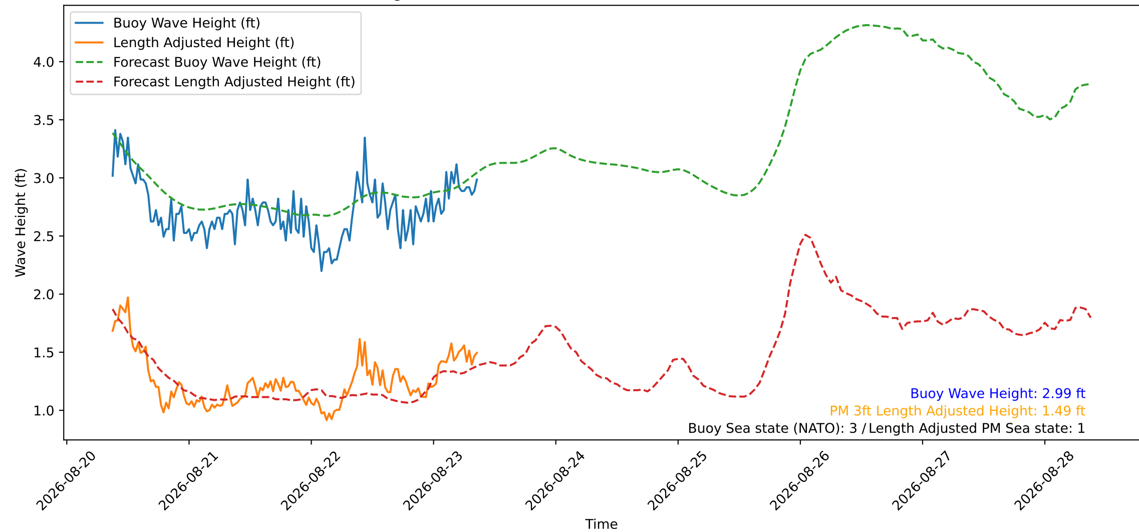
Wave Heights over Time for Oceanside Harbor at 2026-08-23 09:10:30
