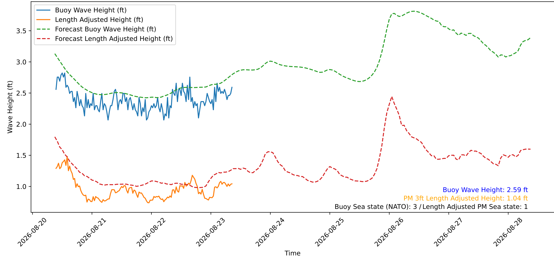
Wave Heights over Time for Red Beach at 2026-08-23 09:10:50
