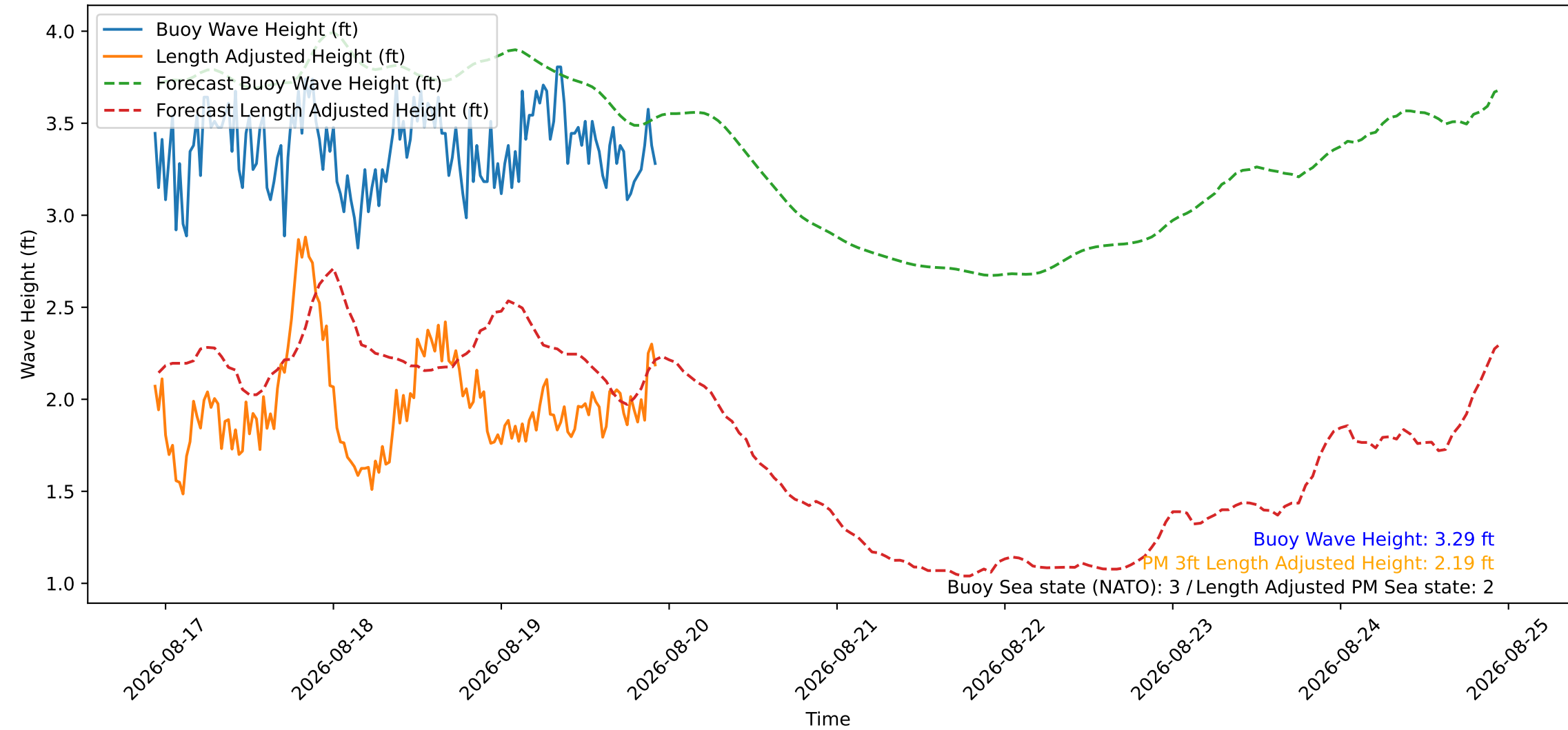
Wave Heights over Time for Oceanside Harbor at 2026-08-19 22:40:26
