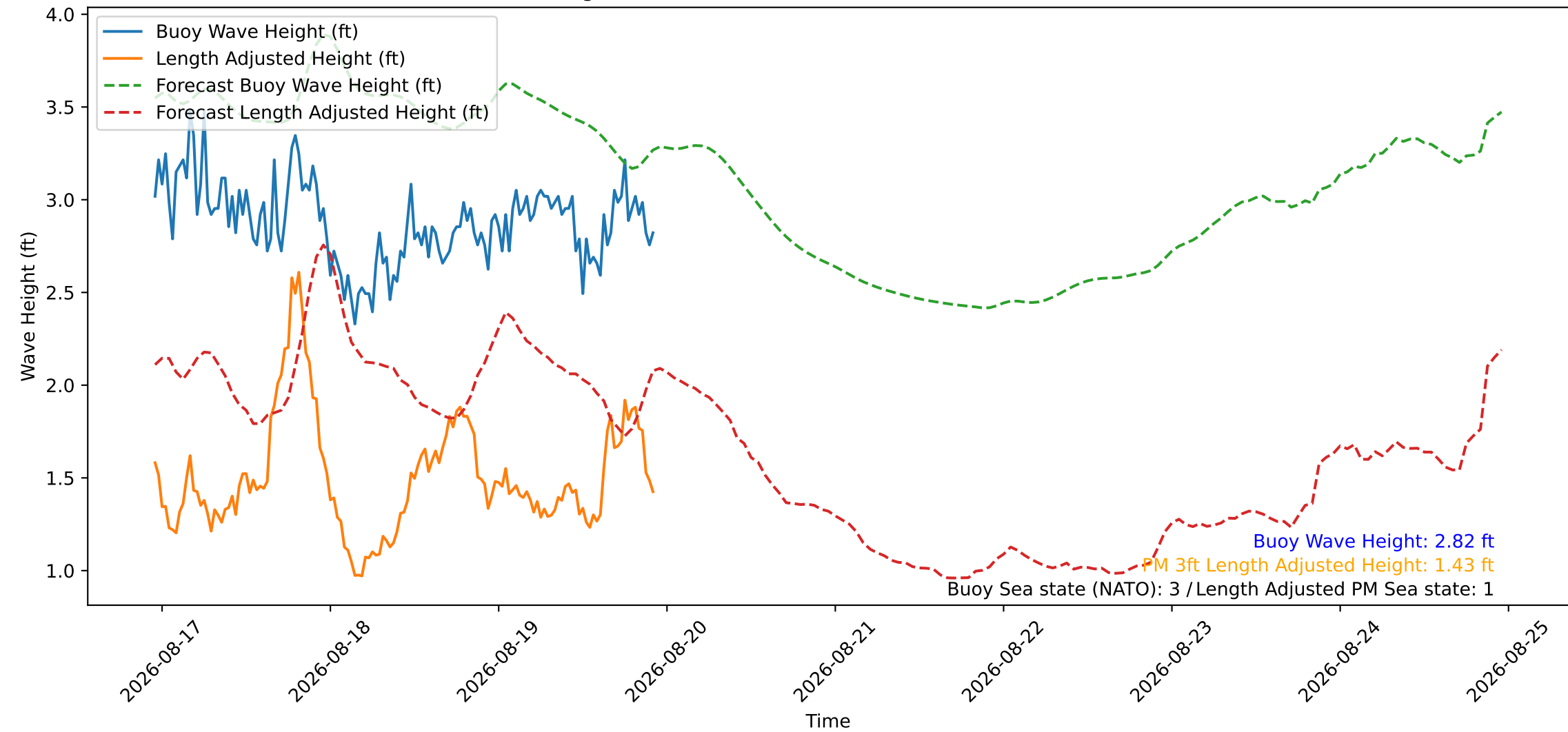
Wave Heights over Time for Red Beach at 2026-08-19 22:40:46
