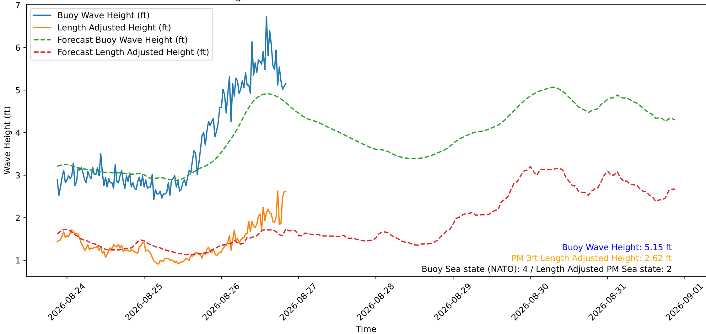
Wave Heights over Time for Oceanside Harbor at 2026-08-26 20:50:29
