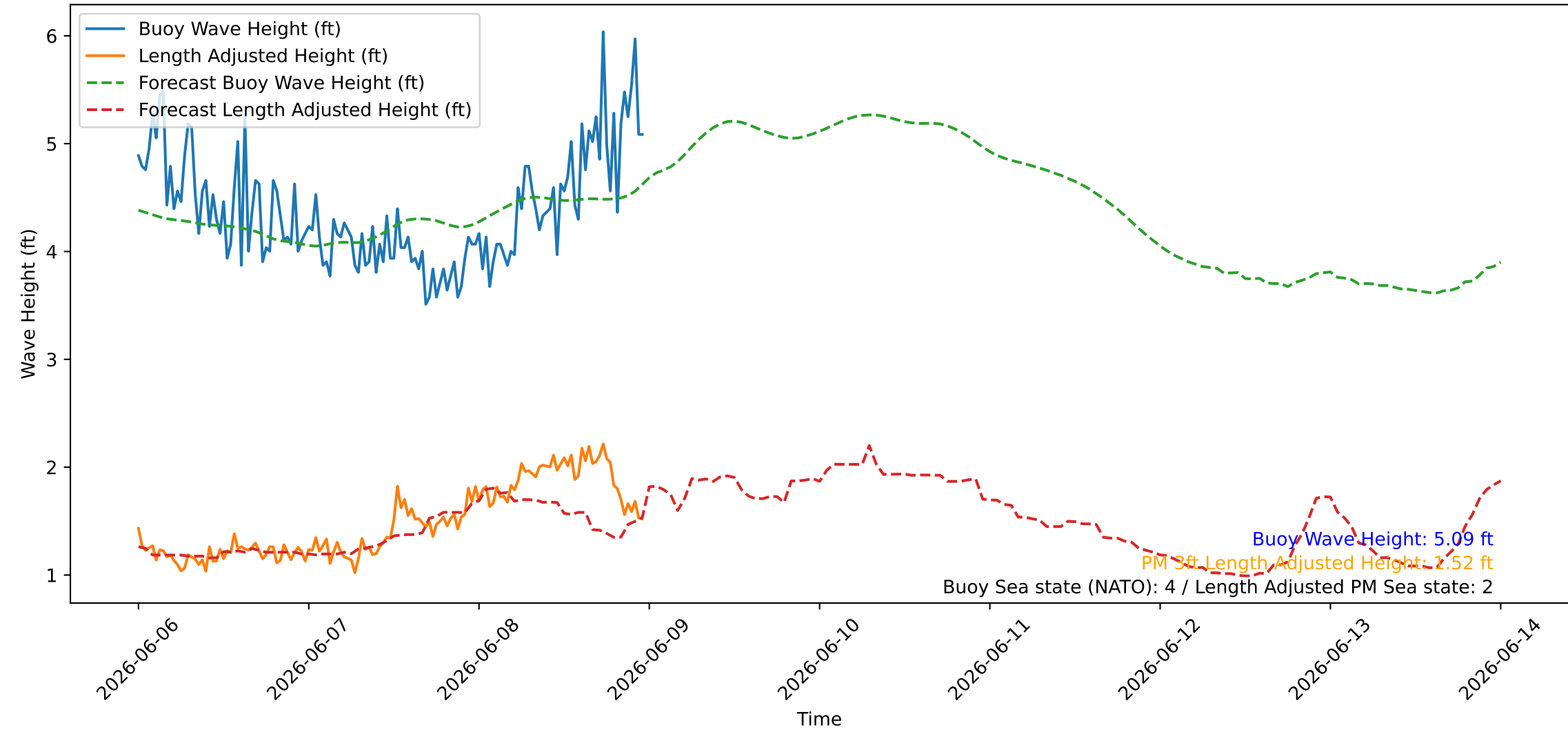
Wave Heights over Time for Oceanside Harbor at 2026-06-09 00:00:26
