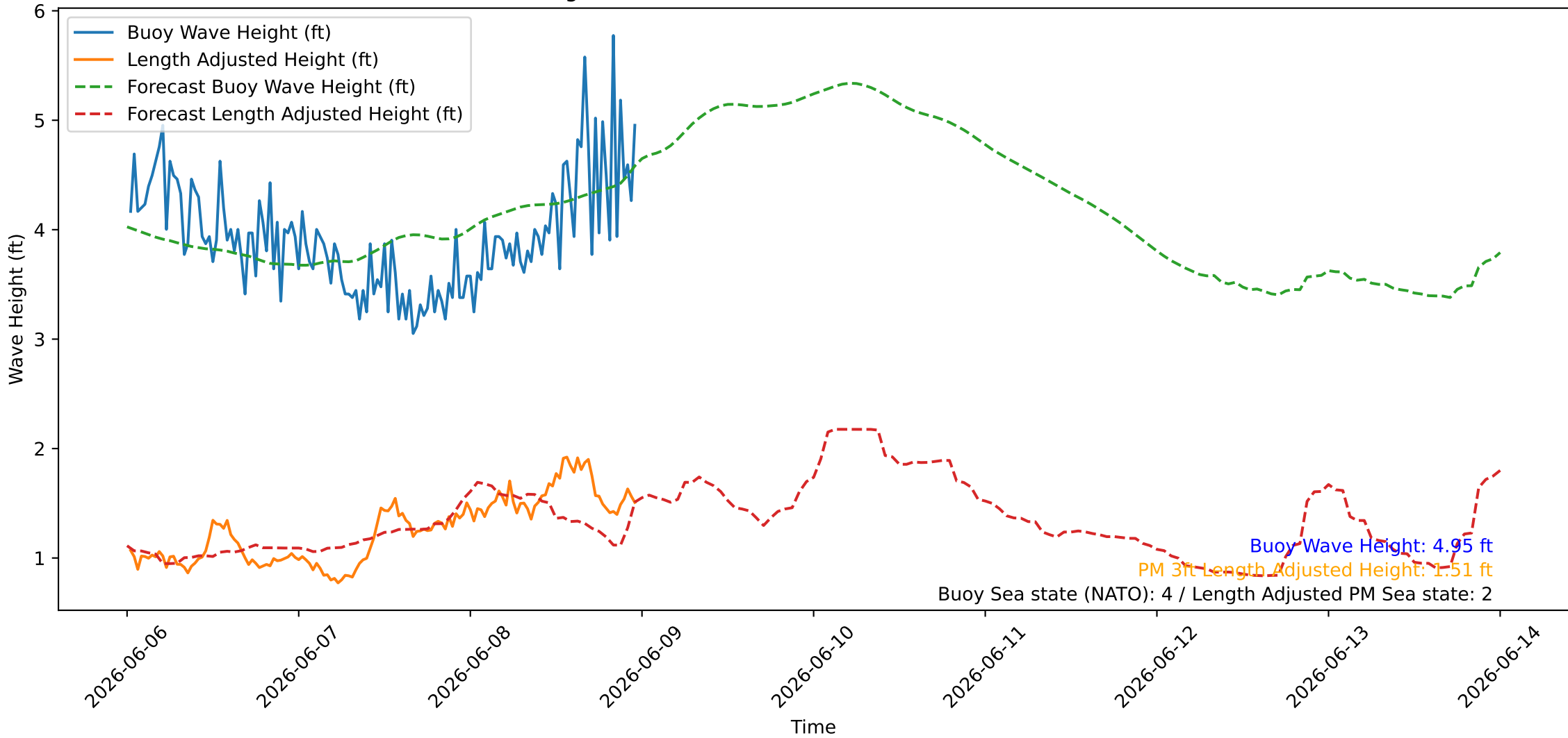
Wave Heights over Time for Red Beach at 2026-06-09 00:00:46
