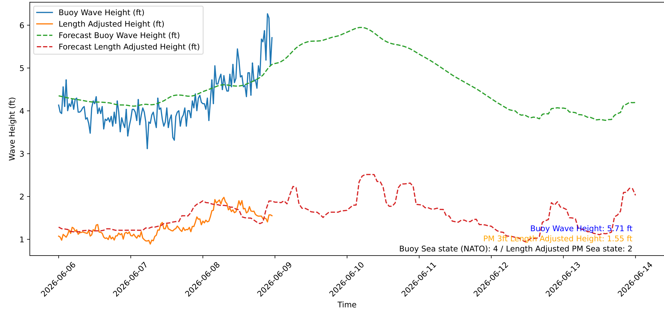
Wave Heights over Time for Green Beach at 2026-06-09 00:01:10
