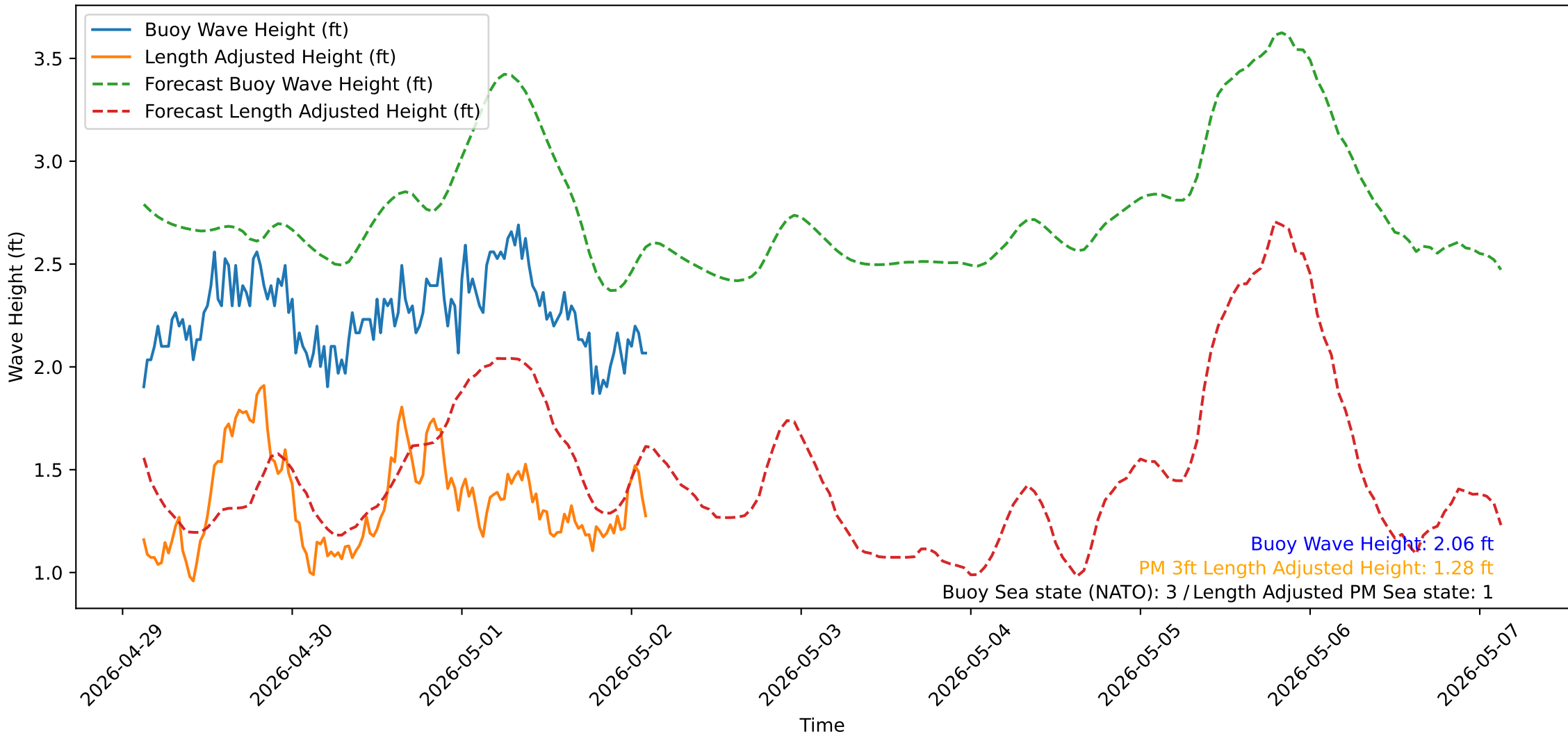
Wave Heights over Time for Oceanside Harbor at 2026-05-02 02:50:31
