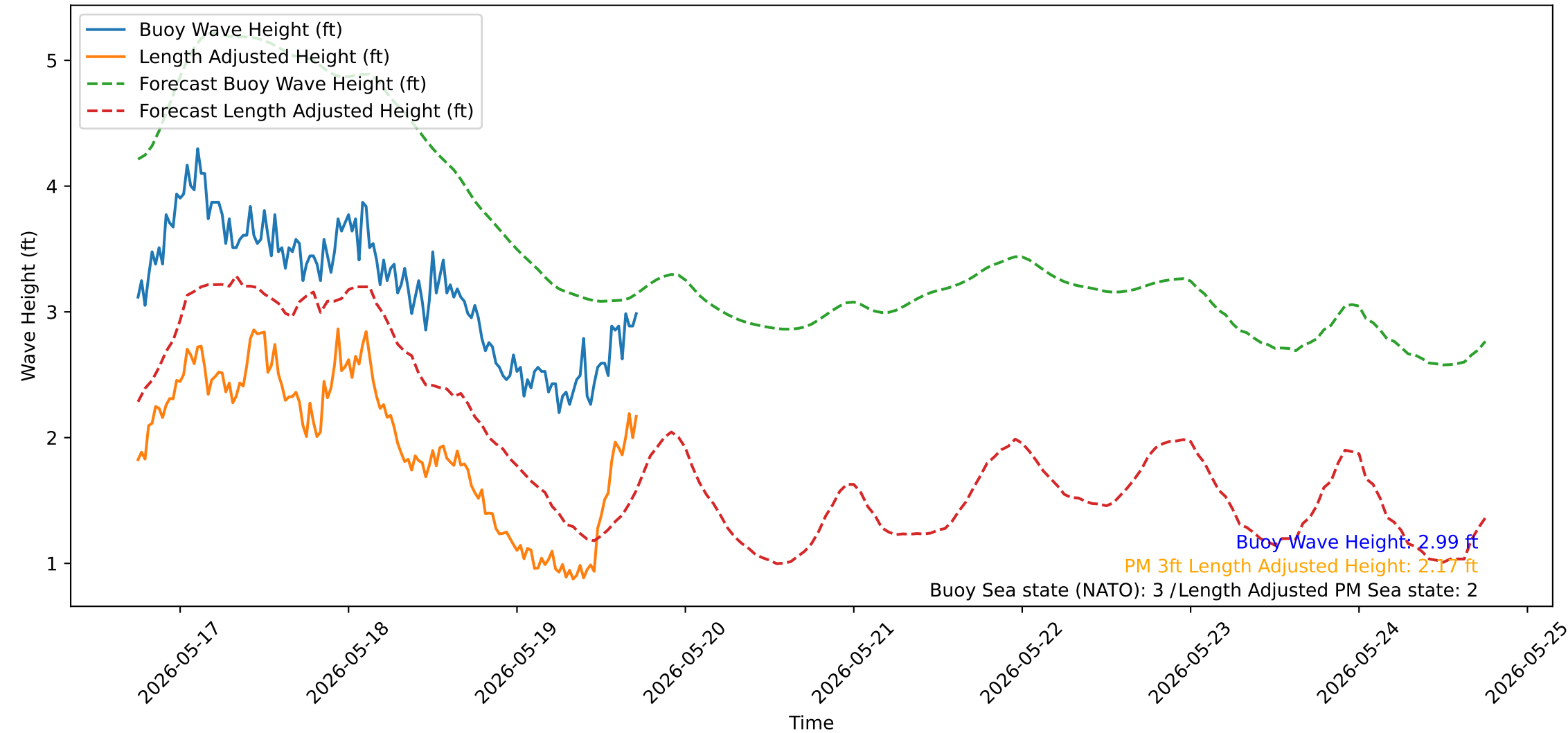
Wave Heights over Time for Oceanside Harbor at 2026-05-19 17:50:32
