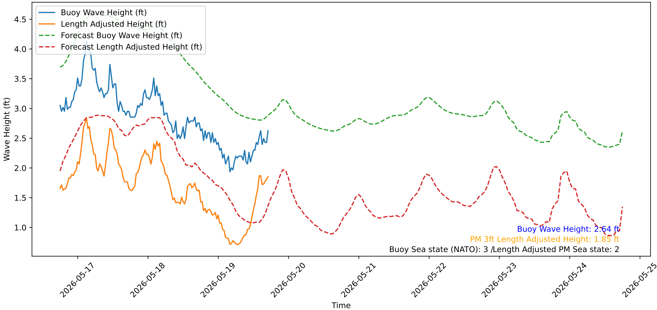
Wave Heights over Time for Red Beach at 2026-05-19 17:50:53
