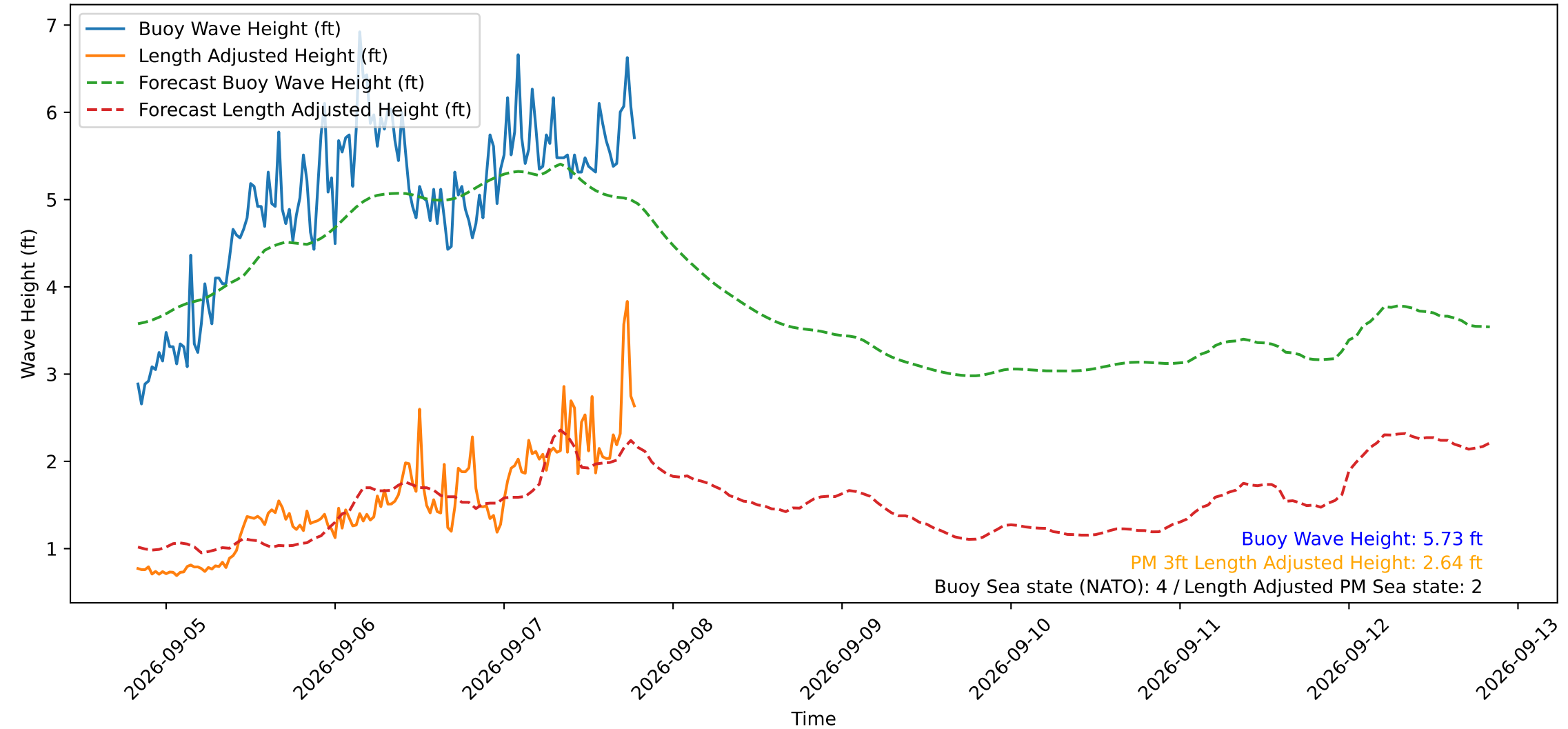
Wave Heights over Time for Red Beach at 2026-09-07 19:30:50
