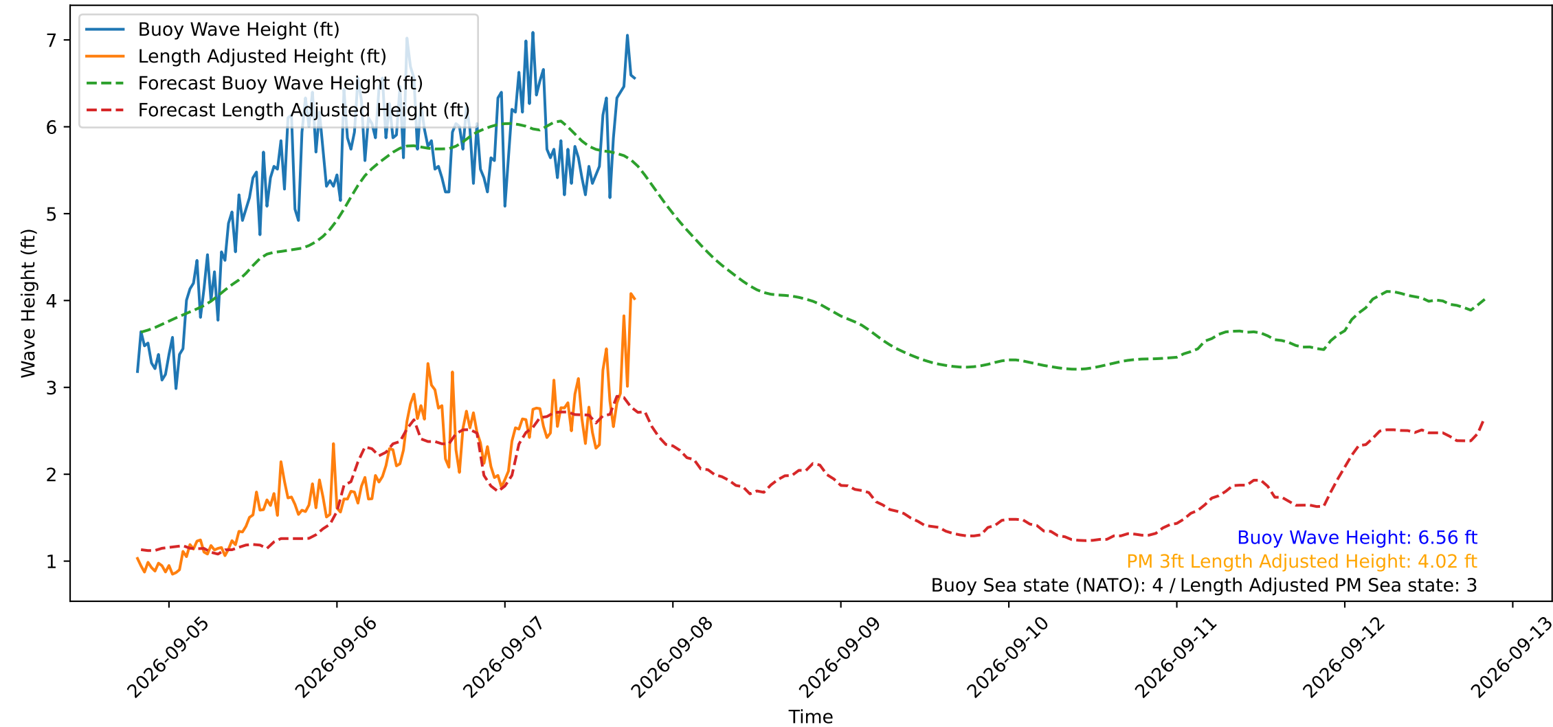
Wave Heights over Time for Oceanside Harbor at 2026-09-07 19:30:30
