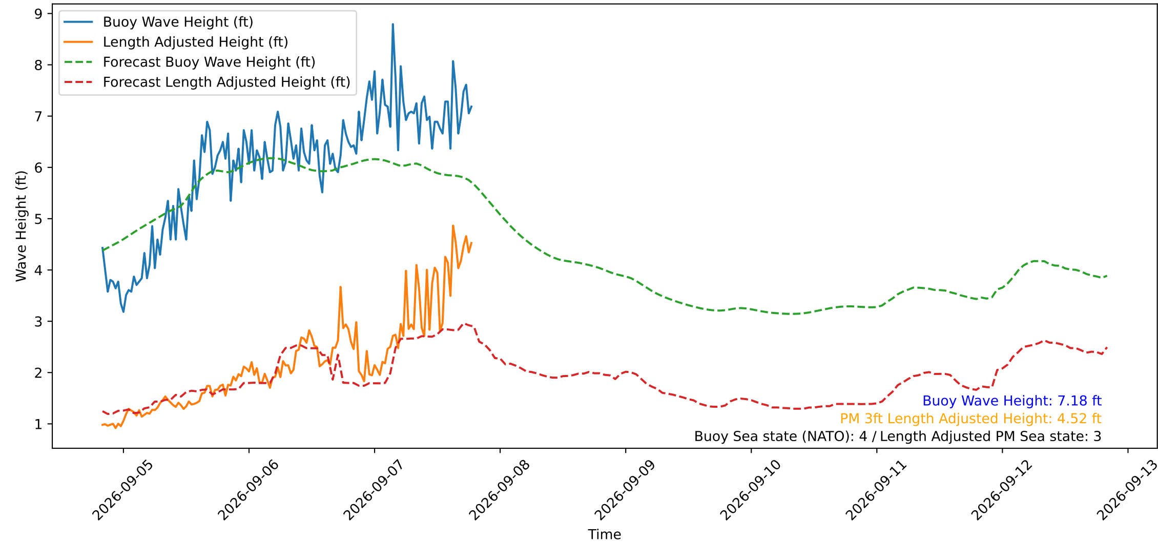
Wave Heights over Time for Green Beach at 2026-09-07 19:31:12
