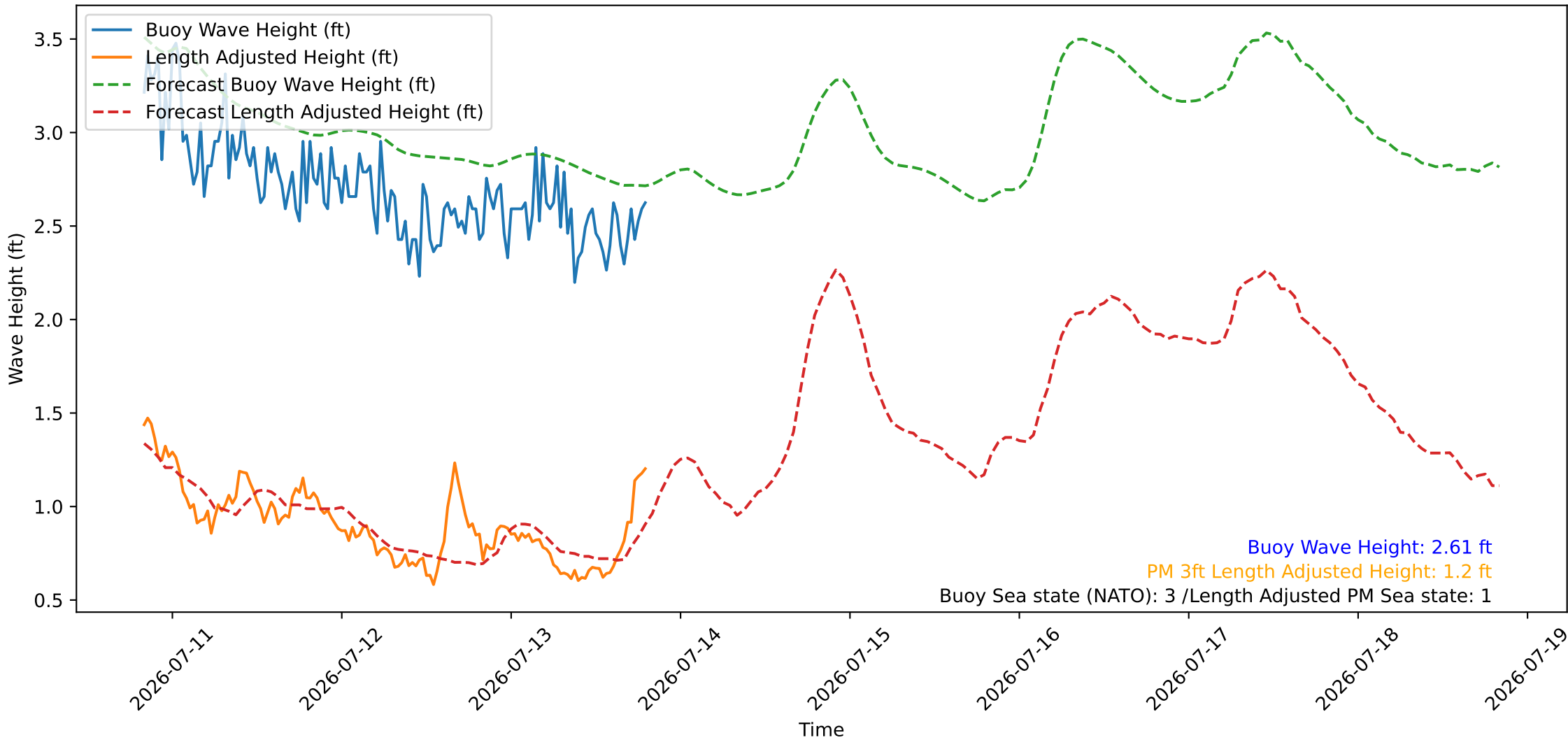
Wave Heights over Time for Green Beach at 2026-07-13 19:51:10
