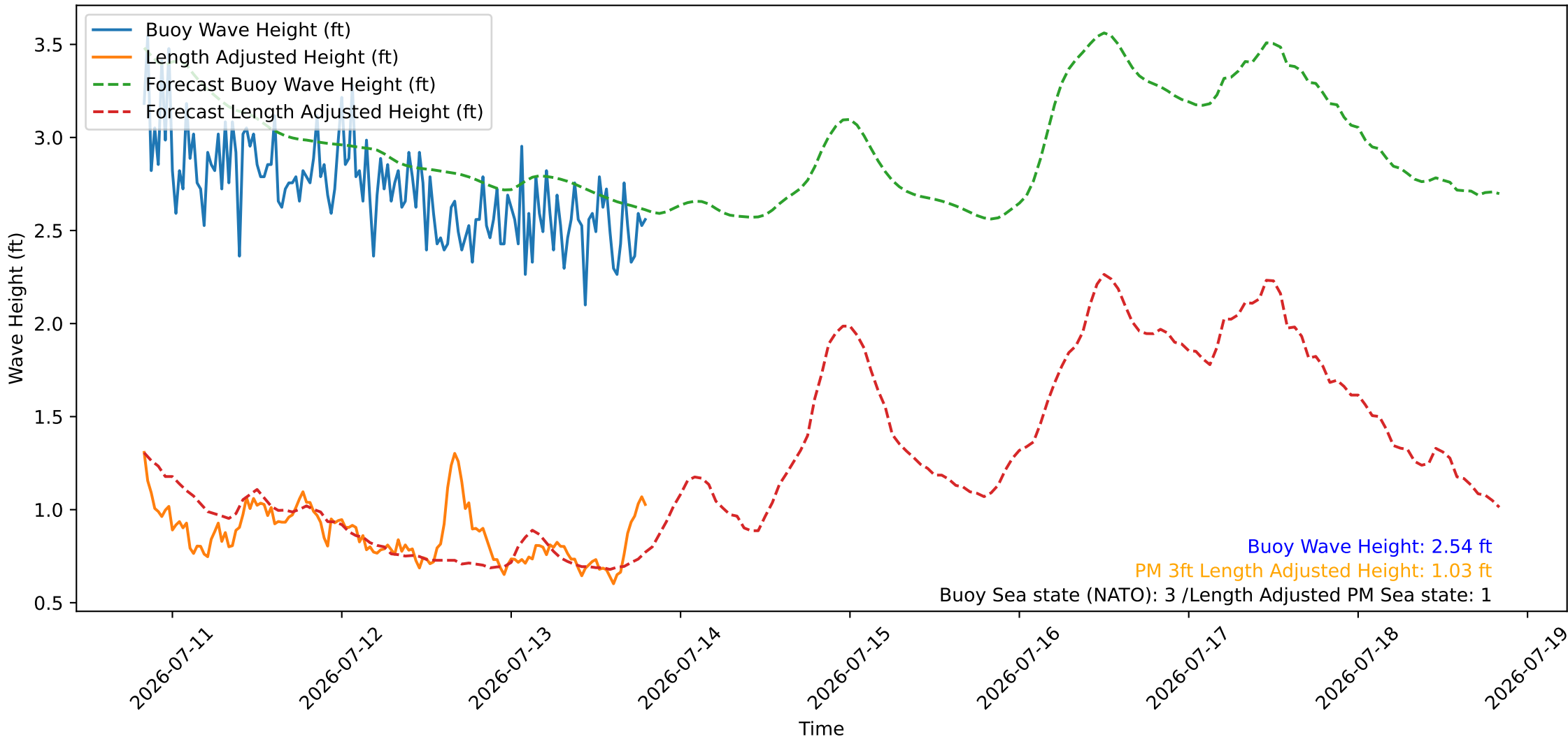
Wave Heights over Time for Oceanside Harbor at 2026-07-13 19:50:26
