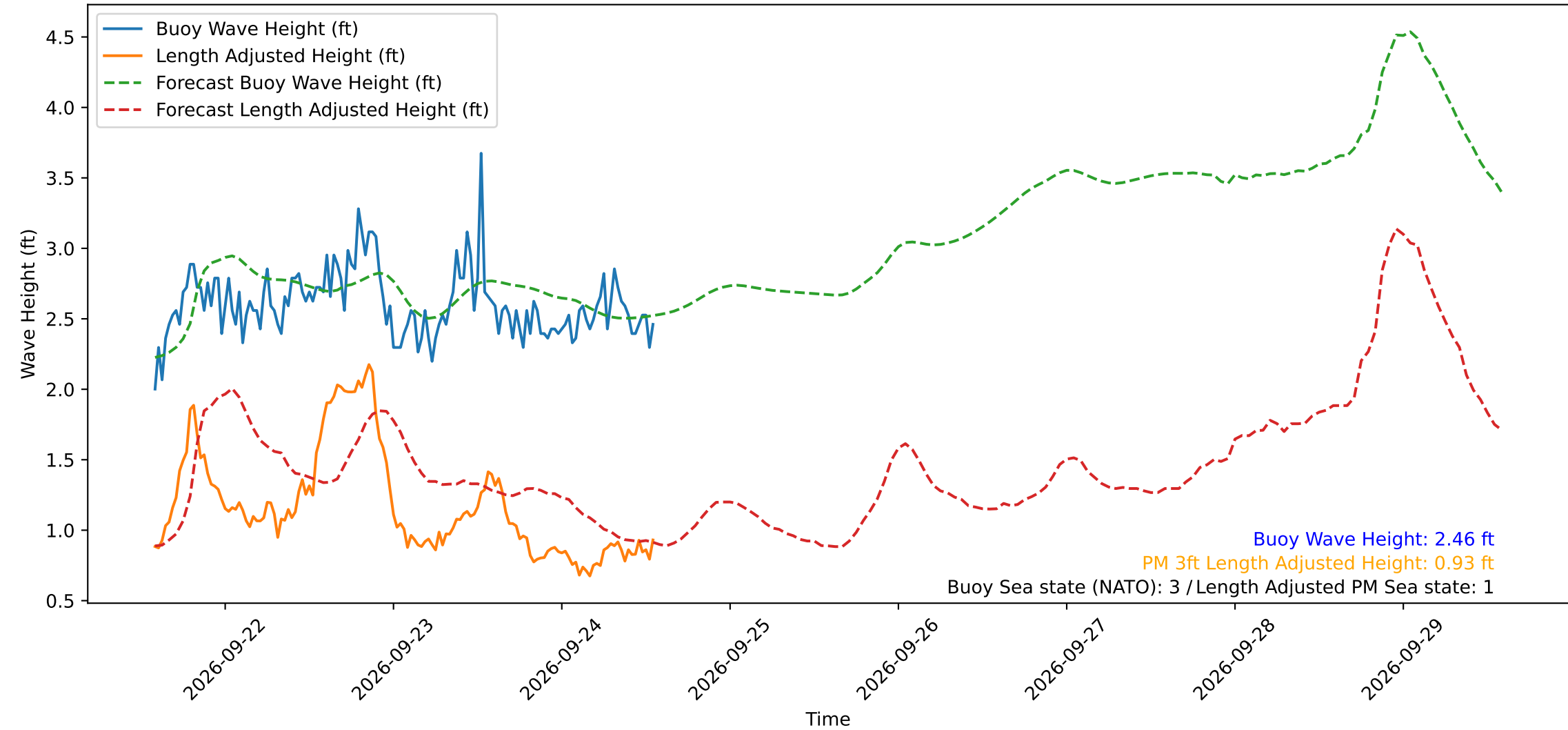
Wave Heights over Time for Red Beach at 2026-09-24 13:40:52
