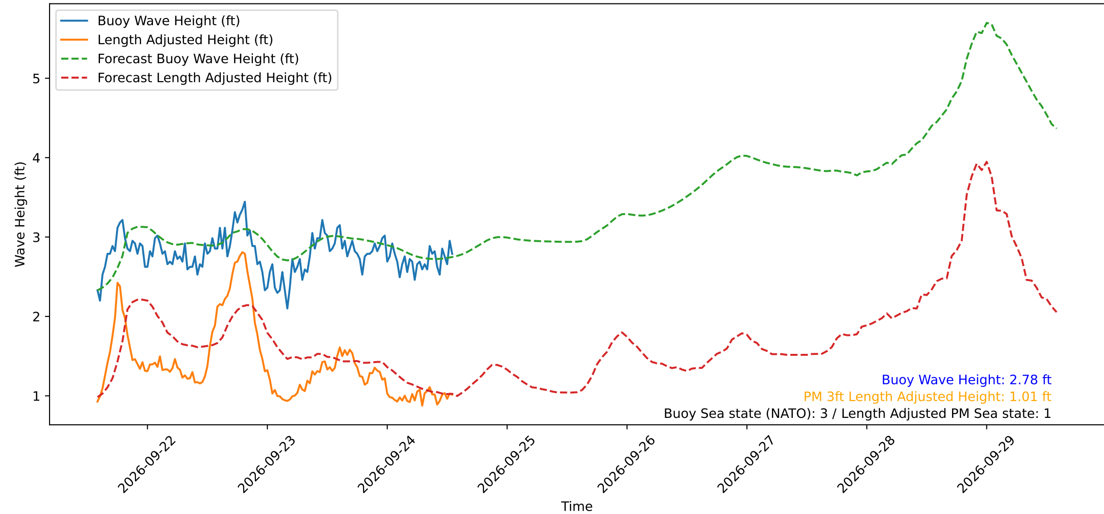
Wave Heights over Time for Green Beach at 2026-09-24 13:41:17
