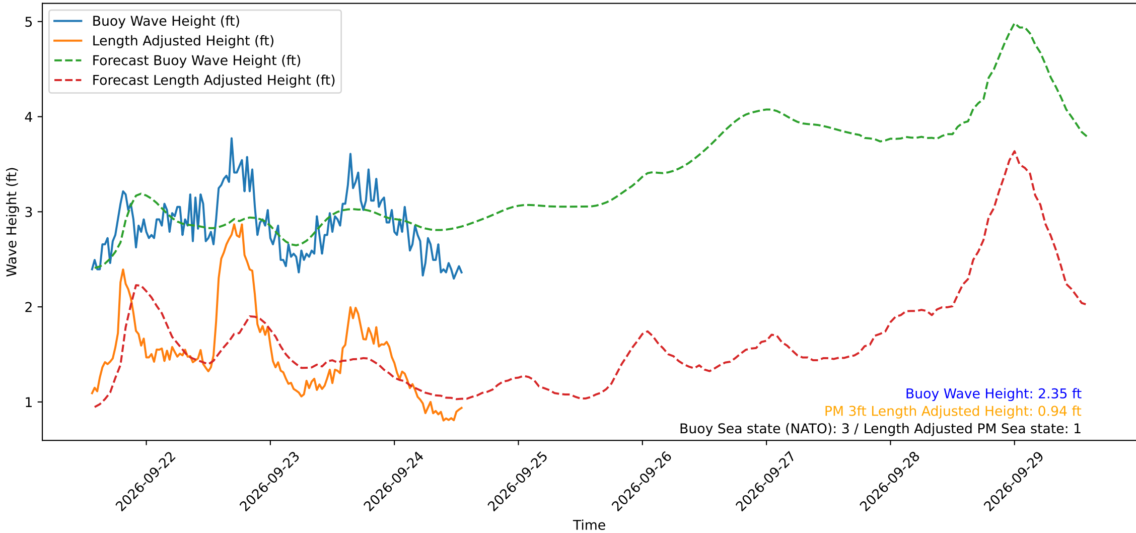
Wave Heights over Time for Oceanside Harbor at 2026-09-24 13:40:31
