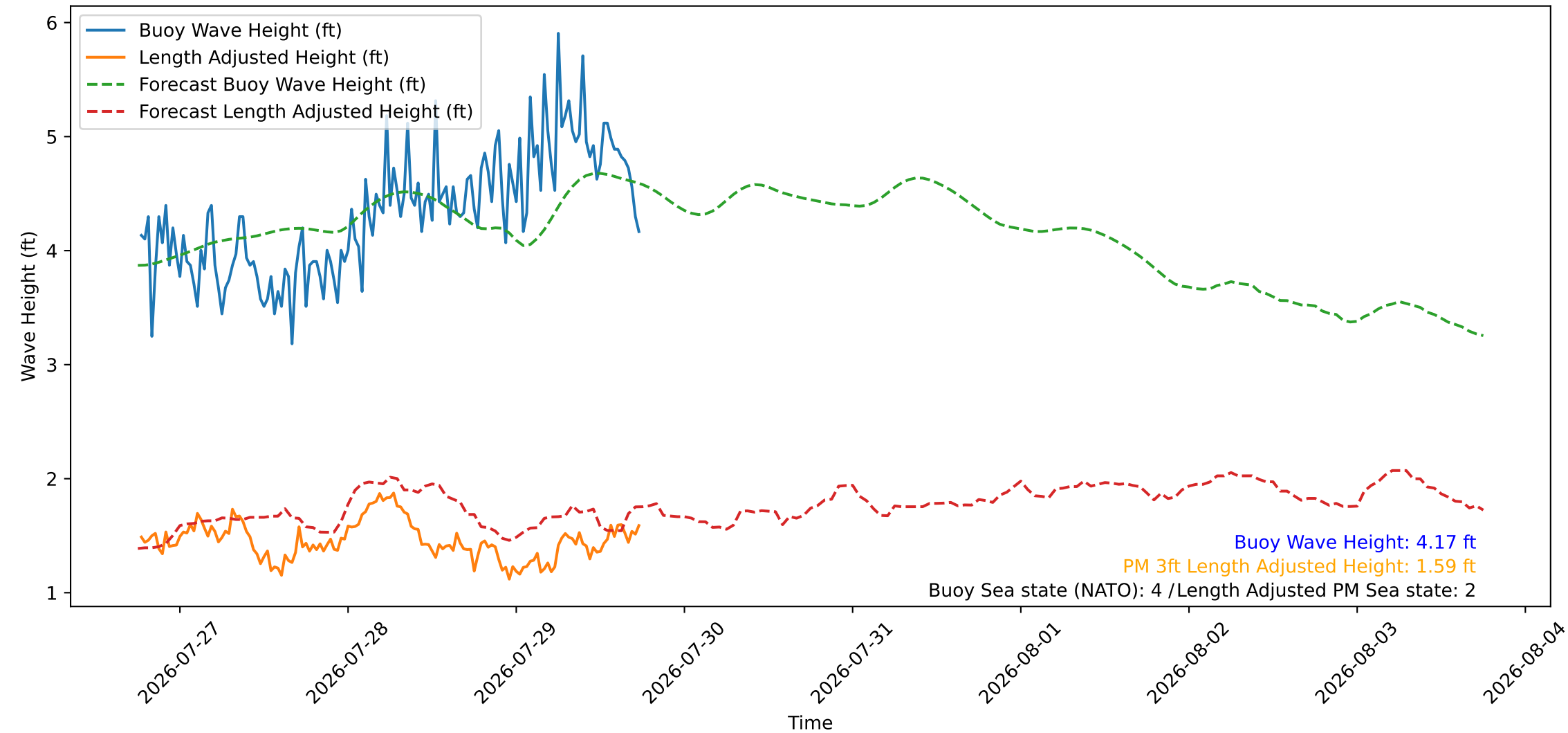
Wave Heights over Time for Oceanside Harbor at 2026-07-29 18:20:26
