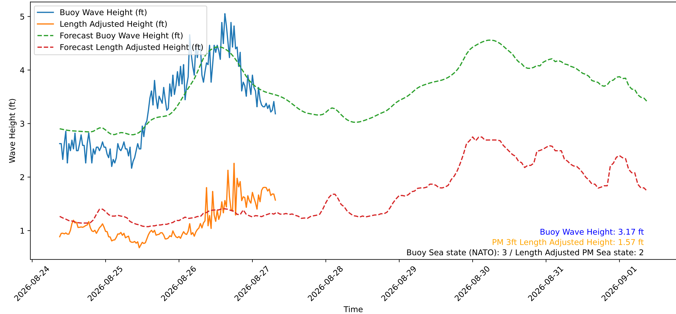
Wave Heights over Time for Red Beach at 2026-08-27 08:30:49
