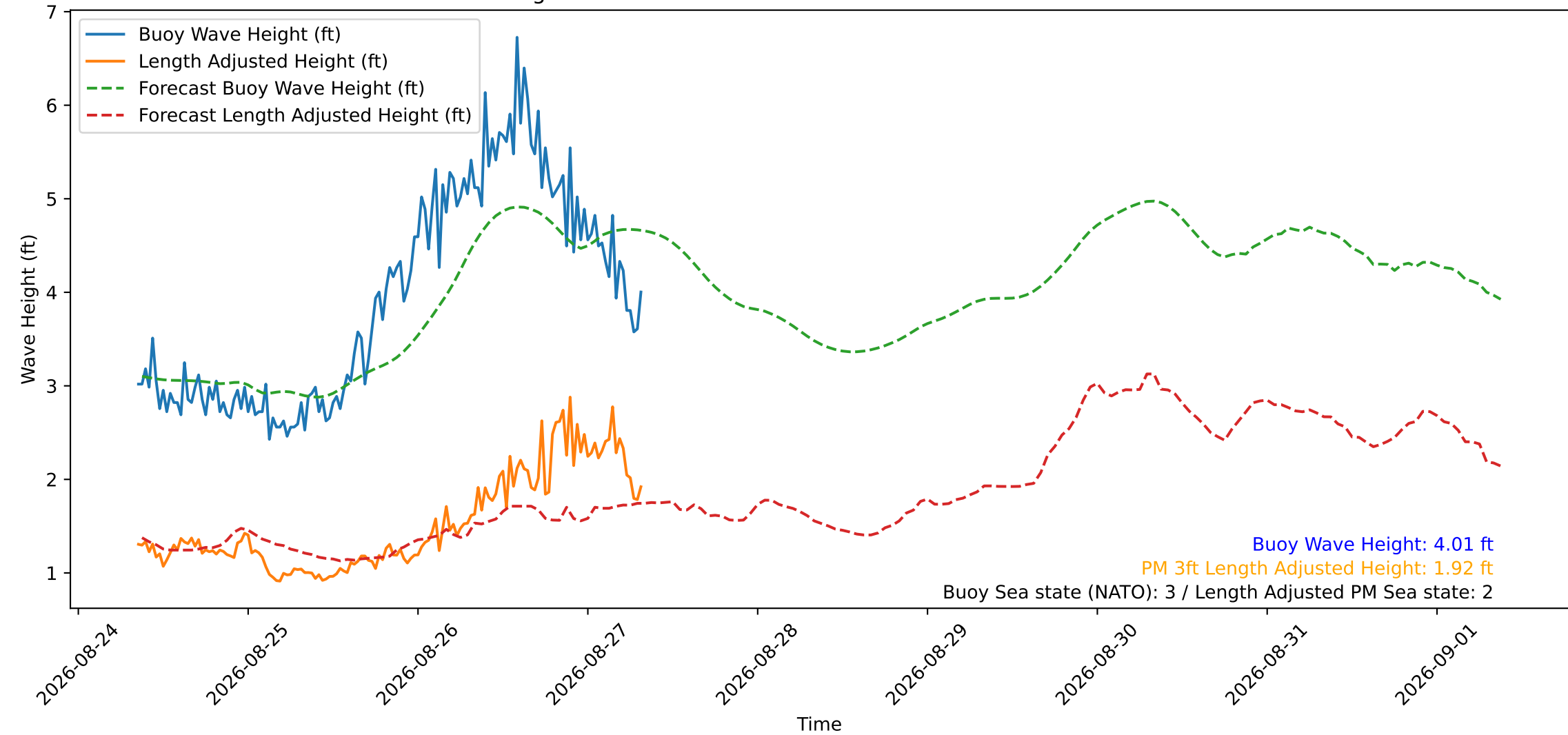
Wave Heights over Time for Oceanside Harbor at 2026-08-27 08:30:29
