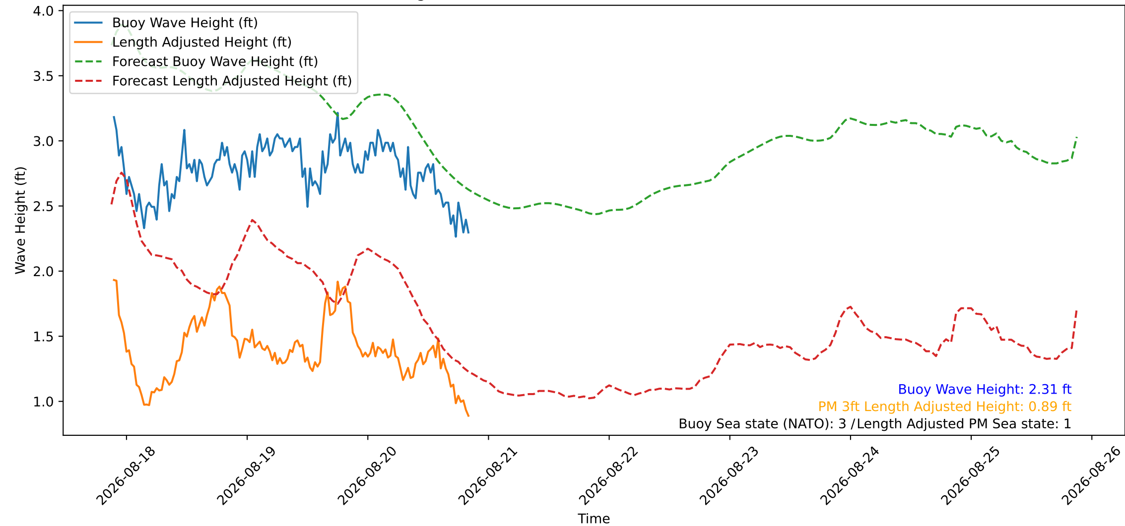
Wave Heights over Time for Red Beach at 2026-08-20 21:10:46
