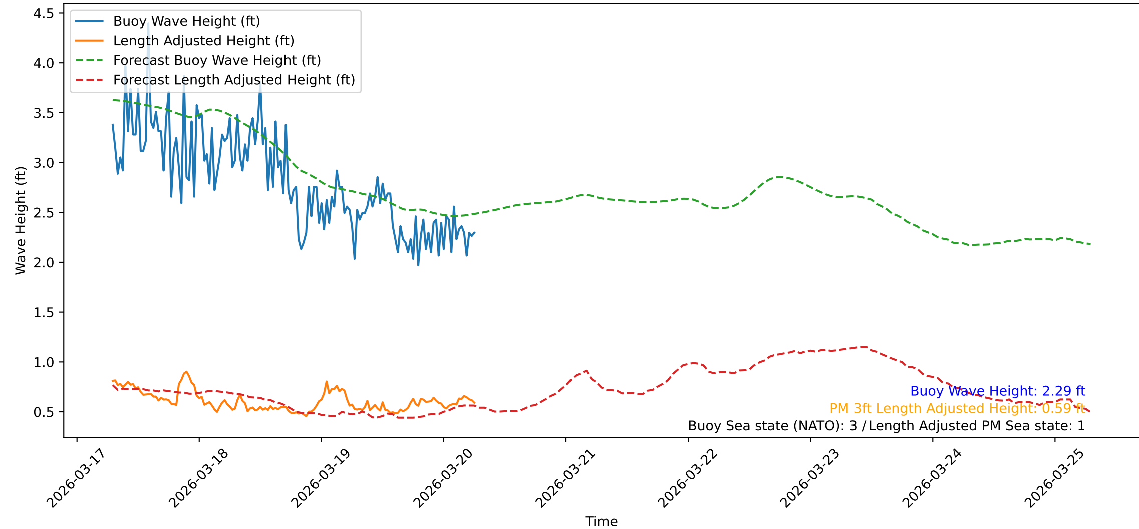
Wave Heights over Time for Oceanside Harbor at 2026-03-20 06:50:31
