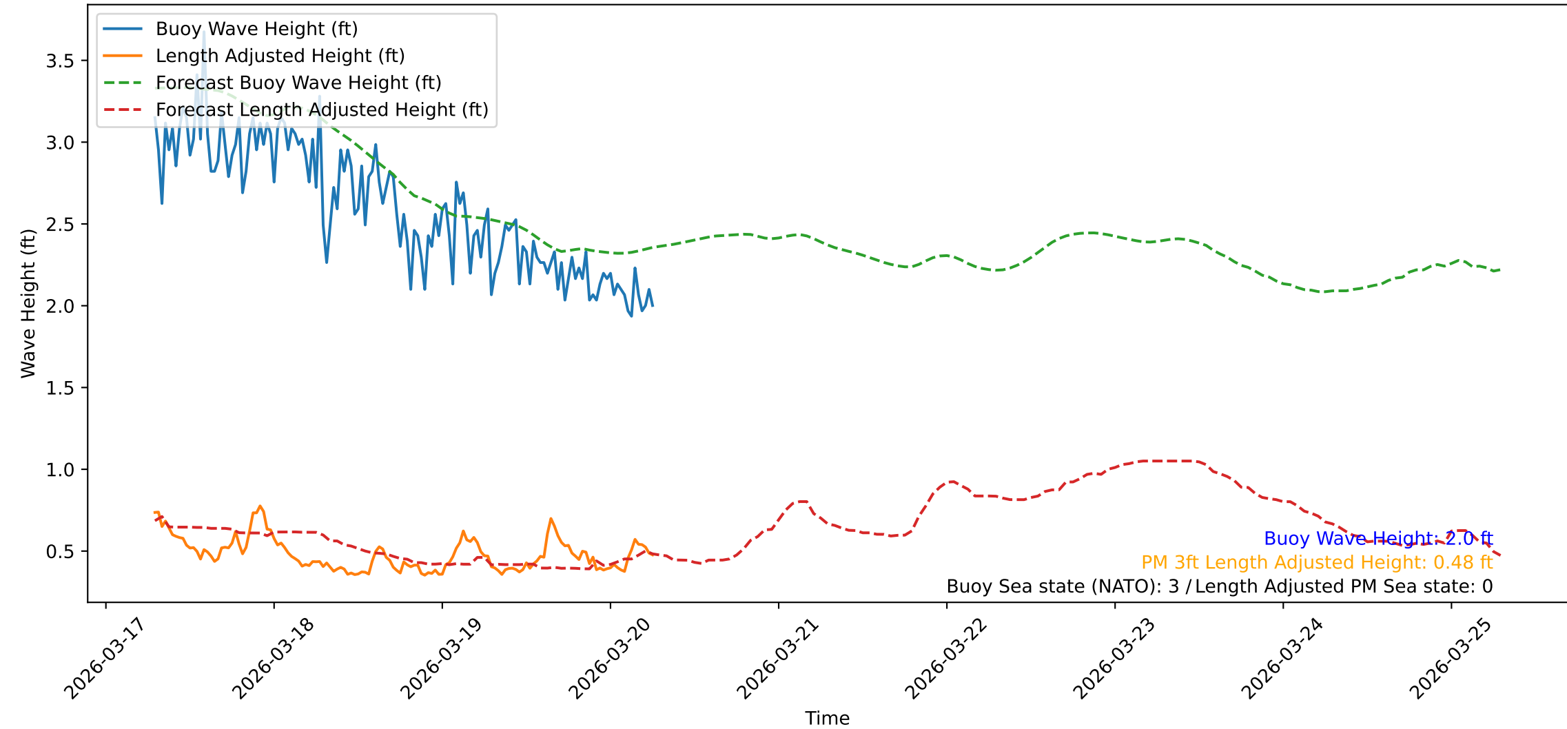
Wave Heights over Time for Red Beach at 2026-03-20 06:50:47
