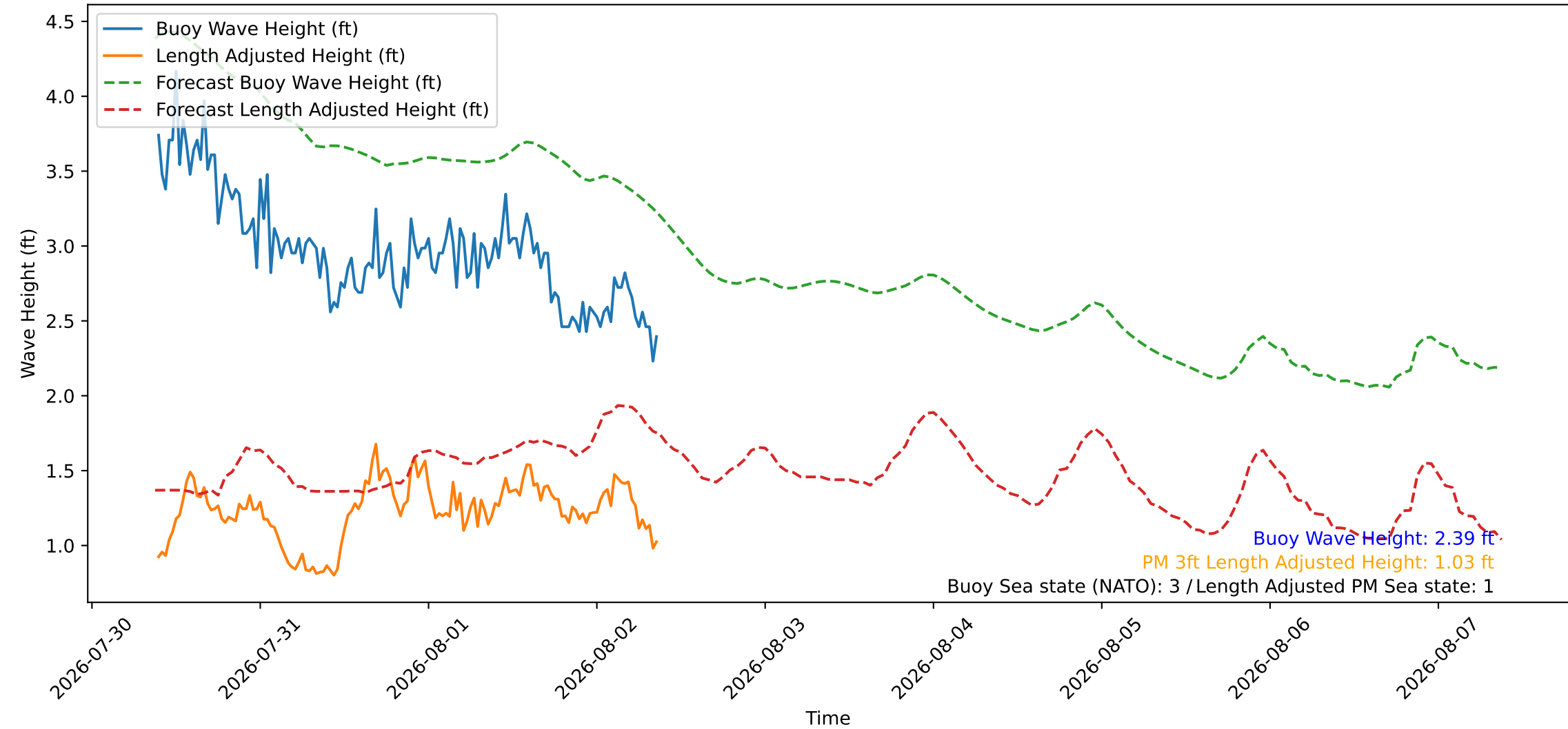
Wave Heights over Time for Red Beach at 2026-08-02 09:20:47
