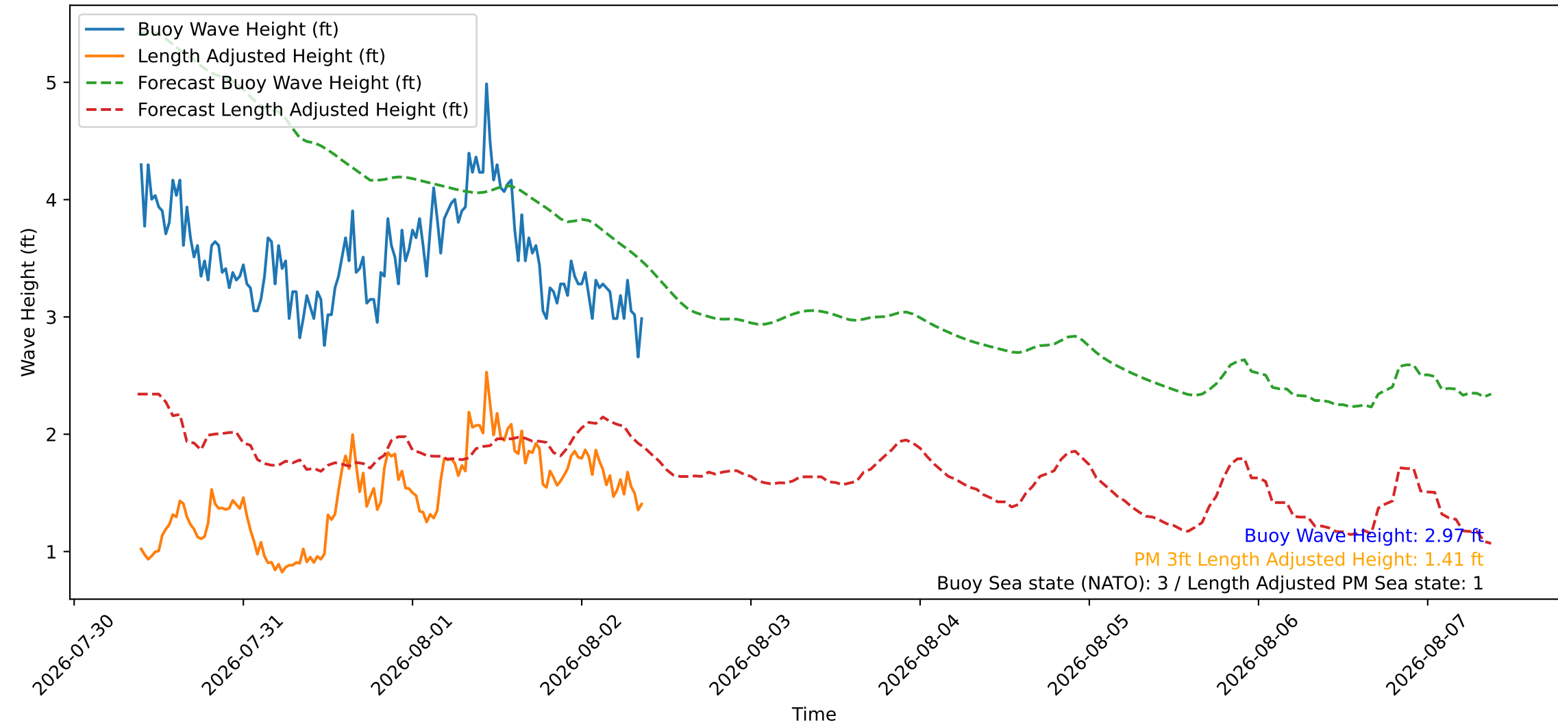
Wave Heights over Time for Green Beach at 2026-08-02 09:21:10
