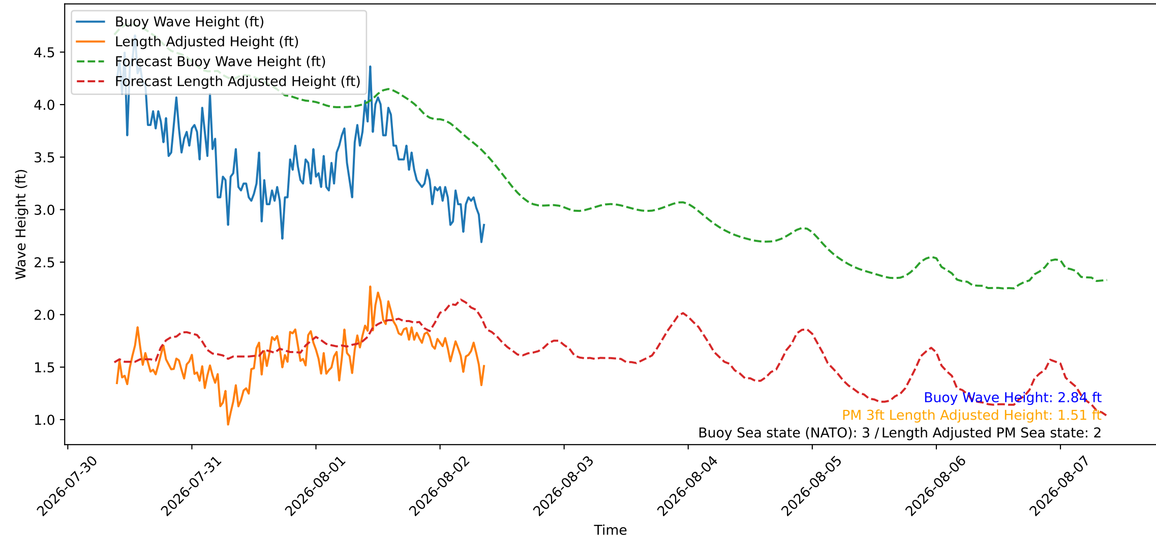
Wave Heights over Time for Oceanside Harbor at 2026-08-02 09:20:26
