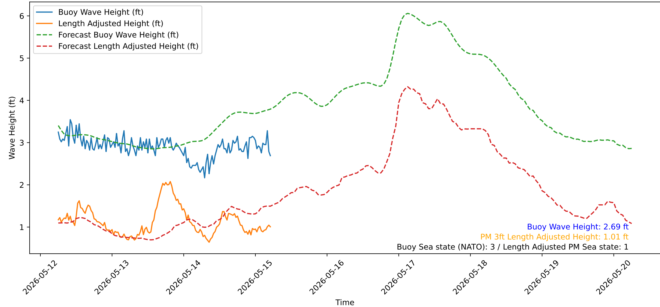
Wave Heights over Time for Oceanside Harbor at 2026-05-15 06:00:31
