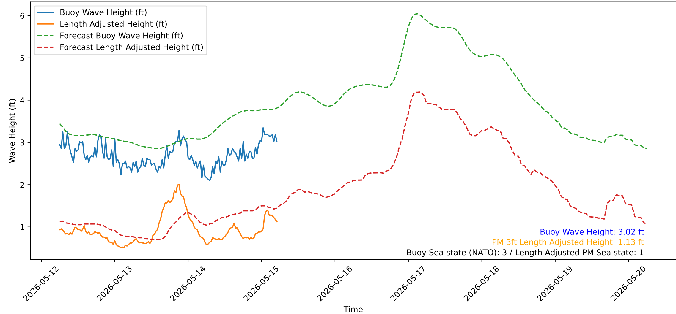
Wave Heights over Time for Green Beach at 2026-05-15 06:01:13
