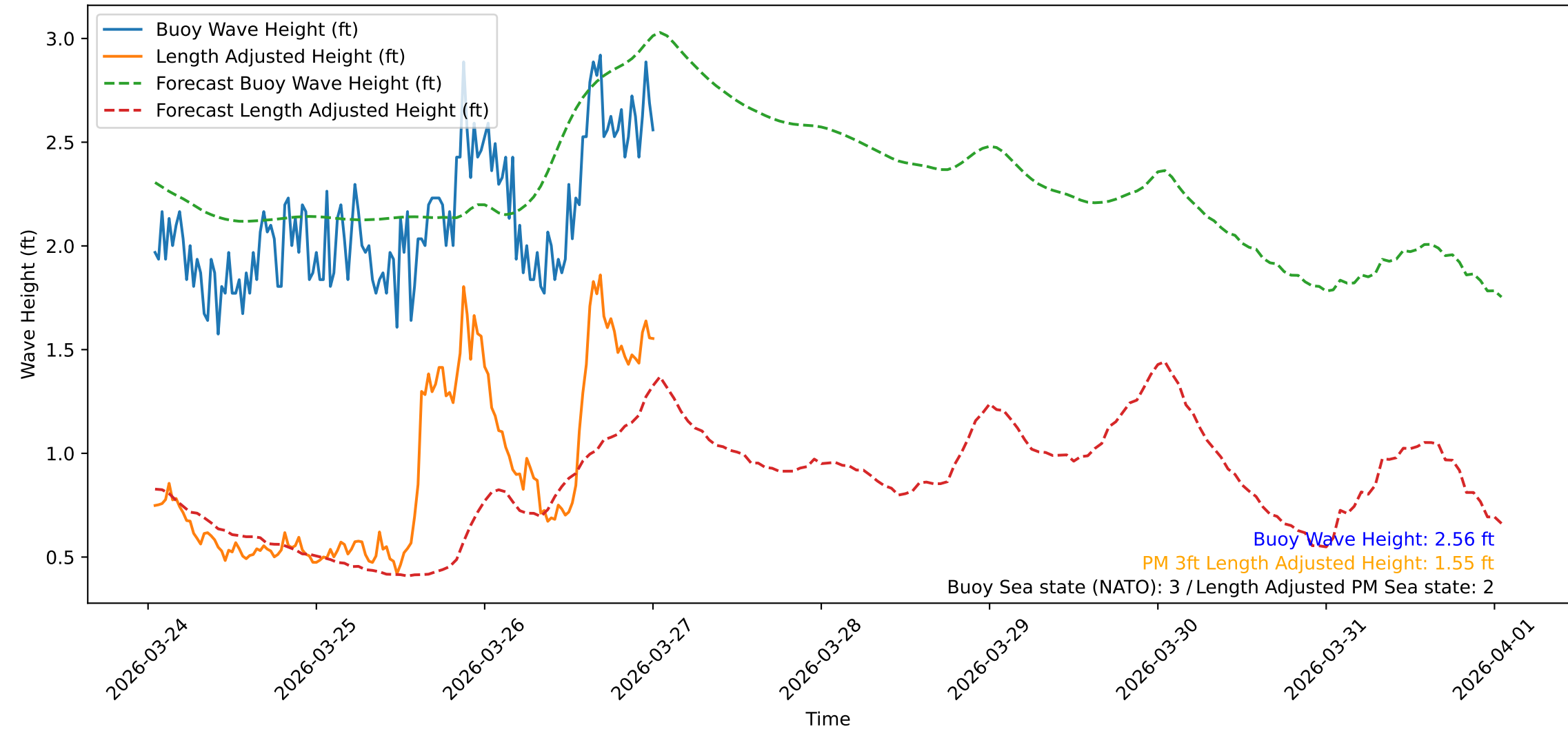
Wave Heights over Time for Oceanside Harbor at 2026-03-27 01:10:31
