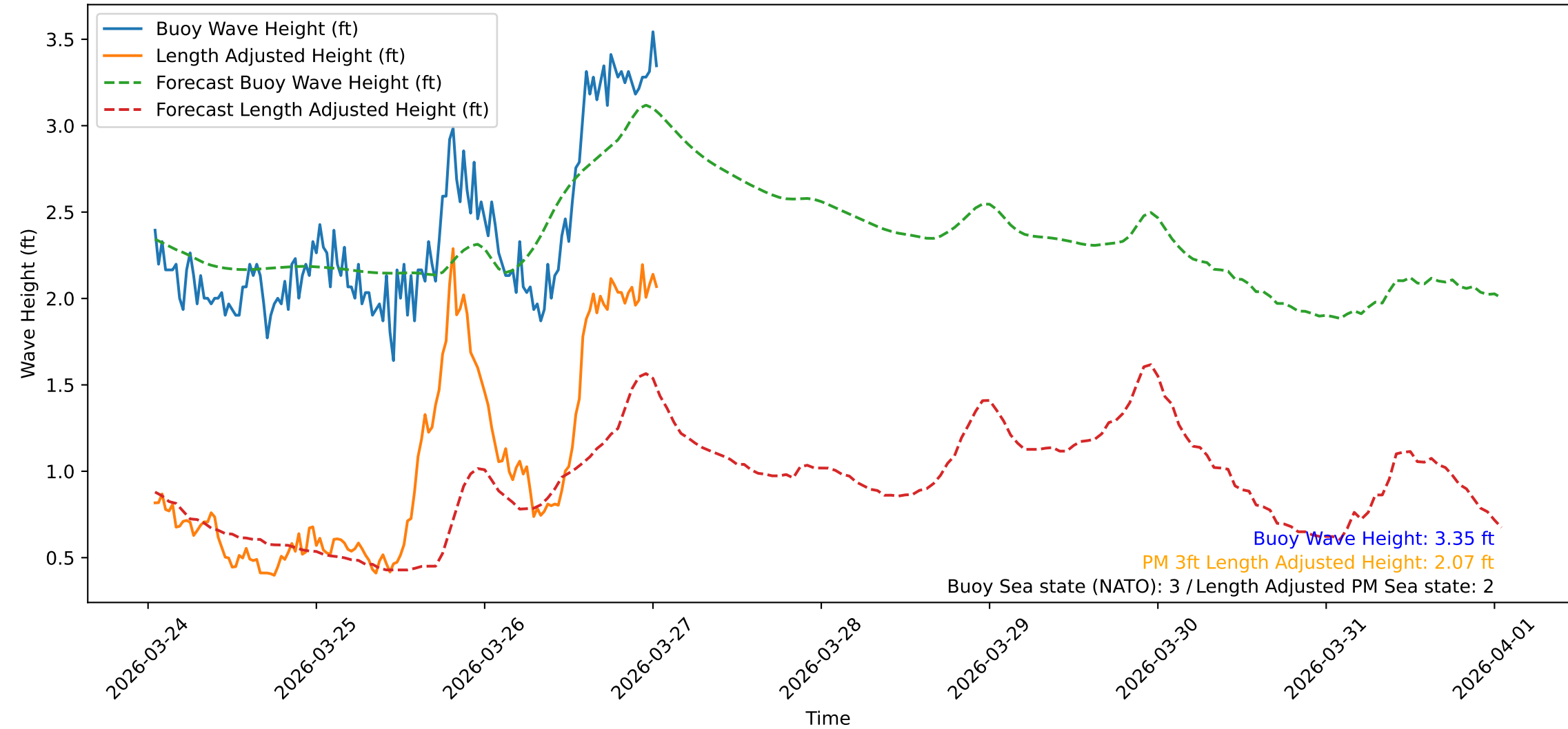
Wave Heights over Time for Green Beach at 2026-03-27 01:11:10
