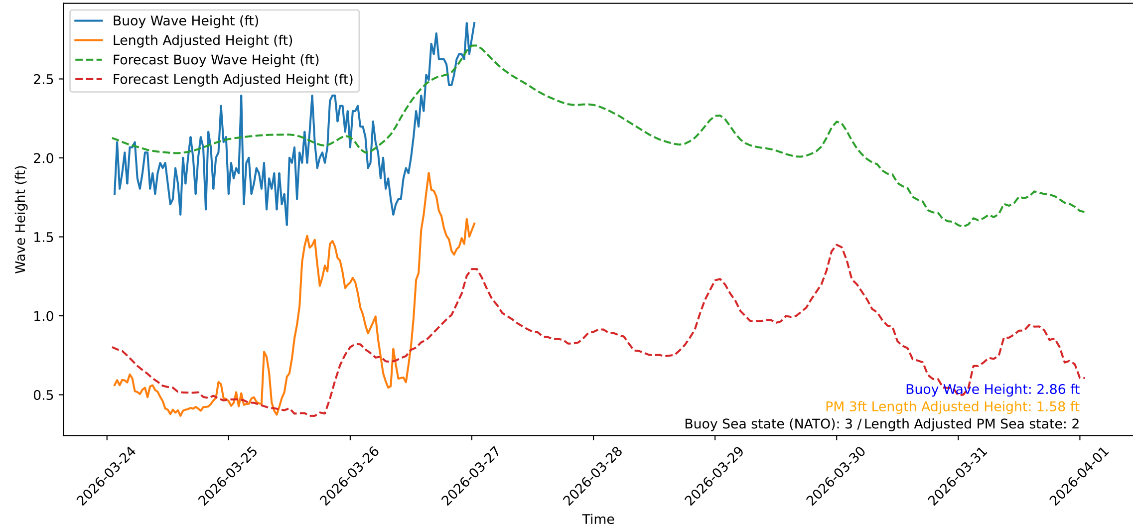
Wave Heights over Time for Red Beach at 2026-03-27 01:10:47
