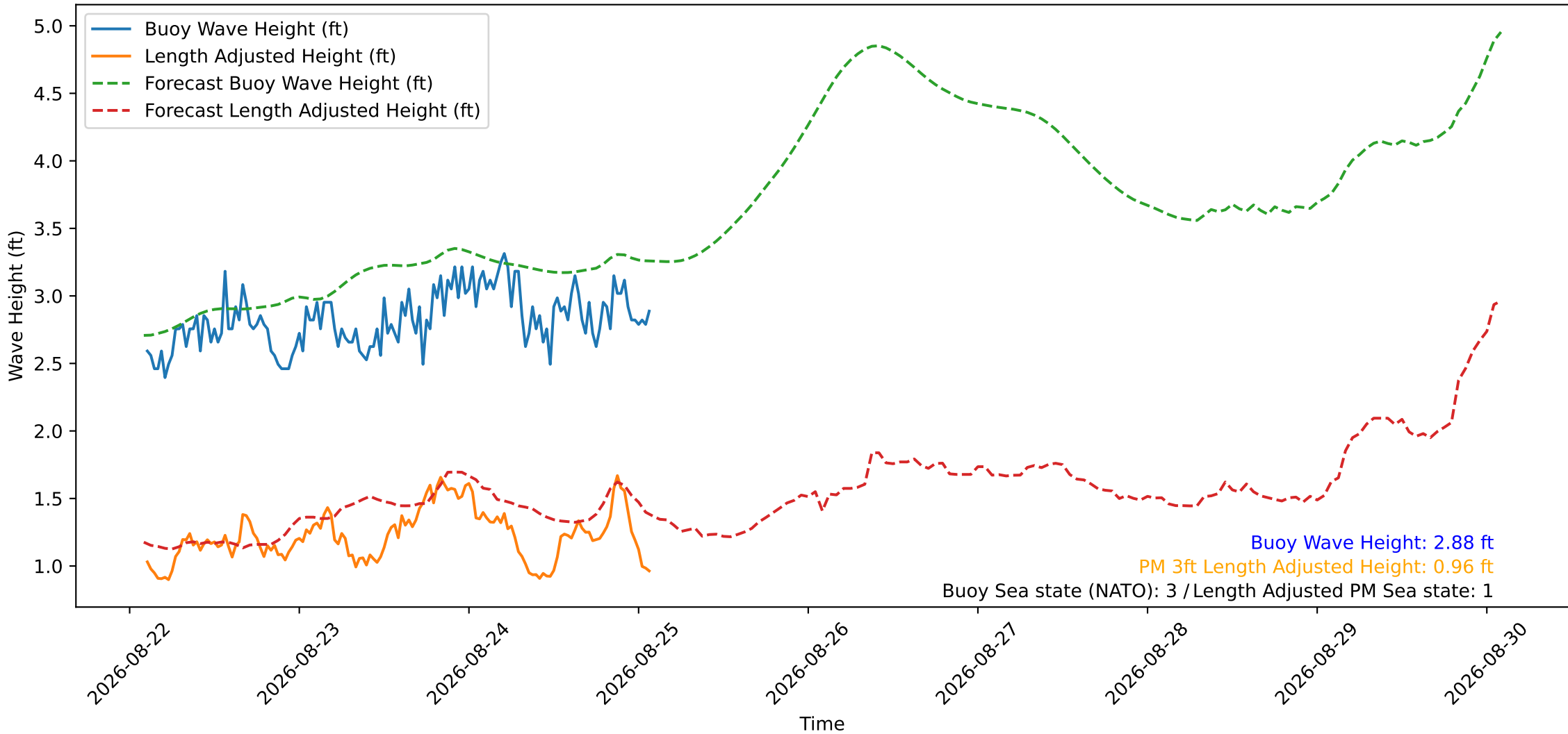
Wave Heights over Time for Green Beach at 2026-08-25 02:11:11
