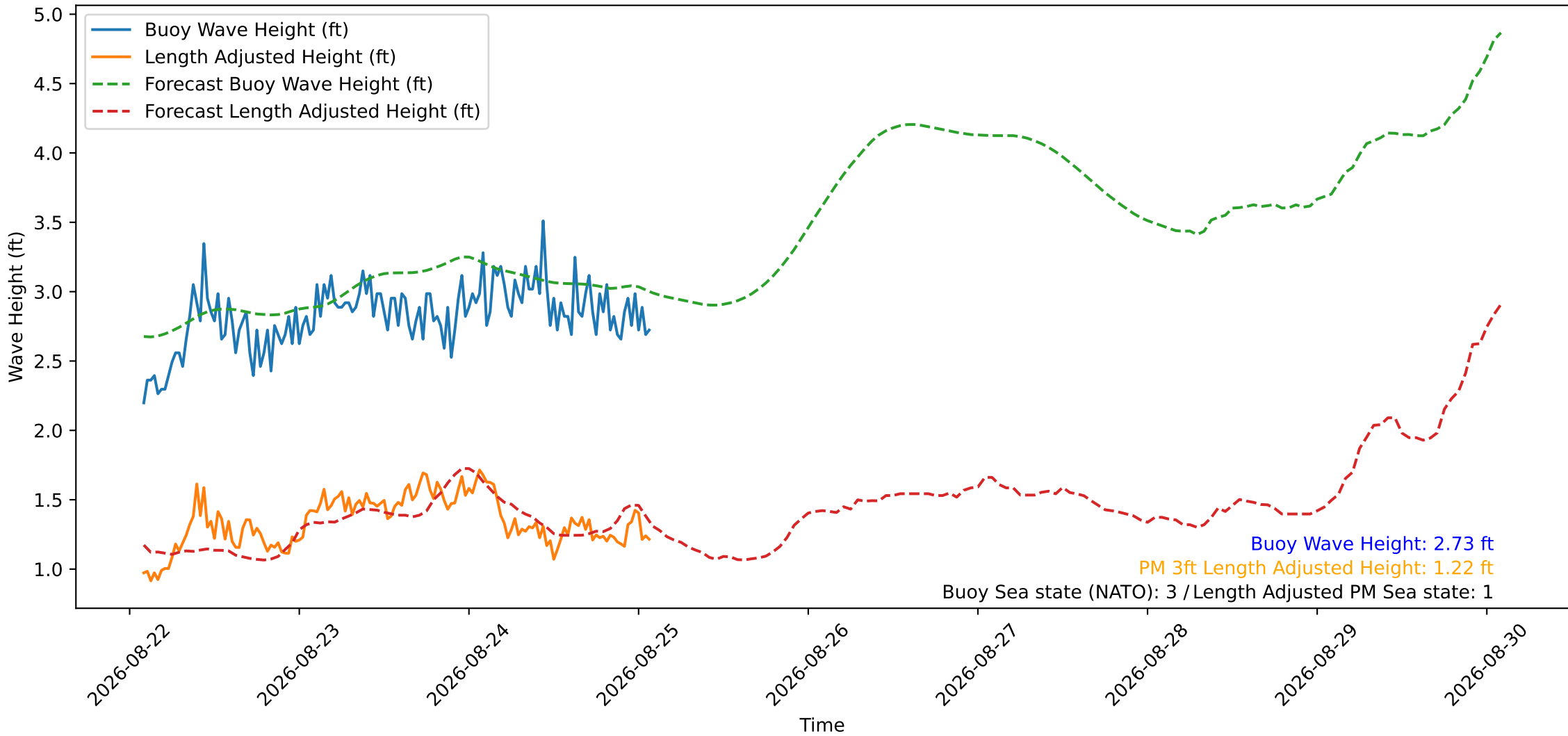
Wave Heights over Time for Oceanside Harbor at 2026-08-25 02:10:30
