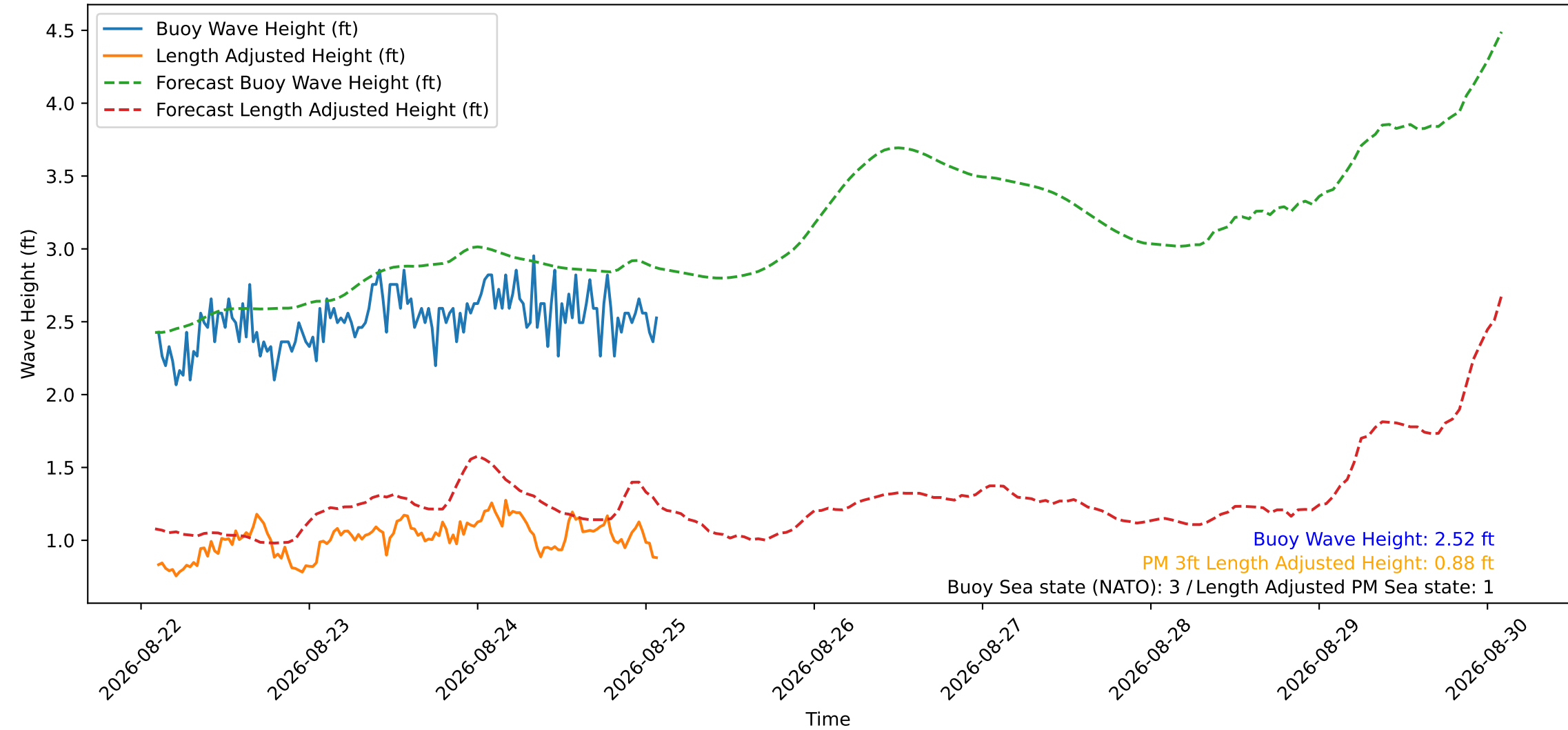
Wave Heights over Time for Red Beach at 2026-08-25 02:10:49
