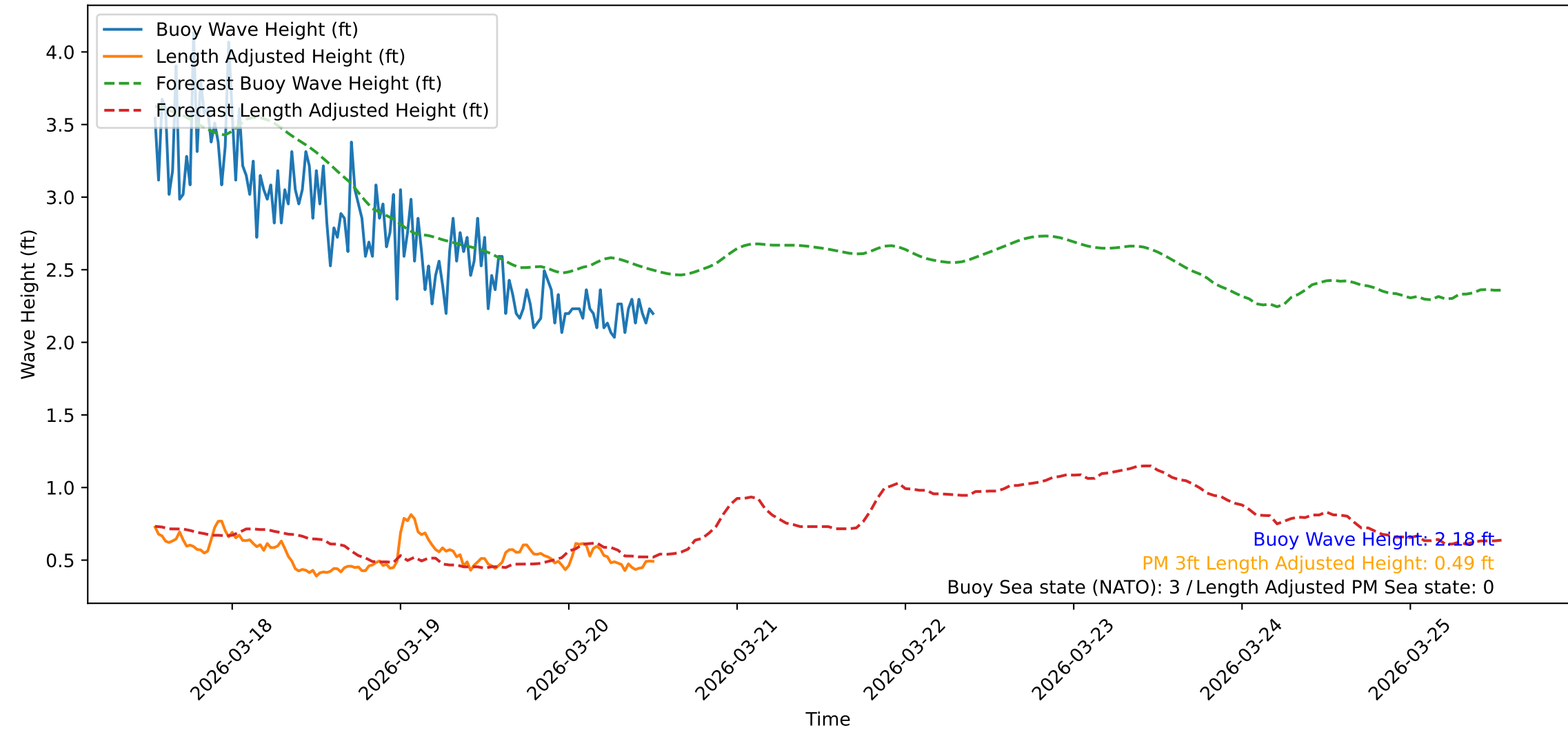
Wave Heights over Time for Green Beach at 2026-03-20 13:01:10
