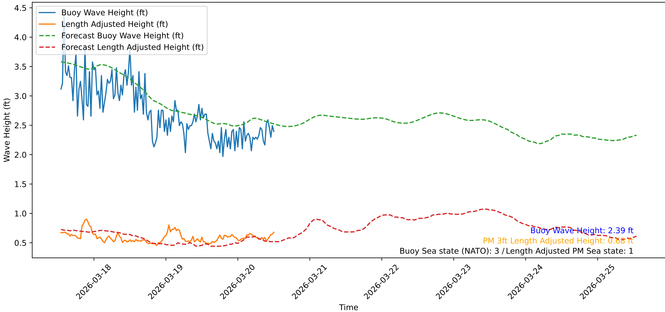
Wave Heights over Time for Oceanside Harbor at 2026-03-20 13:00:31
