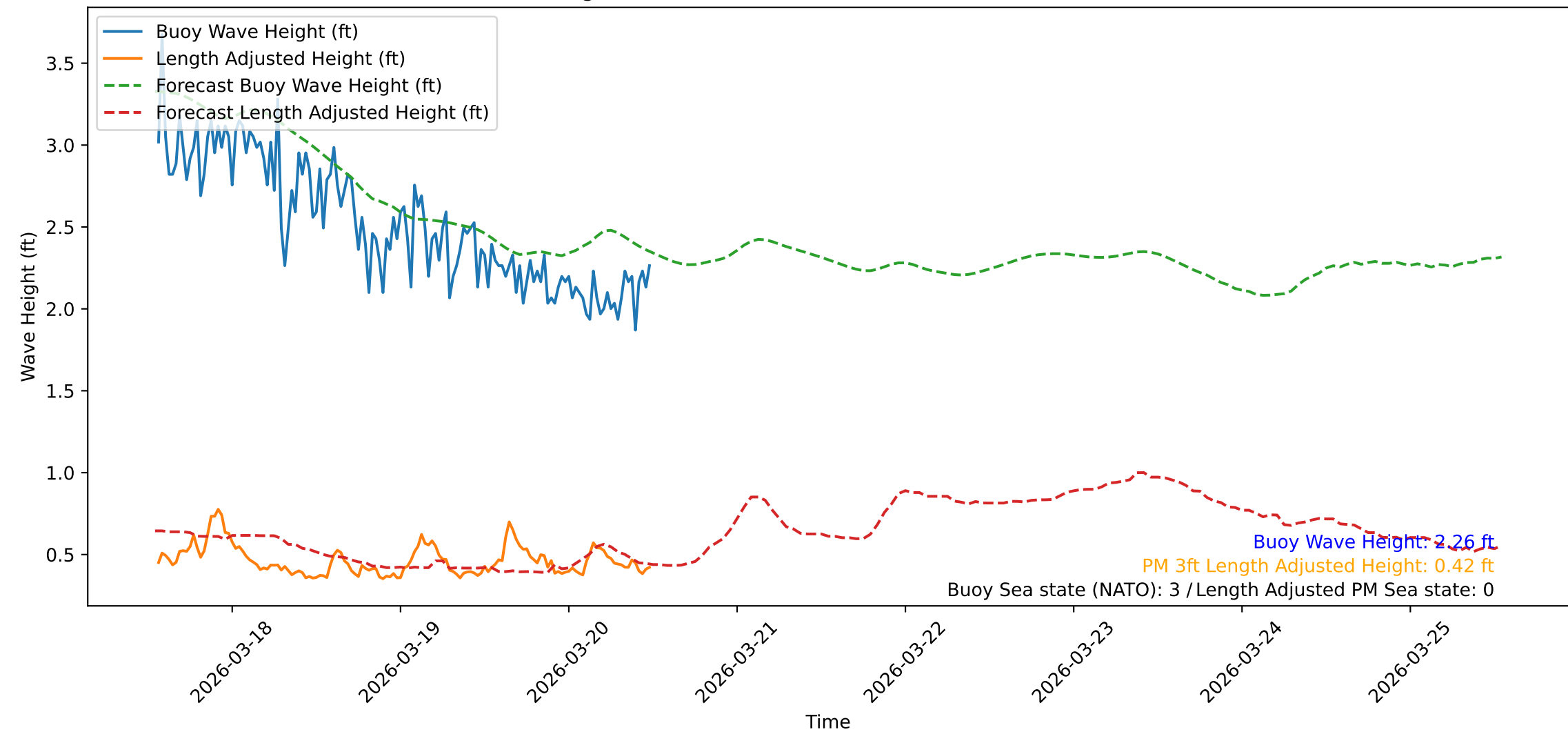
Wave Heights over Time for Red Beach at 2026-03-20 13:00:47
