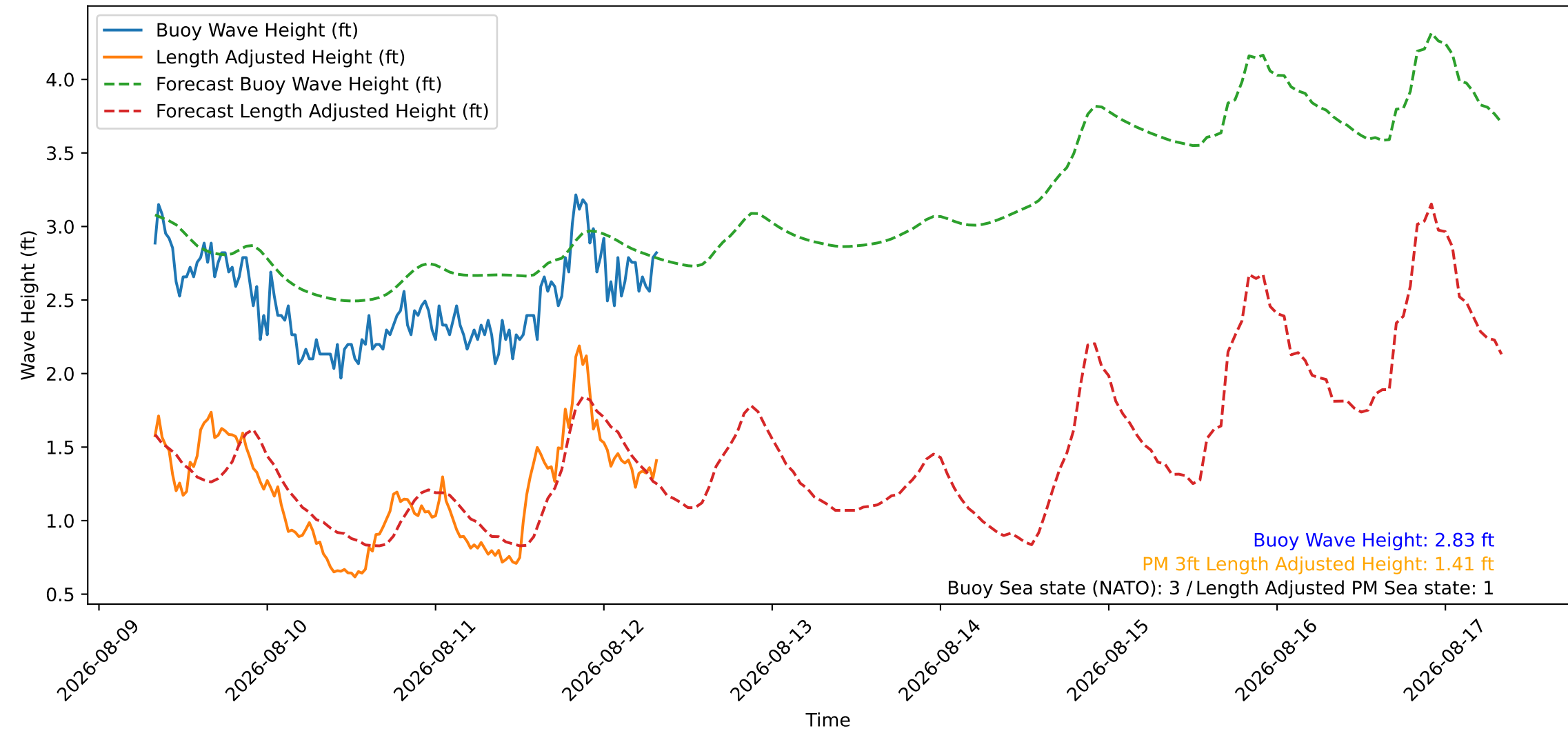
Wave Heights over Time for Green Beach at 2026-08-12 08:11:09
