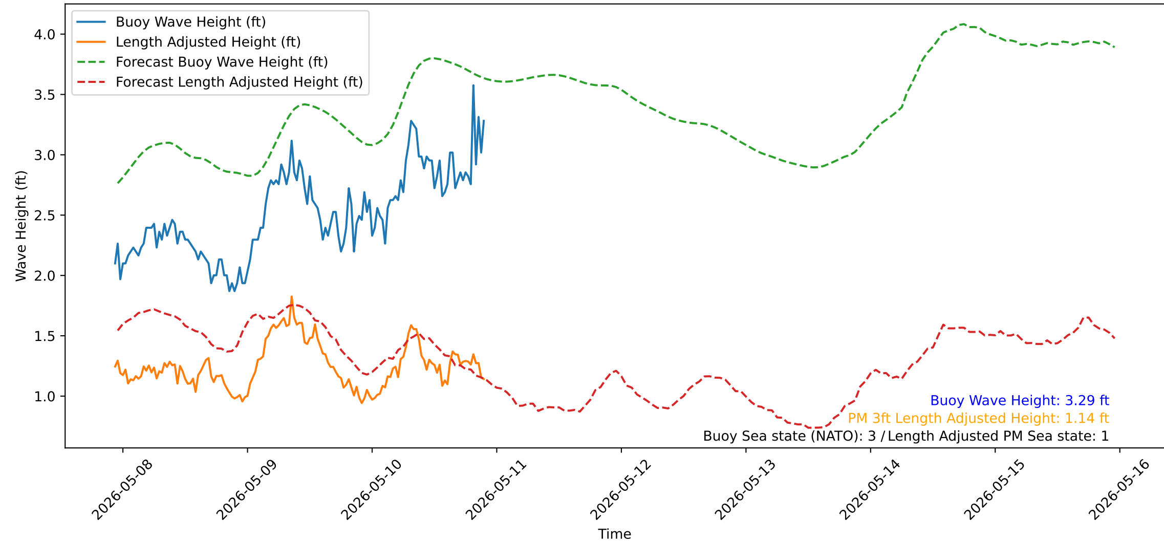
Wave Heights over Time for Oceanside Harbor at 2026-05-10 22:30:32
