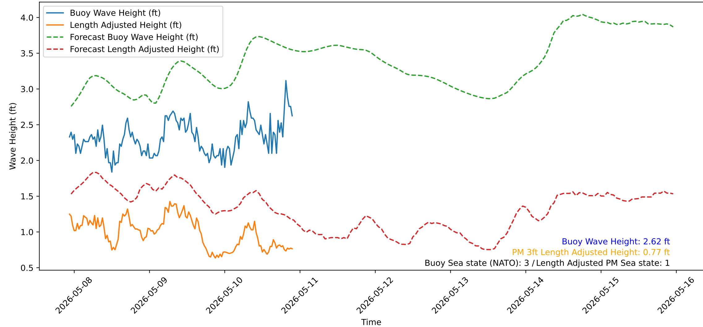
Wave Heights over Time for Green Beach at 2026-05-10 22:31:13
