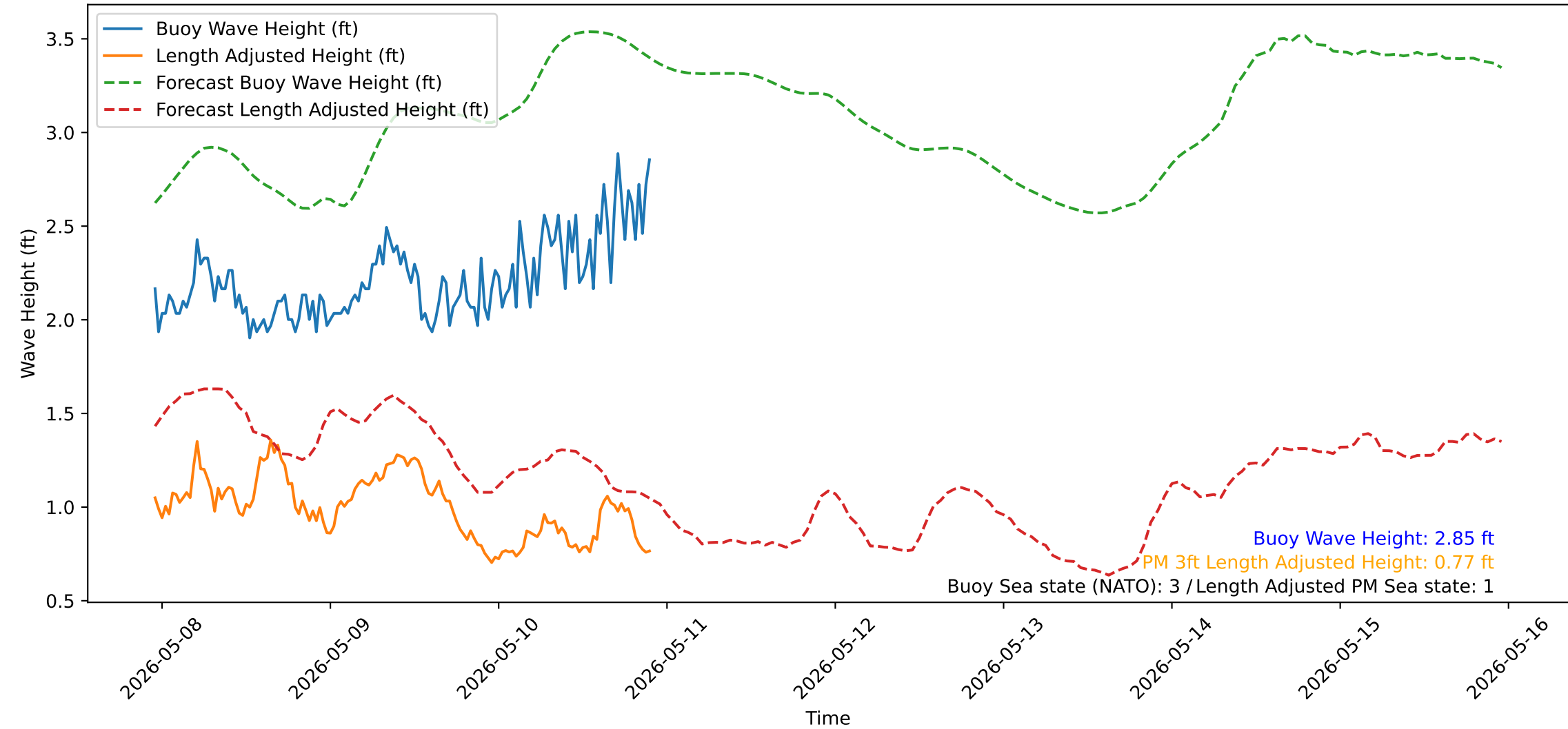
Wave Heights over Time for Red Beach at 2026-05-10 22:30:51
