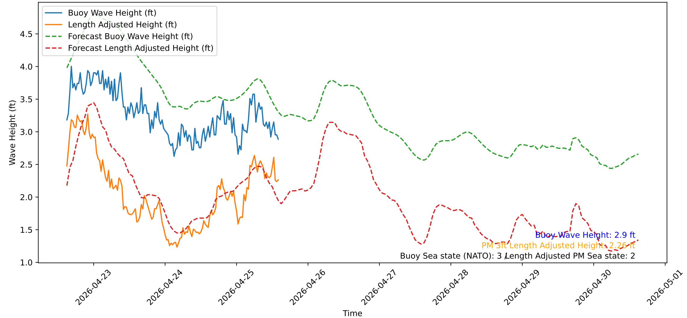
Wave Heights over Time for Green Beach at 2026-04-25 15:01:14
