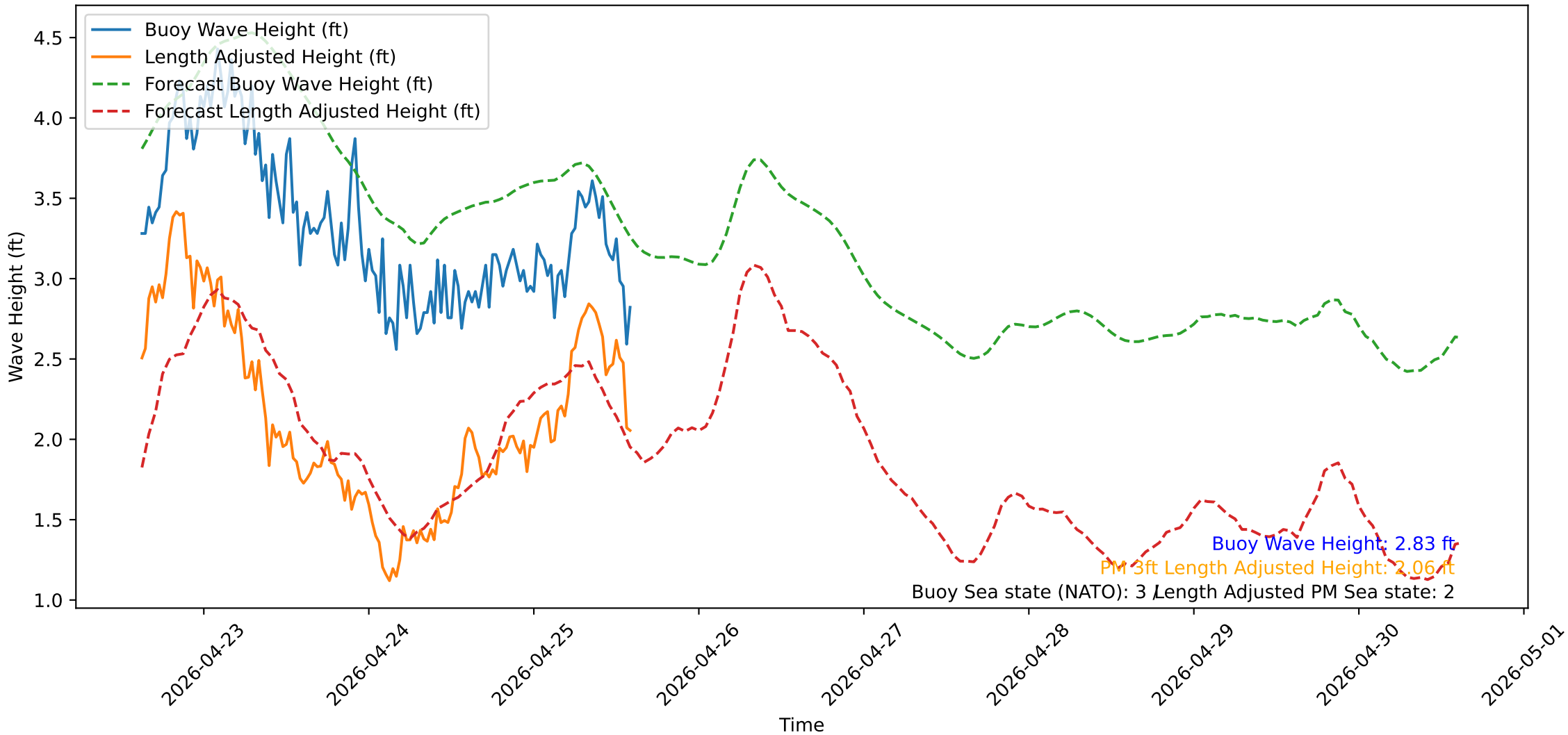
Wave Heights over Time for Oceanside Harbor at 2026-04-25 15:00:32
