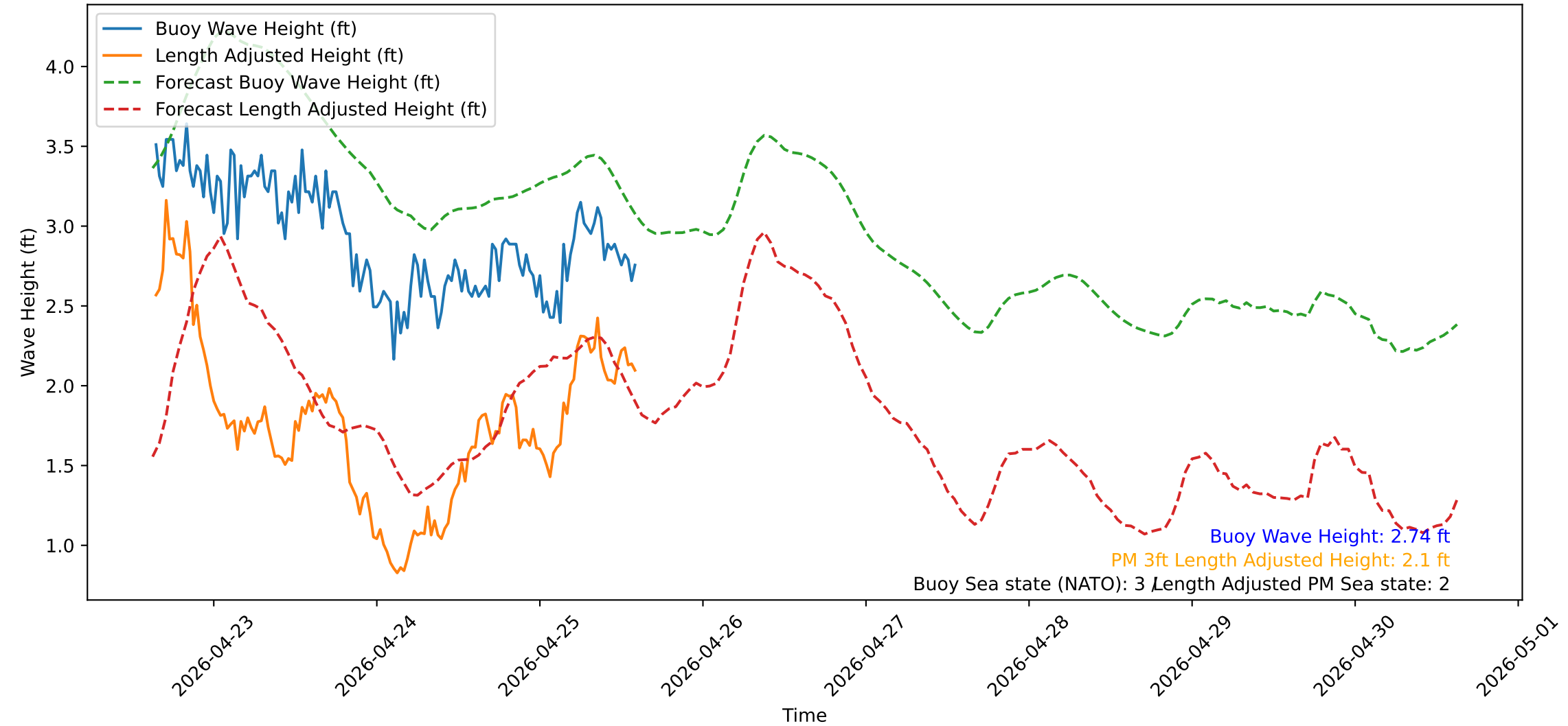
Wave Heights over Time for Red Beach at 2026-04-25 15:00:51
