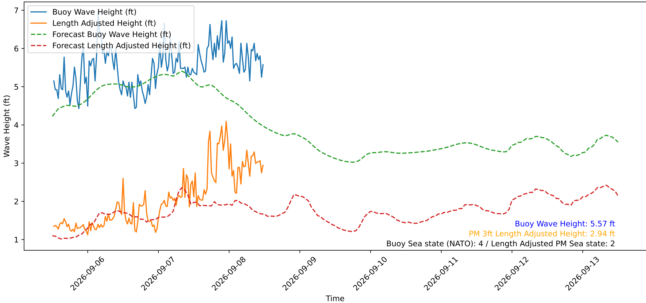
Wave Heights over Time for Red Beach at 2026-09-08 12:20:50
