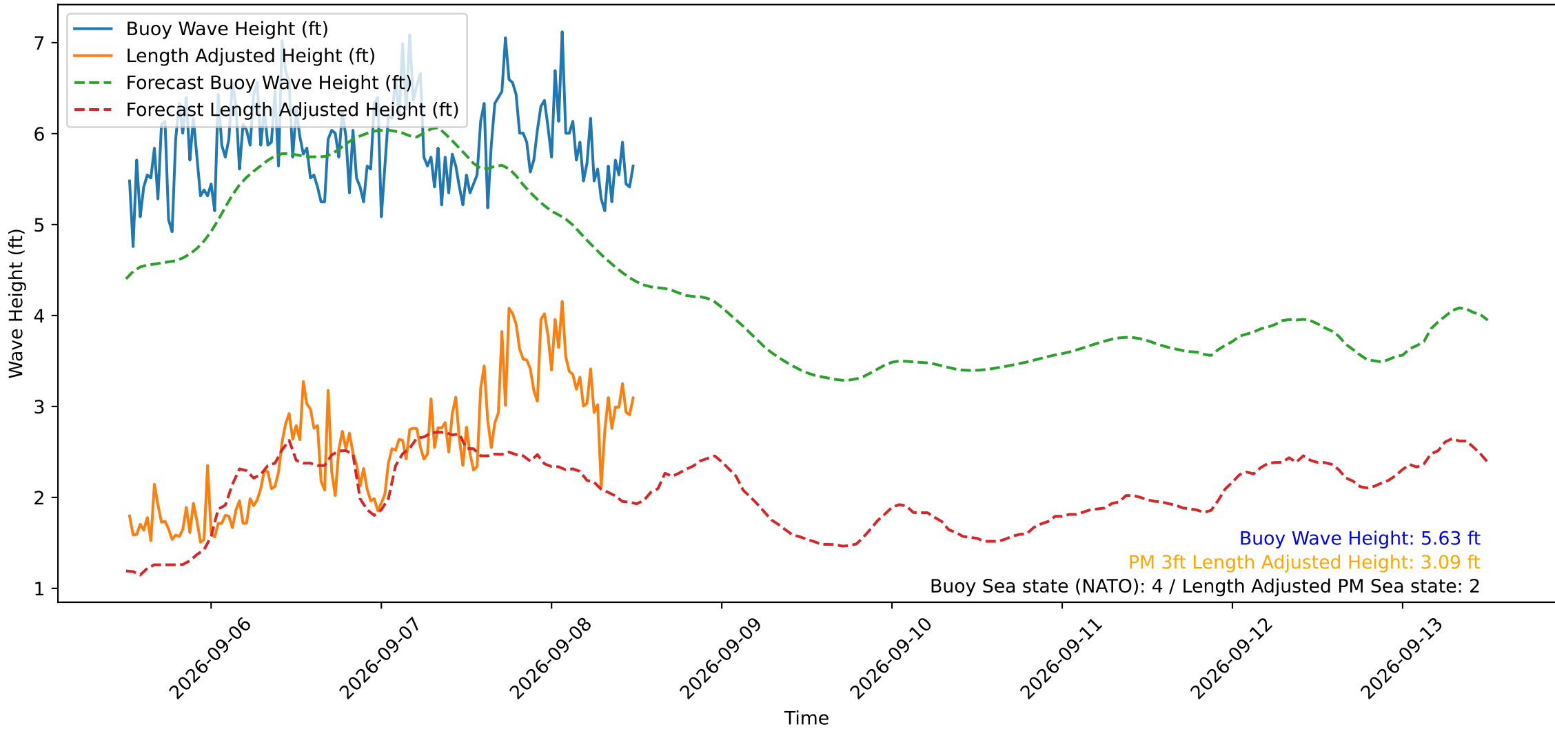
Wave Heights over Time for Oceanside Harbor at 2026-09-08 12:20:29
