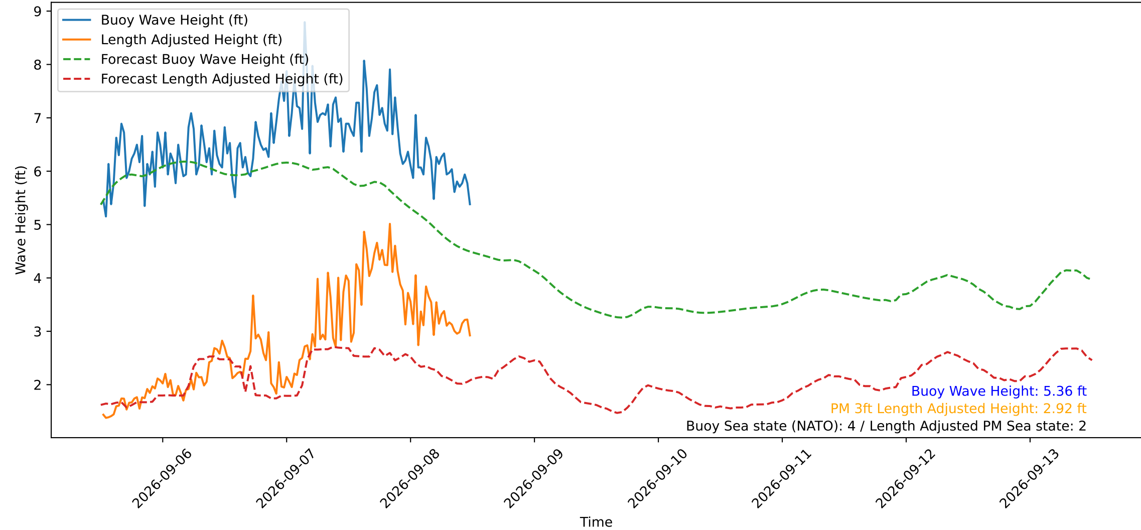
Wave Heights over Time for Green Beach at 2026-09-08 12:21:13
