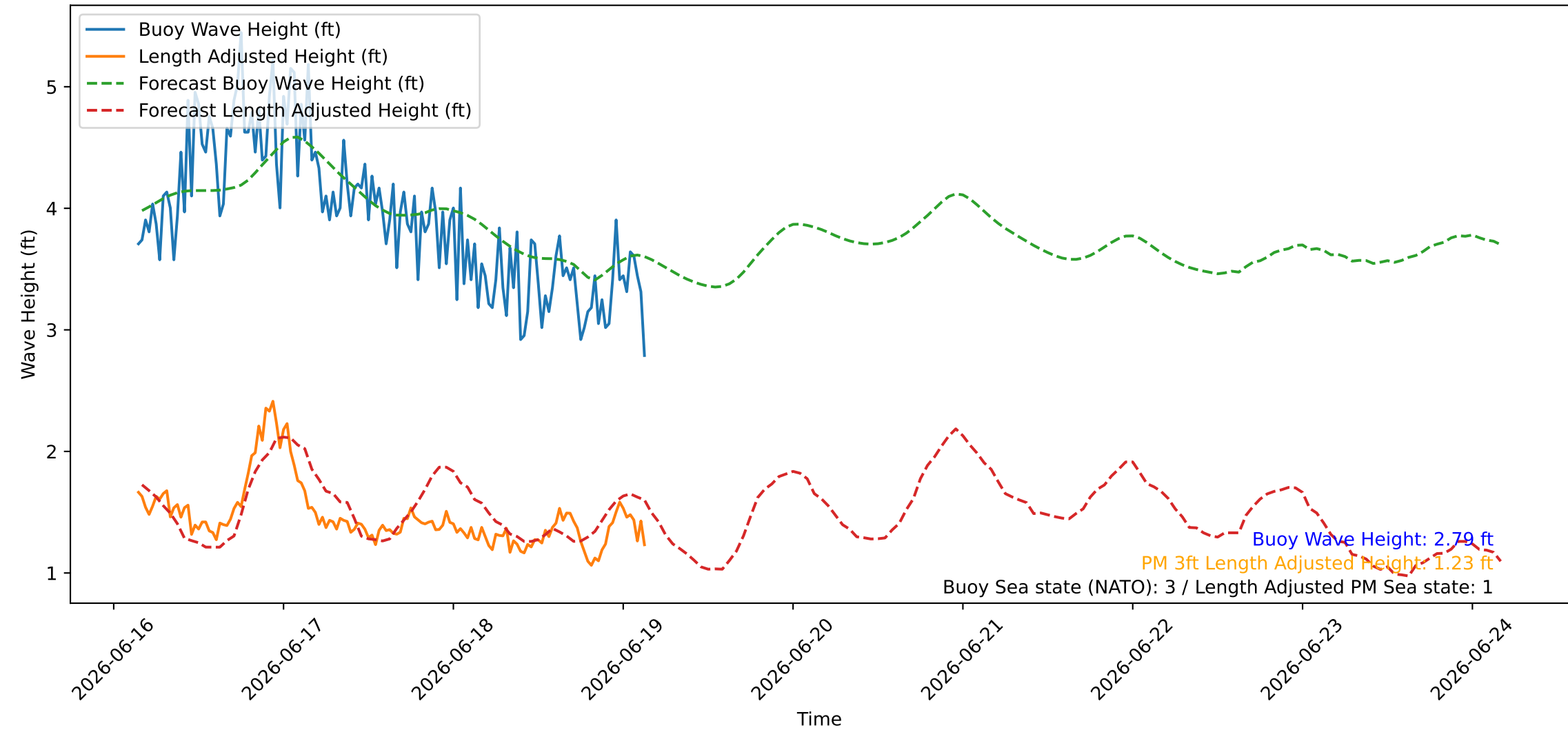
Wave Heights over Time for Oceanside Harbor at 2026-06-19 03:30:26
