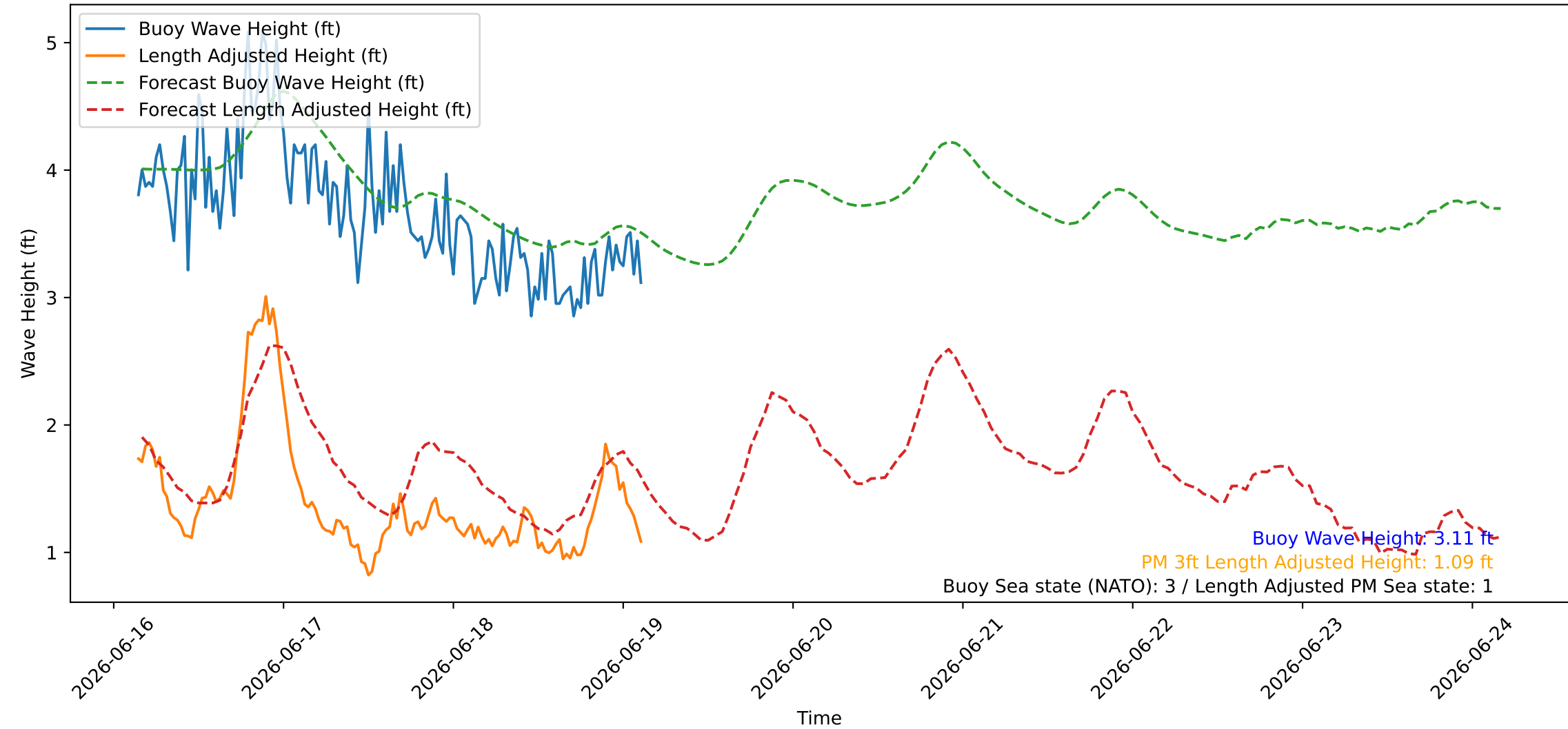
Wave Heights over Time for Green Beach at 2026-06-19 03:31:07
