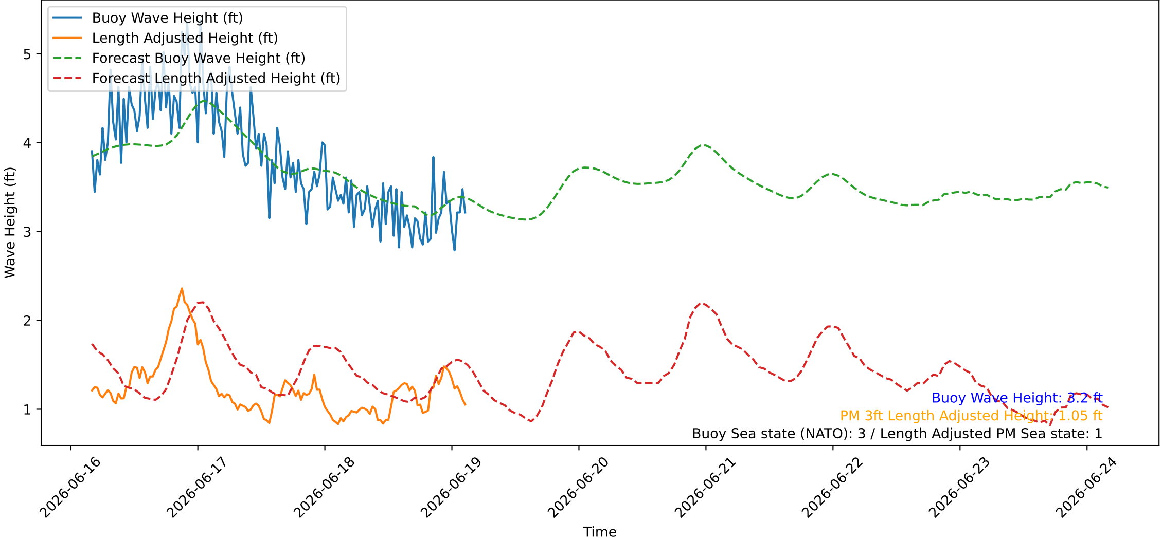
Wave Heights over Time for Red Beach at 2026-06-19 03:30:45
