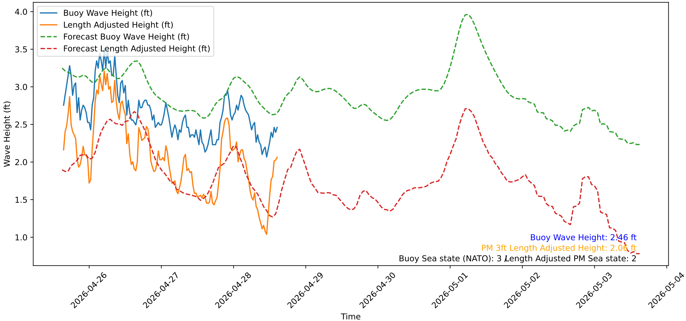
Wave Heights over Time for Green Beach at 2026-04-28 15:21:14
