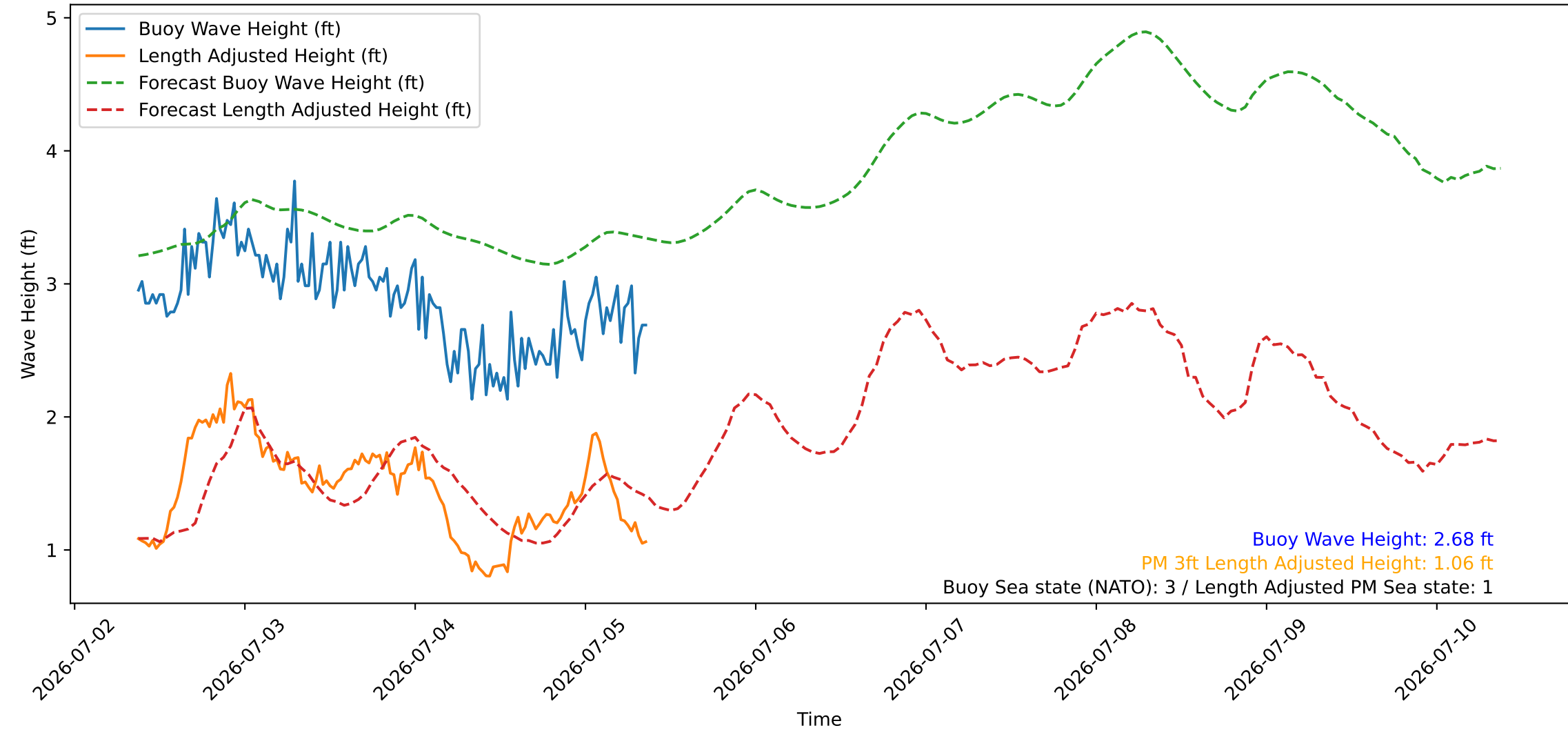
Wave Heights over Time for Oceanside Harbor at 2026-07-05 09:10:26
