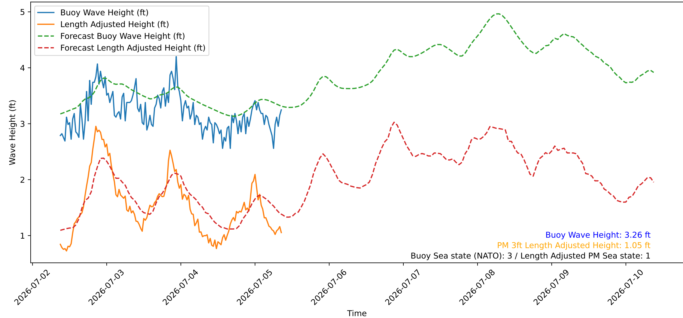
Wave Heights over Time for Green Beach at 2026-07-05 09:11:08
