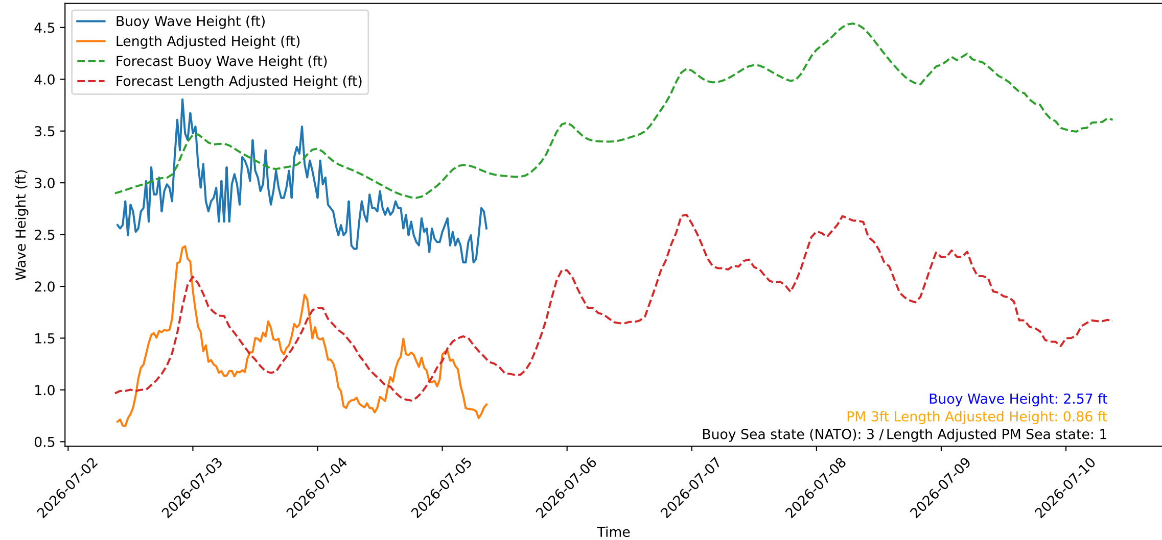
Wave Heights over Time for Red Beach at 2026-07-05 09:10:45
